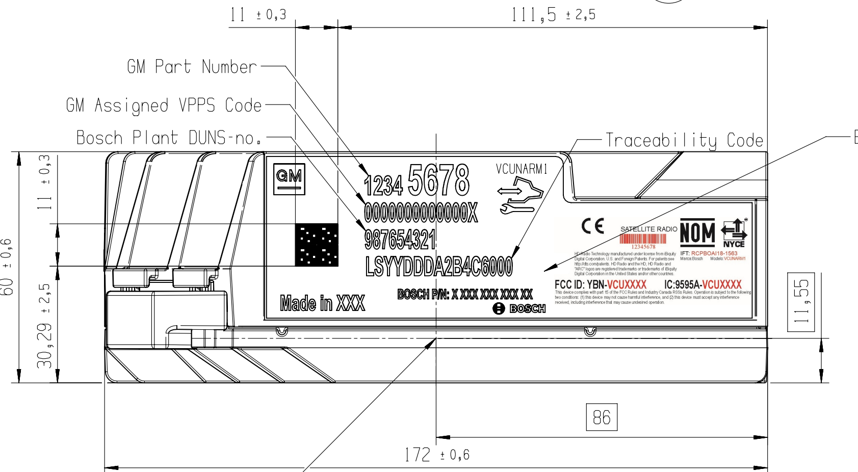
VIEW A
