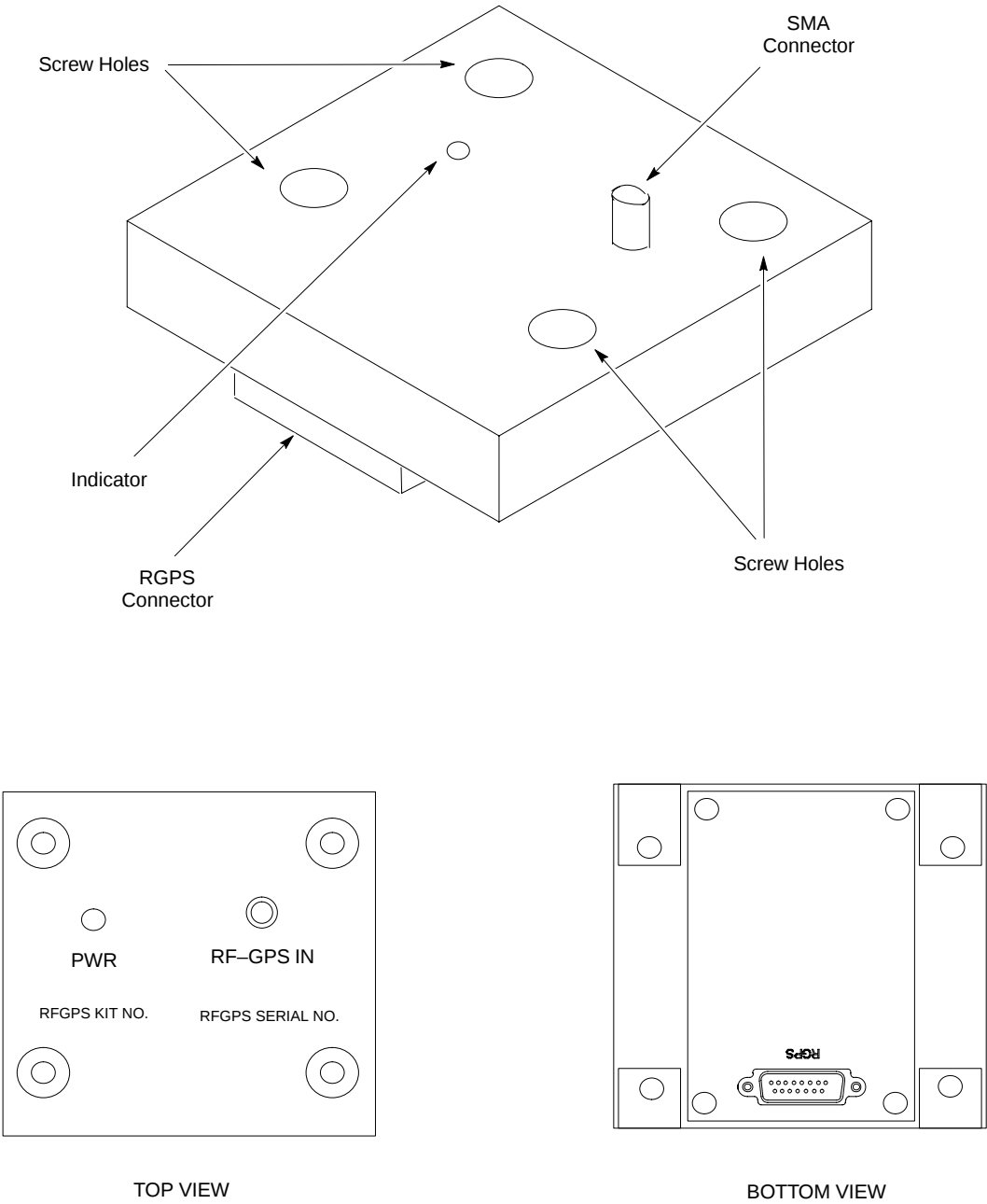
Figure 9-7: RF-GPS Module
