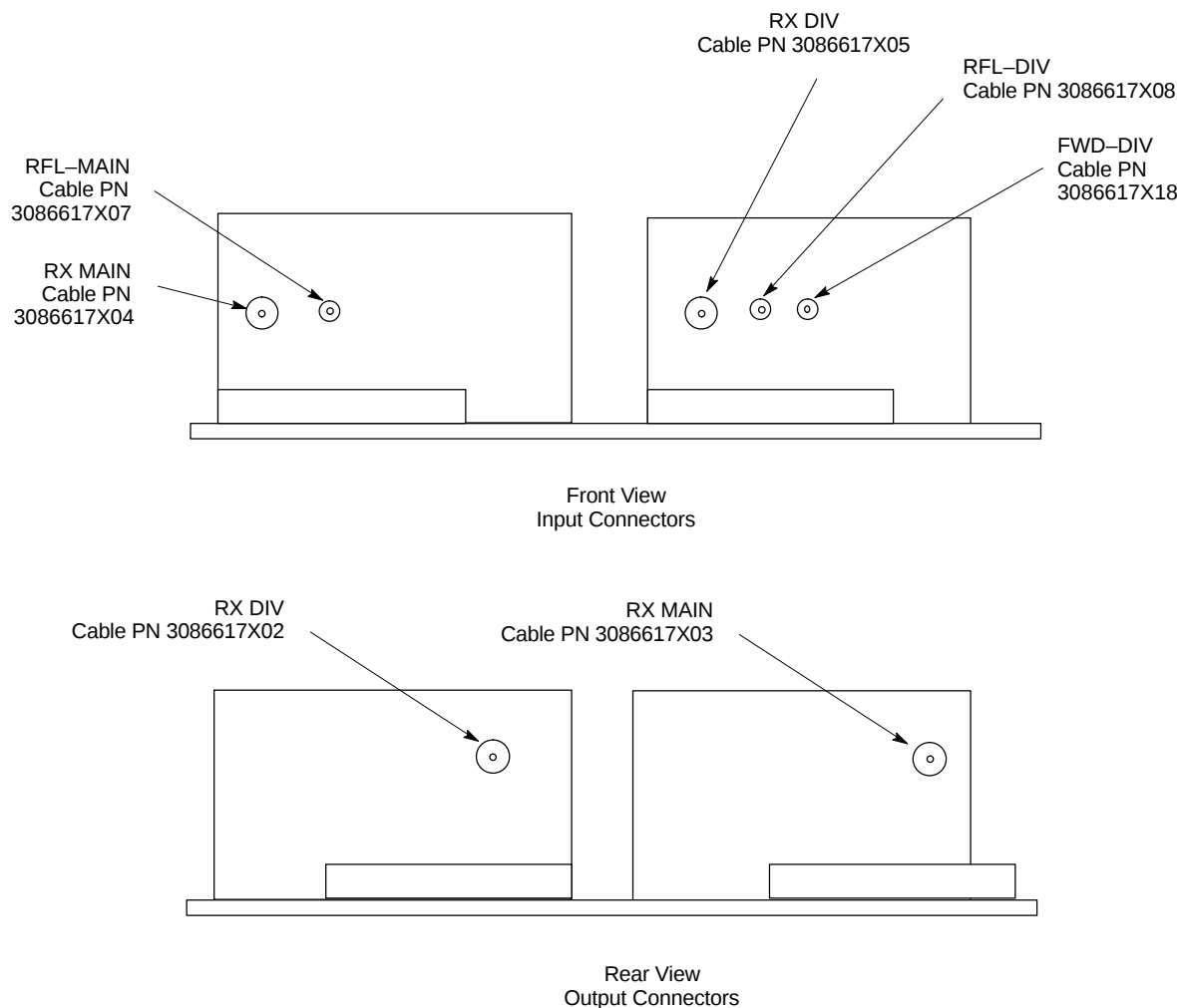
Figure 9-22: Filter Tray Connectors and Cable Part Numbers
