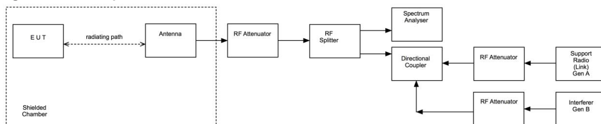
Figure i Test Setup
