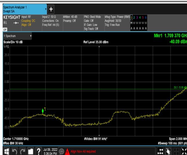
Band66-1.4MHz-QPSK-131979-6RB#0
