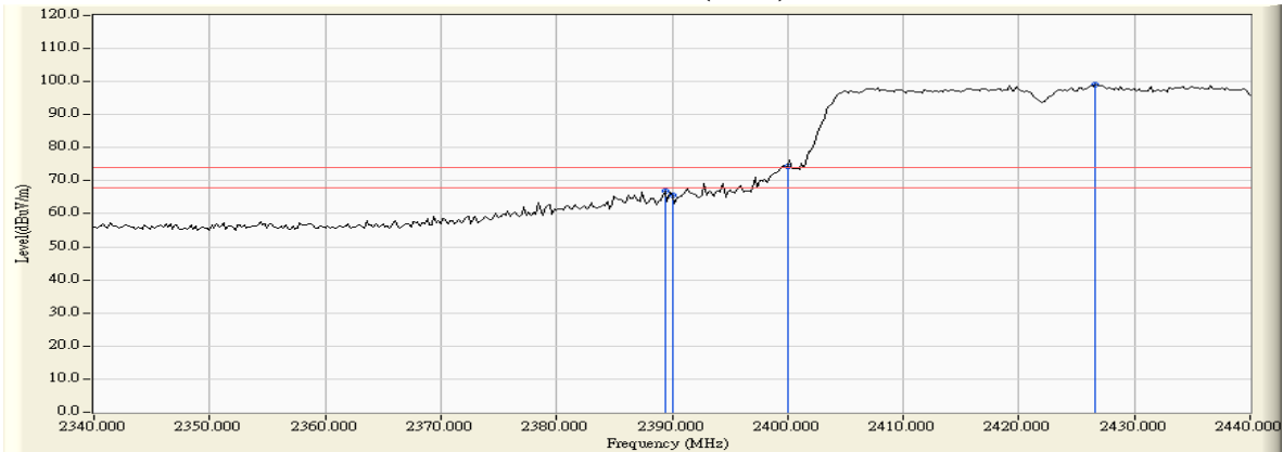
Figure Channel 03:
