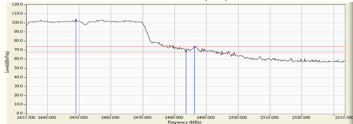
Figure Channel 09:
