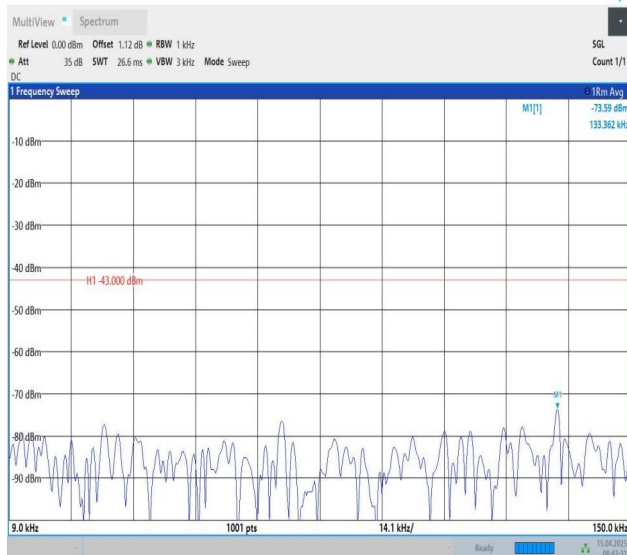
Band25-5MHz-QPSK-26365-1RB#0-0.009~0.15-PASS
