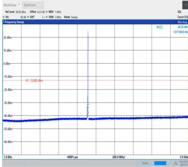
Band25-5MHz-QPSK-26665-1RB#24-1000~3000-PASS
