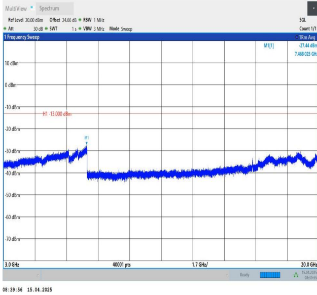
Band25-3MHz-QPSK-26365-1RB#0-3000~20000-PASS
