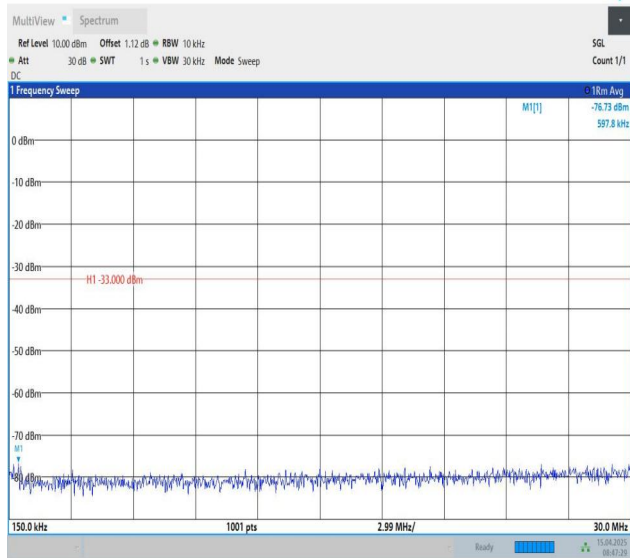
Band25-10MHz-QPSK-26090-1RB#49-0.15~30-PASS
