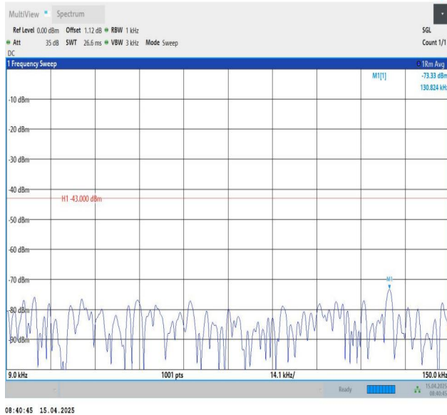
Band25-3MHz-QPSK-26675-1RB#0-0.009~0.15-PASS
