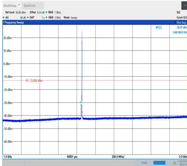
Band25-5MHz-QPSK-26065-1RB#24-1000~3000-PASS
