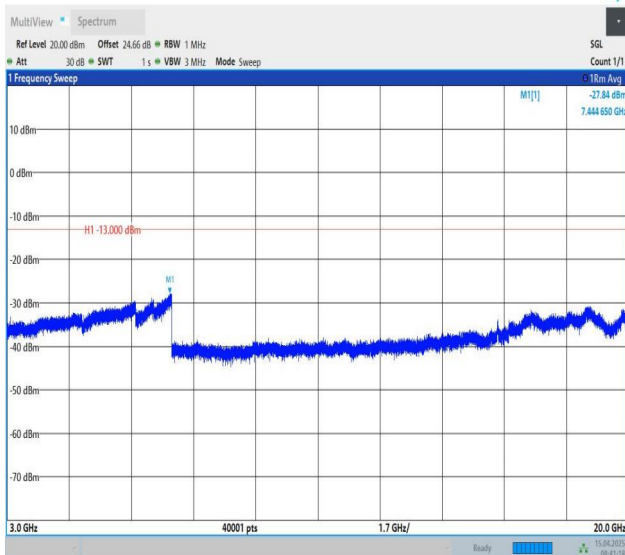
Band25-3MHz-QPSK-26675-1RB#0-3000~20000-PASS
