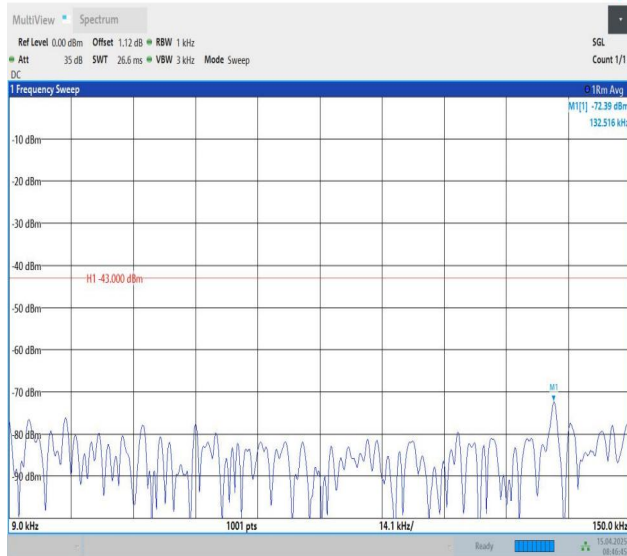
Band25-10MHz-QPSK-26090-1RB#0-0.009~0.15-PASS
