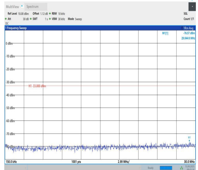
Band25-5MHz-QPSK-26365-1RB#0-0.15~30-PASS
