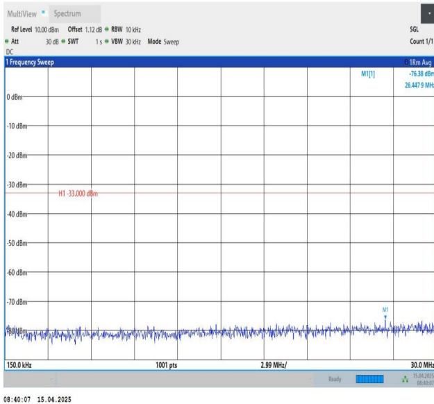
Band25-3MHz-QPSK-26365-1RB#14-0.15~30-PASS
