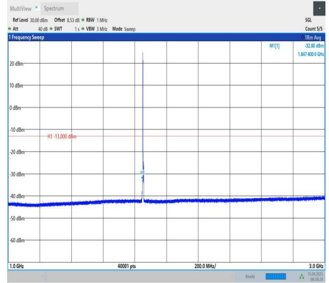
Band25-3MHz-QPSK-26055-1RB#0-1000~3000-PASS
