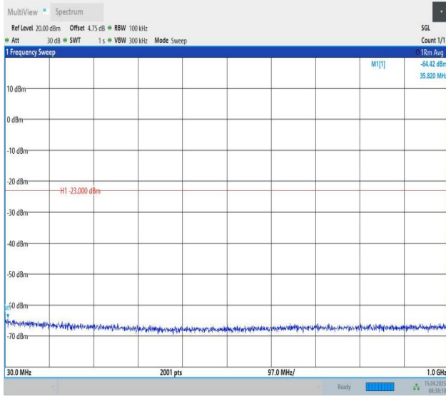
Band25-3MHz-QPSK-26055-1RB#0-30~1000-PASS
