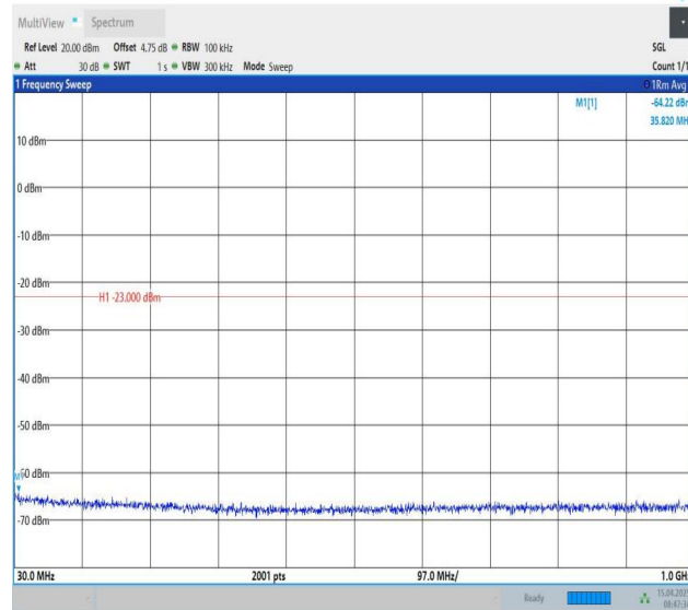
Band25-10MHz-QPSK-26090-1RB#49-30~1000-PASS
