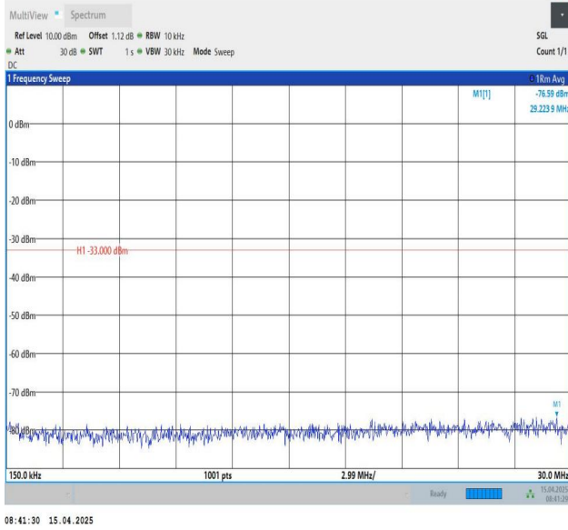
Band25-3MHz-QPSK-26675-1RB#14-0.15~30-PASS
