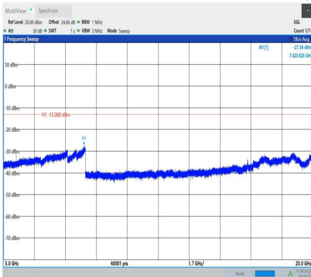
Band25-3MHz-QPSK-26055-1RB#0-3000~20000-PASS
