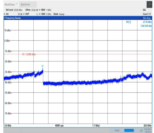
Band25-5MHz-QPSK-26065-1RB#24-3000~20000-PASS
