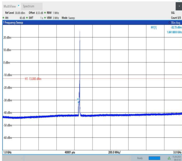
Band25-10MHz-QPSK-26090-1RB#49-1000~3000-PASS
