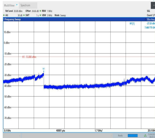
Band25-10MHz-QPSK-26090-1RB#49-3000~20000-PASS
