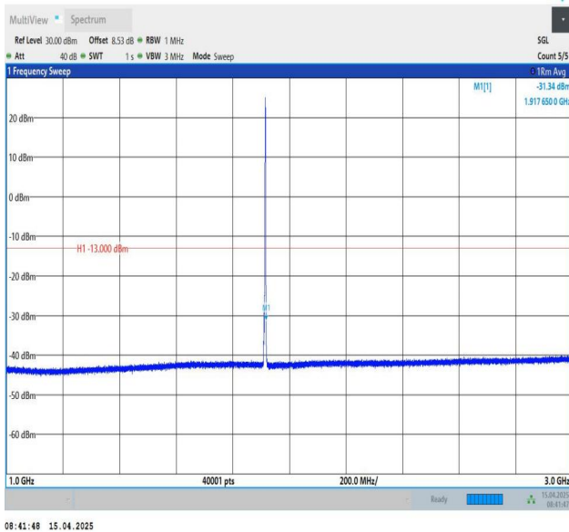
Band25-3MHz-QPSK-26675-1RB#14-1000~3000-PASS
