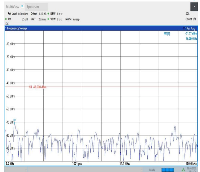
Band25-3MHz-QPSK-26675-1RB#14-0.009~0.15-PASS
