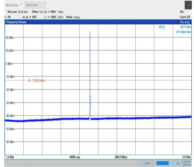
Band25-3MHz-QPSK-26675-1RB#0-1000~3000-PASS
