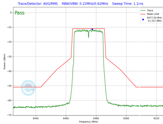
Plot 7-808. LPI In-Band Emission Plot Antenna WF8 (20MHz 802.11ax (UNII Band 6) – Ch. 105, MCS4)
