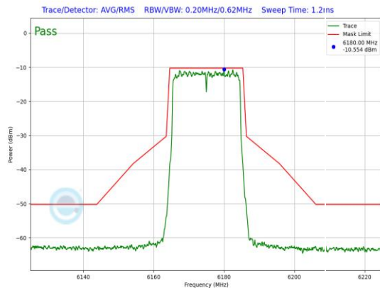
Plot 7-893. LPI In-Band Emission Plot Antenna WF7 (20MHz 802.11ax (UNII Band 5) – Ch. 45, MCS4)
