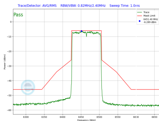
Plot 7-900. LPI In-Band Emission Plot Antenna WF7 (80MHz 802.11ax (UNII Band 6) – Ch. 103, MCS4)
