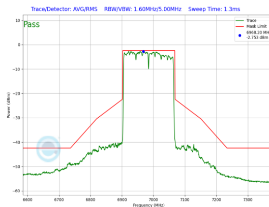
Plot 7-841. LPI In-Band Emission Plot Antenna WF8 (160MHz 802.11ax (UNII Band 8) – Ch. 207, MCS11)
