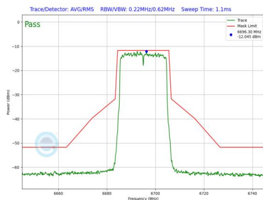
Plot 7-903. LPI In-Band Emission Plot Antenna WF7 (20MHz 802.11ax (UNII Band 7) – Ch. 149, MCS4)
