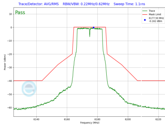
Plot 7-842. SP In-Band Emission Plot Antenna WF8 (20MHz 802.11a (UNII Band 5) – Ch. 45, 12Mbps)
