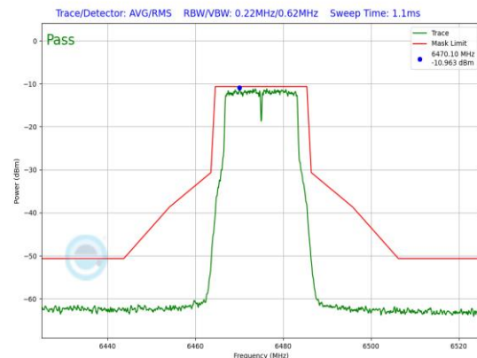
Plot 7-897. LPI In-Band Emission Plot Antenna WF7 (20MHz 802.11a (UNII Band 6) – Ch. 105, 24Mbps)
