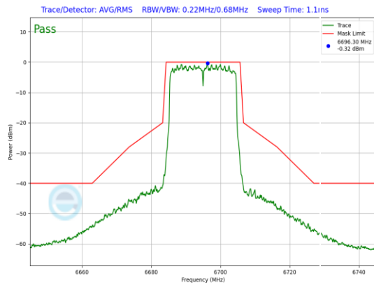
Plot 7-868. SP In-Band Emission Plot Antenna WF8 (20MHz 802.11ax (UNII Band 7) – Ch. 149, MCS11)
