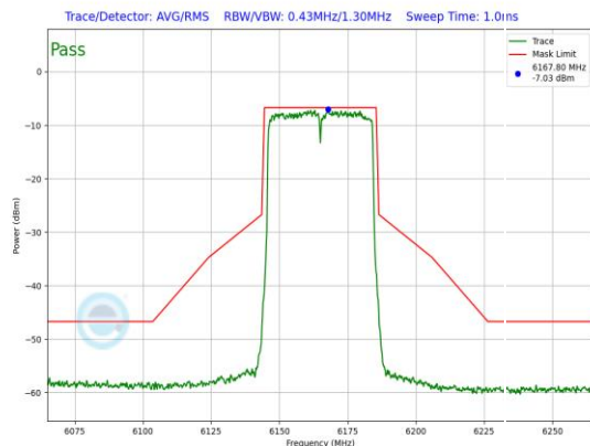
Plot 7-894. LPI In-Band Emission Plot Antenna WF7 (40MHz 802.11ax (UNII Band 5) – Ch. 43, MCS4)
