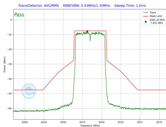
Plot 7-829. LPI In-Band Emission Plot Antenna WF8 (40MHz 802.11ax (UNII Band 6) – Ch. 107, MCS11)
