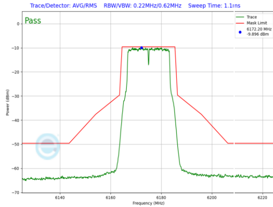
Plot 7-802. LPI In-Band Emission Plot Antenna WF8 (20MHz 802.11a (UNII Band 5) – Ch. 45, 24Mbps)
