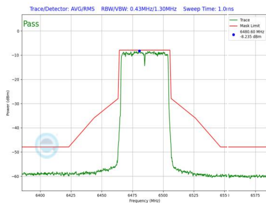
Plot 7-899. LPI In-Band Emission Plot Antenna WF7 (40MHz 802.11ax (UNII Band 6) – Ch. 107, MCS4)
