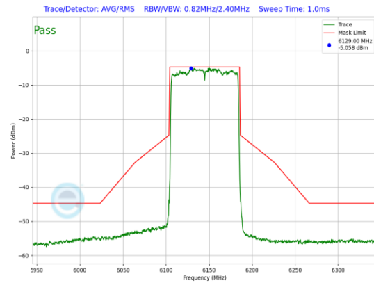
Plot 7-895. LPI In-Band Emission Plot Antenna WF7 (80MHz 802.11ax (UNII Band 5) – Ch. 39, MCS4)
