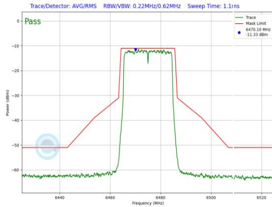
Plot 7-878. LPI In-Band Emission Plot Antenna WF7 (20MHz 802.11ax (UNII Band 6) – Ch. 105, MCS2)
