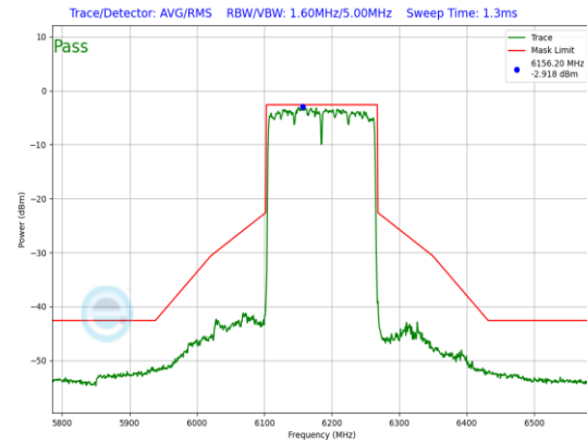
Plot 7-916. LPI In-Band Emission Plot Antenna WF7 (160MHz 802.11ax (UNII Band 5) – Ch. 47, MCS11)
