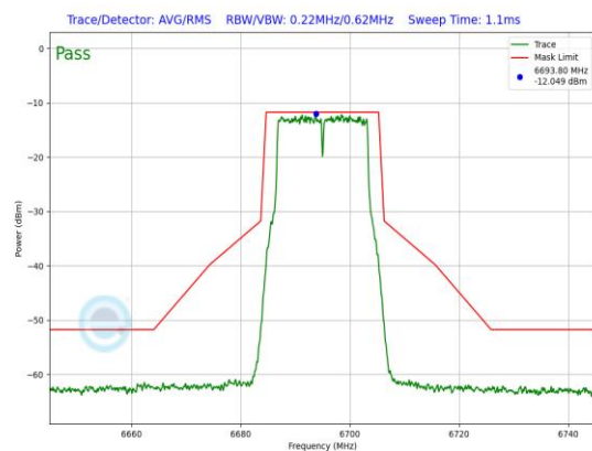
Plot 7-902. LPI In-Band Emission Plot Antenna WF7 (20MHz 802.11a (UNII Band 7) – Ch. 149, 24Mbps)
