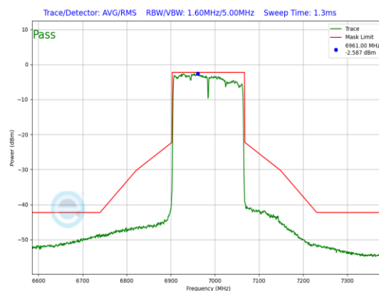
Plot 7-891. LPI In-Band Emission Plot Antenna WF7 (160MHz 802.11ax (UNII Band 8) – Ch. 207, MCS2)
