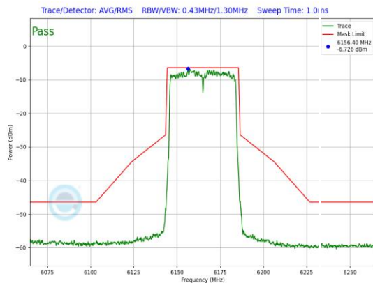
Plot 7-914. LPI In-Band Emission Plot Antenna WF7 (40MHz 802.11ax (UNII Band 5) – Ch. 43, MCS11)
