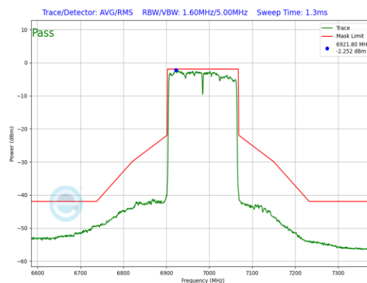
Plot 7-821. LPI In-Band Emission Plot Antenna WF8 (160MHz 802.11ax (UNII Band 8) – Ch. 207, MCS4)
