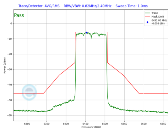
Plot 7-830. LPI In-Band Emission Plot Antenna WF8 (80MHz 802.11ax (UNII Band 6) – Ch. 103, MCS11)
