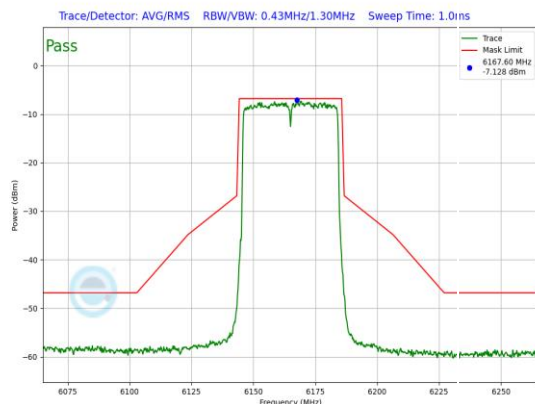
Plot 7-874. LPI In-Band Emission Plot Antenna WF7 (40MHz 802.11ax (UNII Band 5) – Ch. 43, MCS2)
