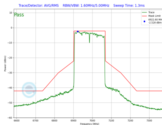
Plot 7-911. LPI In-Band Emission Plot Antenna WF7 (160MHz 802.11ax (UNII Band 8) – Ch. 207, MCS4)
