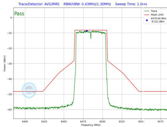
Plot 7-879. LPI In-Band Emission Plot Antenna WF7 (40MHz 802.11ax (UNII Band 6) – Ch. 107, MCS2)
