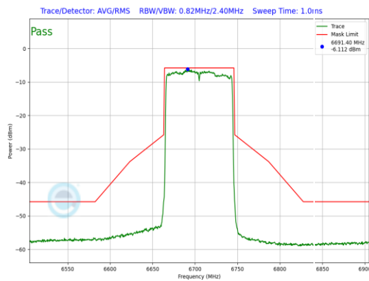
Plot 7-795. LPI In-Band Emission Plot Antenna WF8 (80MHz 802.11ax (UNII Band 7) – Ch. 151, MCS2)
