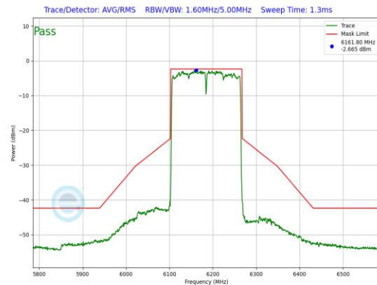
Plot 7-896. LPI In-Band Emission Plot Antenna WF7 (160MHz 802.11ax (UNII Band 5) – Ch. 47, MCS4)
