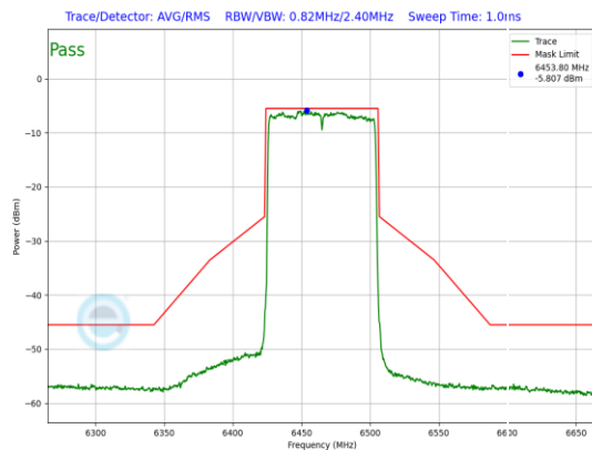
Plot 7-790. LPI In-Band Emission Plot Antenna WF8 (80MHz 802.11ax (UNII Band 6) – Ch. 103, MCS2)
