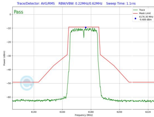
Plot 7-913. LPI In-Band Emission Plot Antenna WF7 (20MHz 802.11ax (UNII Band 5) – Ch. 45, MCS11)
