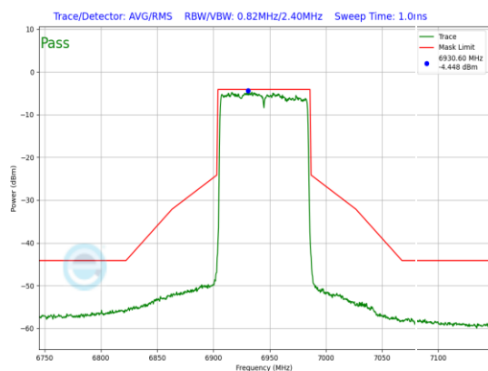
Plot 7-820. LPI In-Band Emission Plot Antenna WF8 (80MHz 802.11ax (UNII Band 8) – Ch. 199, MCS4)
