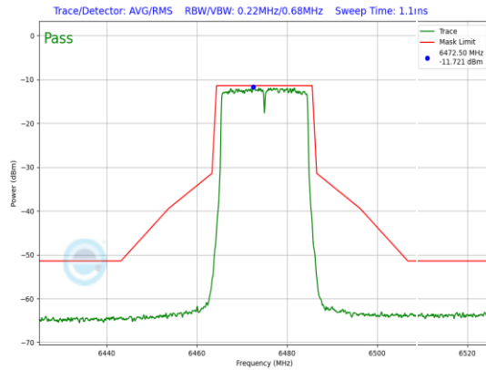
Plot 7-788. LPI In-Band Emission Plot Antenna WF8 (20MHz 802.11ax (UNII Band 6) – Ch. 105, MCS2)
