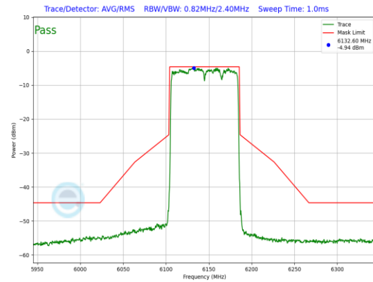
Plot 7-915. LPI In-Band Emission Plot Antenna WF7 (80MHz 802.11ax (UNII Band 5) – Ch. 39, MCS11)
