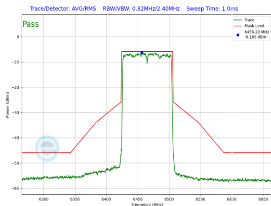
Plot 7-920. LPI In-Band Emission Plot Antenna WF7 (80MHz 802.11ax (UNII Band 6) – Ch. 103, MCS11)
