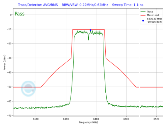
Plot 7-828. LPI In-Band Emission Plot Antenna WF8 (20MHz 802.11ax (UNII Band 6) – Ch. 105, MCS11)
