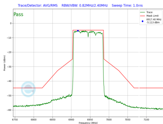
Plot 7-840. LPI In-Band Emission Plot Antenna WF8 (80MHz 802.11ax (UNII Band 8) – Ch. 199, MCS11)
