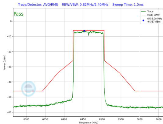
Plot 7-880. LPI In-Band Emission Plot Antenna WF7 (80MHz 802.11ax (UNII Band 6) – Ch. 103, MCS2)
