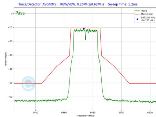
Plot 7-917. LPI In-Band Emission Plot Antenna WF7 (20MHz 802.11a (UNII Band 6) – Ch. 105, 54Mbps)
