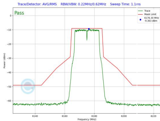
Plot 7-872. LPI In-Band Emission Plot Antenna WF7 (20MHz 802.11a (UNII Band 5) – Ch. 45, 12Mbps)
