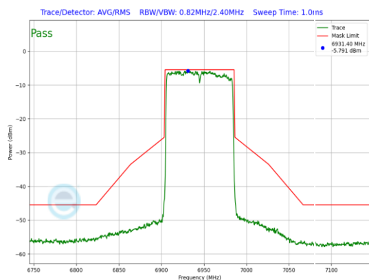
Plot 7-910. LPI In-Band Emission Plot Antenna WF7 (80MHz 802.11ax (UNII Band 8) – Ch. 199, MCS4)
