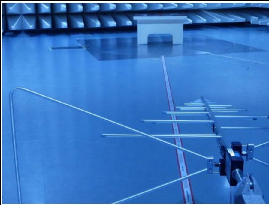
Test setup AC 6 horizontal polarization up to 1 GHz
