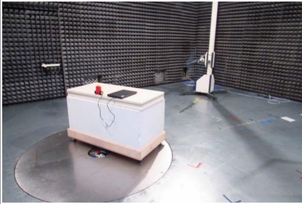
Setup for TX measurement below 1 GHz
