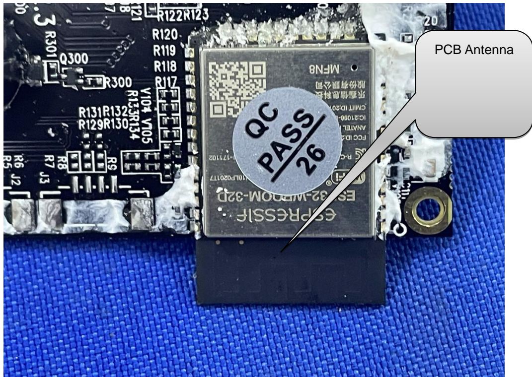
Antenna Position
