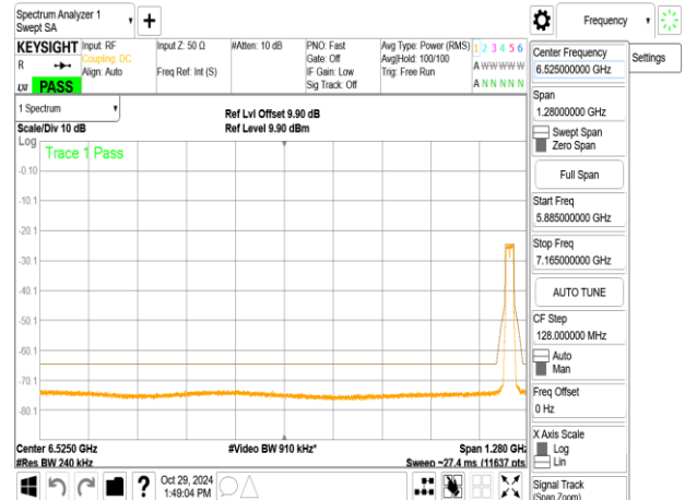
802.11ax_20MHz_ChainB_7115MHz_RU106_54
