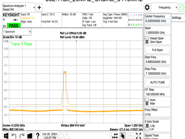
802.11ax_20MHz_ChainB_6415MHz_RU106_54
