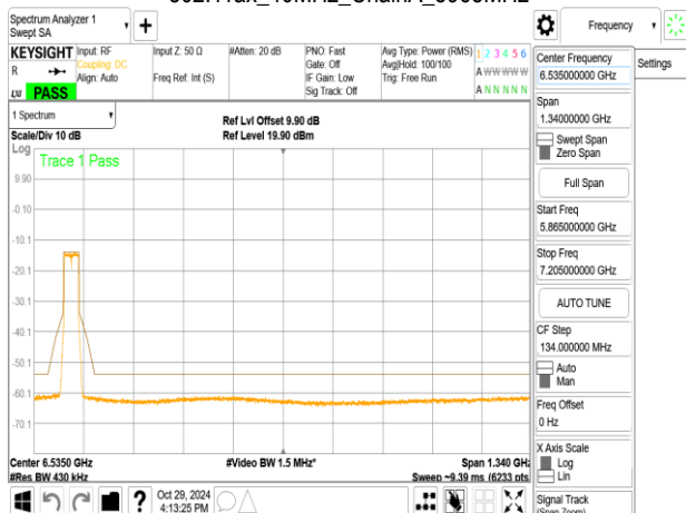
802.11ax_40MHz_ChainA_5965MHz
