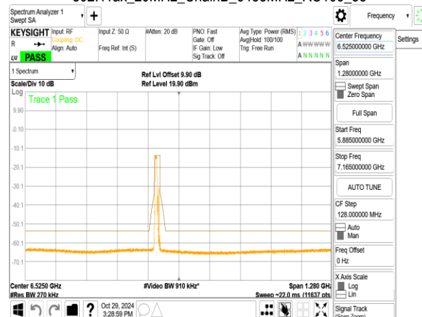
802.11ax_20MHz_ChainB_6435MHz_RU106_53
