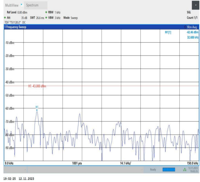
Band2_15MHz_16QAM_19125_1RB#0_0.009~0.15_0.009~0.15
