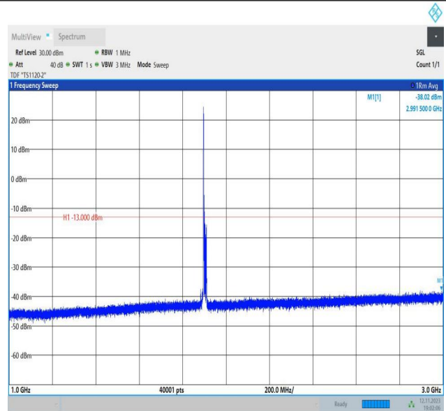
Band2_15MHz_QPSK_19125_1RB#0_1000~3000_1000~3000
