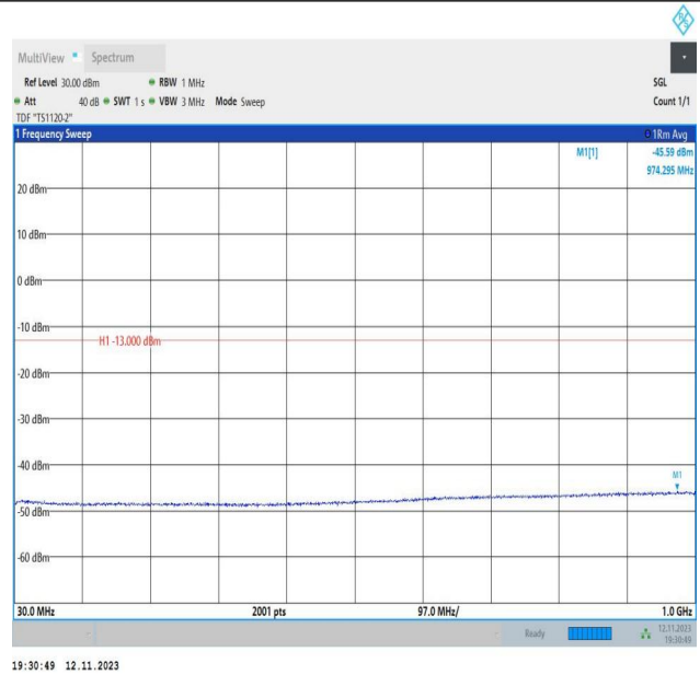
Band2_20MHz_16QAM_18900_1RB#0_30~1000_30~1000
