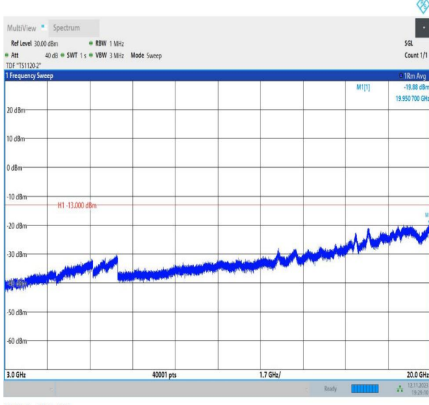
Band2_20MHz_QPSK_18700_1RB#0_3000~20000_3000~20000
