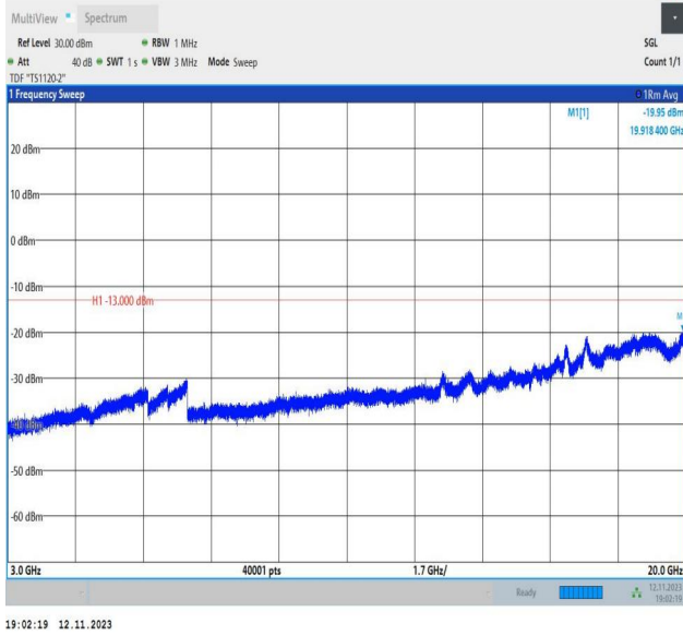
Band2_15MHz_QPSK_19125_1RB#0_3000~20000_3000~20000
