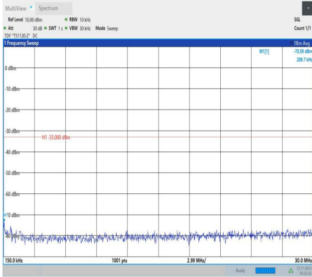
Band2_20MHz_16QAM_19100_1RB#0_0.15~30_0.15~30
