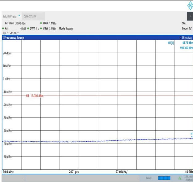
Band2_20MHz_QPSK_18700_1RB#0_30~1000_30~1000
