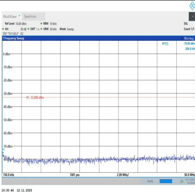
Band2_20MHz_16QAM_18900_1RB#0_0.15~30_0.15~30
