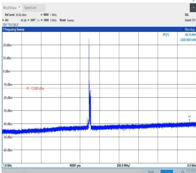
Band2_20MHz_16QAM_19100_1RB#0_1000~3000_1000~30 00
