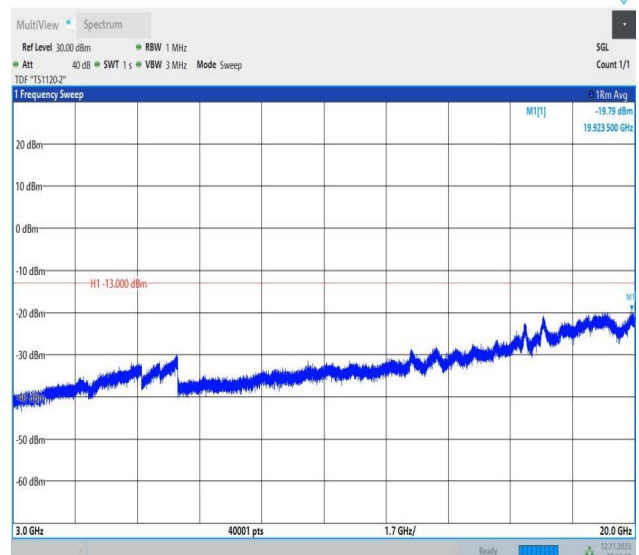
Band2_20MHz_16QAM_19100_1RB#0_3000~20000_3000~20 000
