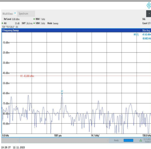
Band2_20MHz_QPSK_18700_1RB#0_0.009~0.15_0.009~0.15
