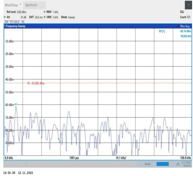
Band2_20MHz_16QAM_18900_1RB#0_0.009~0.15_0.009~0.15
