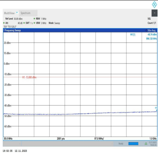
Band2_15MHz_16QAM_19125_1RB#0_30~1000_30~1000
