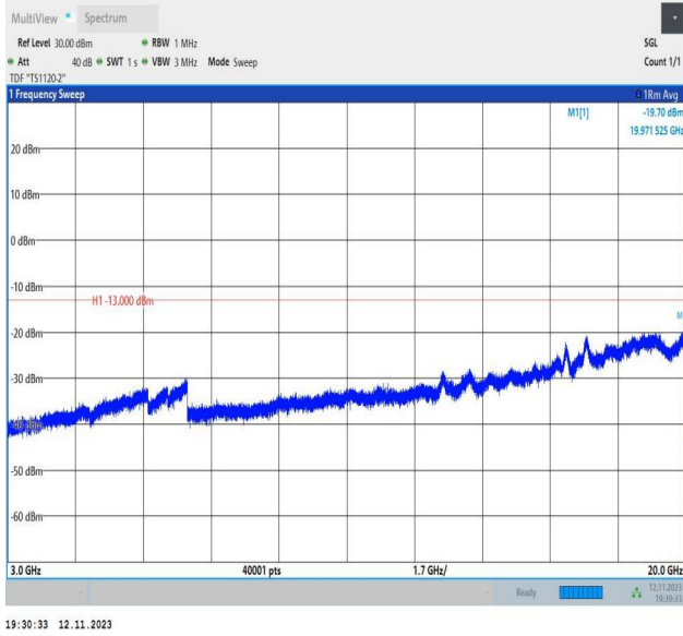
Band2_20MHz_QPSK_18900_1RB#0_3000~20000_3000~20000
