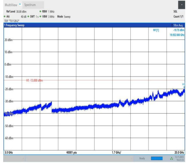
Band2_20MHz_16QAM_18900_1RB#0_3000~20000_3000~20000
