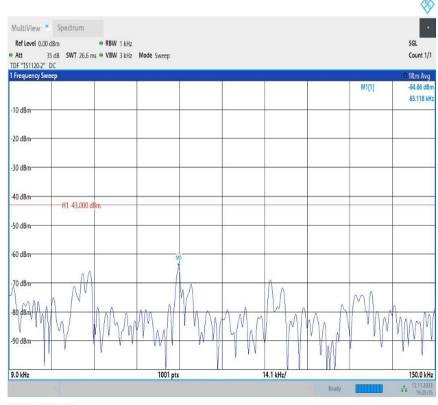
Band2_20MHz_16QAM_18700_1RB#0_0.009~0.15_0.009~0.15
