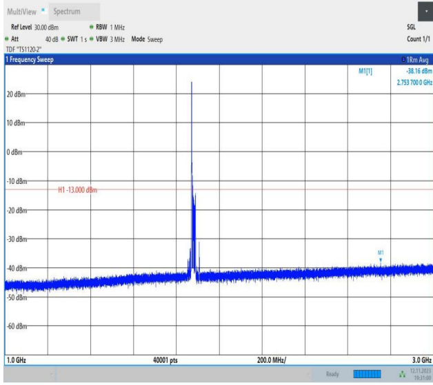
Band2_20MHz_16QAM_18900_1RB#0_1000~3000_1000~3000
