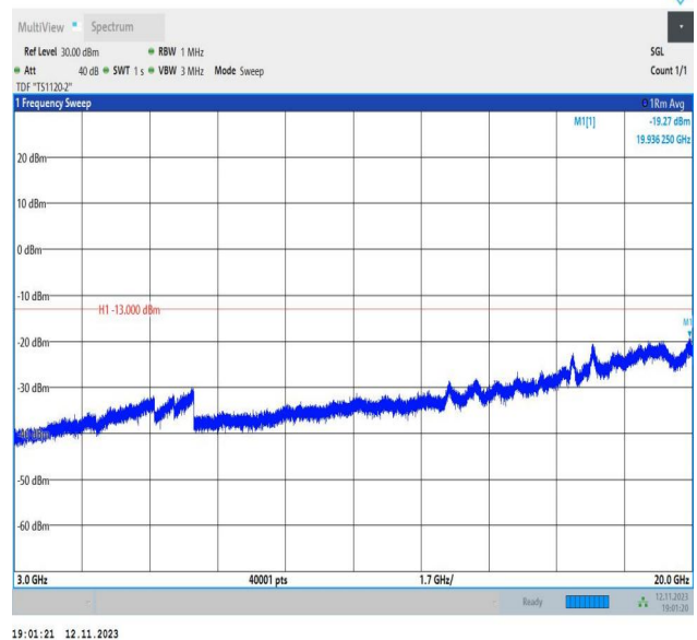
Band2_15MHz_16QAM_18900_1RB#0_3000~20000_3000~20 000
