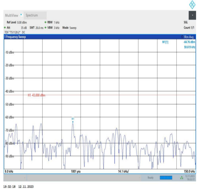
Band2_20MHz_16QAM_19100_1RB#0_0.009~0.15_0.009~0.1
