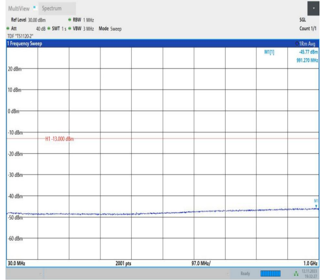
Band2_20MHz_16QAM_19100_1RB#0_30~1000_30~1000
