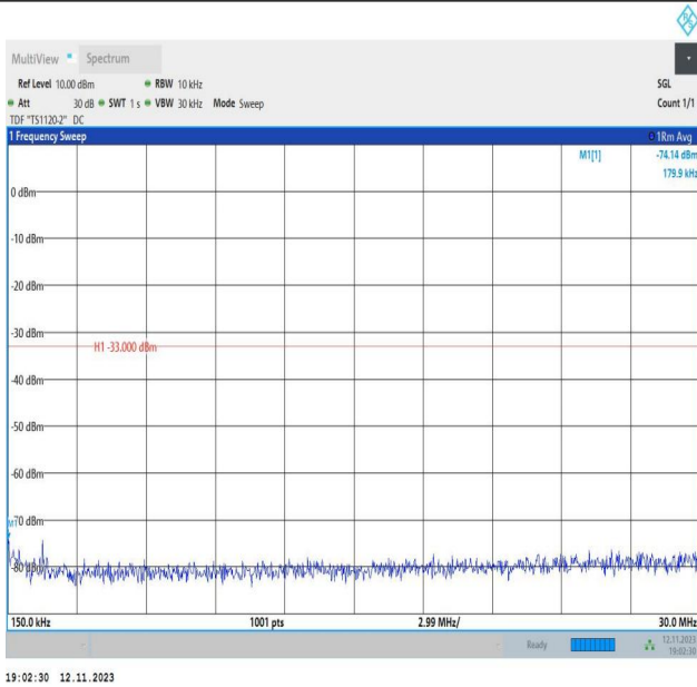
Band2_15MHz_16QAM_19125_1RB#0_0.15~30_0.15~30
