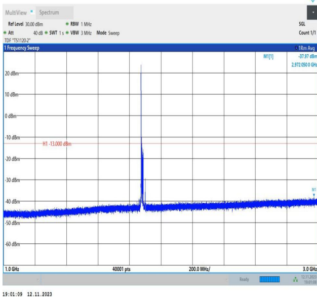
Band2_15MHz_16QAM_18900_1RB#0_1000~3000_1000~30 00
