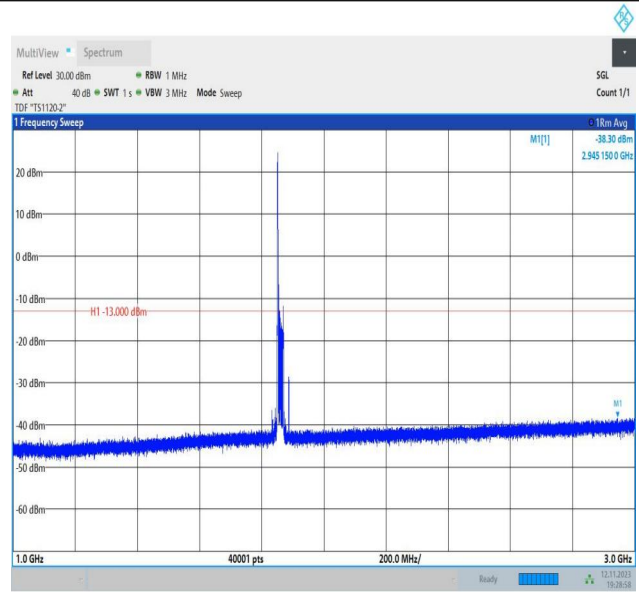
Band2_20MHz_QPSK_18700_1RB#0_1000~3000_1000~3000
