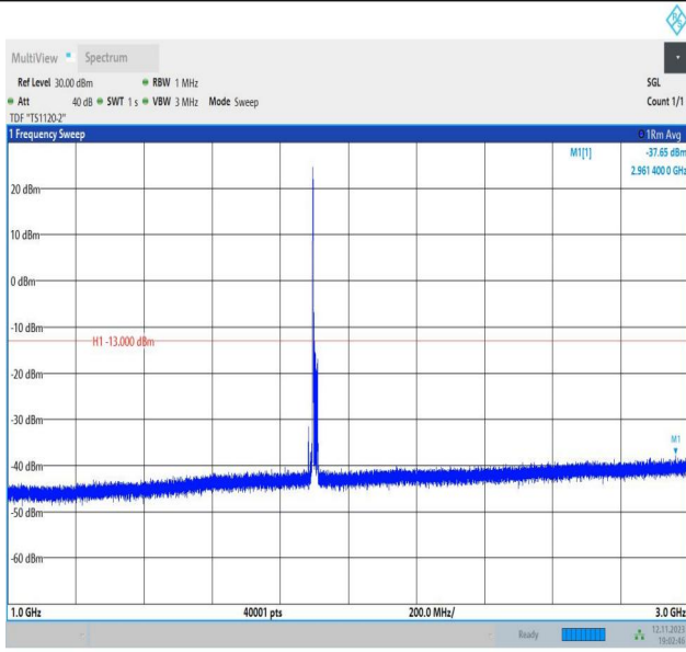
Band2_15MHz_16QAM_19125_1RB#0_1000~3000_1000~3000
