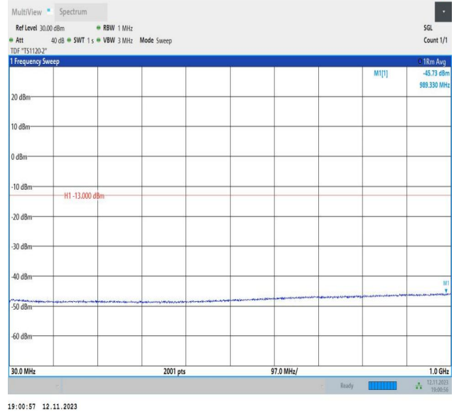
Band2_15MHz_16QAM_18900_1RB#0_30~1000_30~1000
