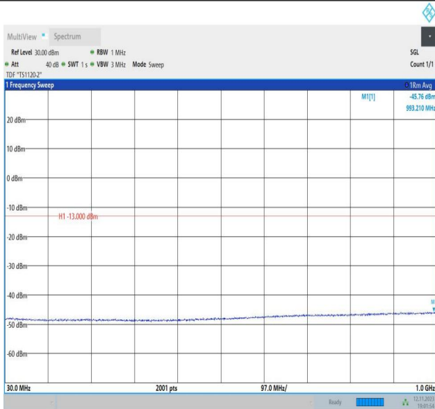
Band2_15MHz_QPSK_19125_1RB#0_30~1000_30~1000
