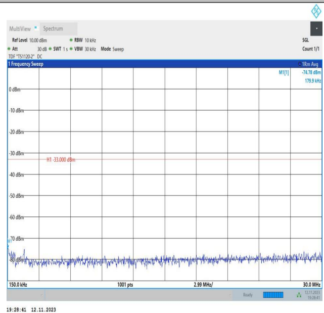
Band2_20MHz_QPSK_18700_1RB#0_0.15~30_0.15~30
