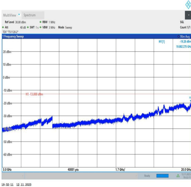
Band2_20MHz_QPSK_19100_1RB#0_3000~20000_3000~20000
