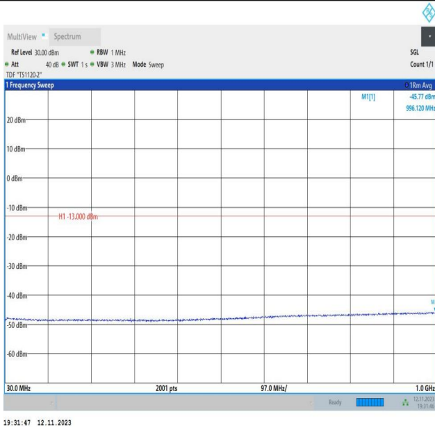
Band2_20MHz_QPSK_19100_1RB#0_30~1000_30~1000
