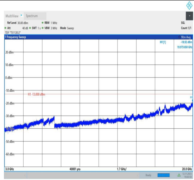
Band2_15MHz_16QAM_19125_1RB#0_3000~20000_3000~20000
