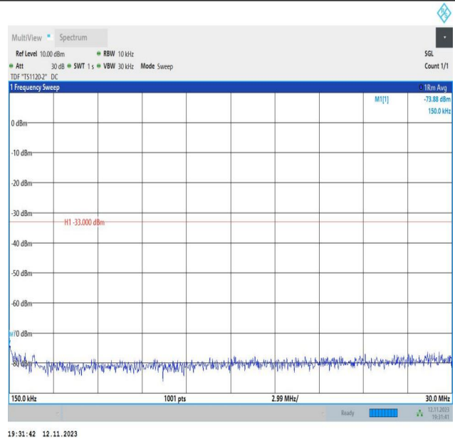
Band2_20MHz_QPSK_19100_1RB#0_0.15~30_0.15~30
