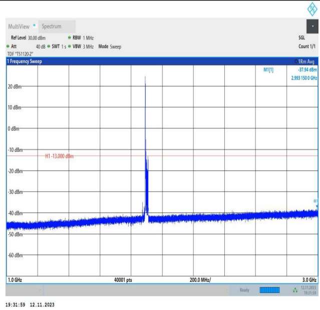
Band2_20MHz_QPSK_19100_1RB#0_1000~3000_1000~3000
