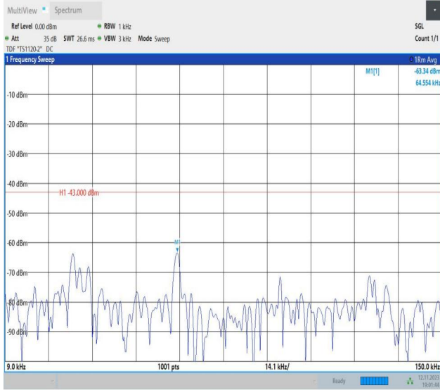
Band2_15MHz_QPSK_19125_1RB#0_0.009~0.15_0.009~0.1
