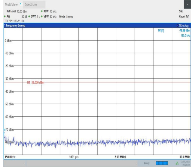
Band2_15MHz_QPSK_19125_1RB#0_0.15~30_0.15~30
