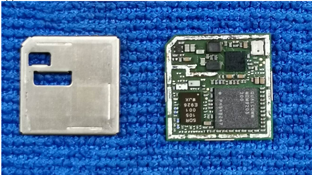
(1) EUT Photo
