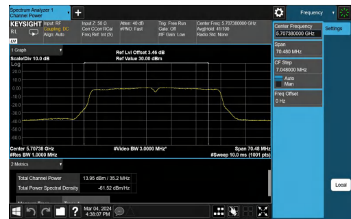
11AC40SISO-Ant1-5710_UNII-2C-TPC_L-PASS
