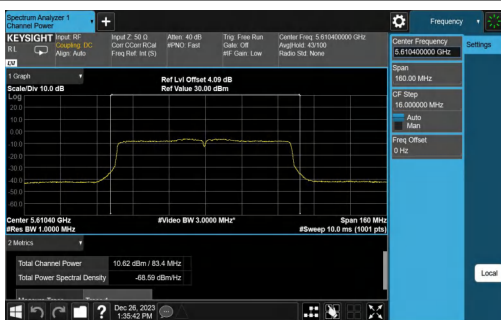
11AC80MIMO-Ant0-5610-TPC_L-PASS
