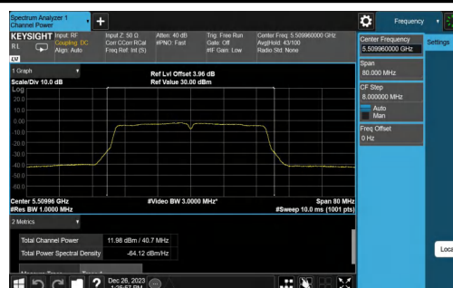
11AC40MIMO-Ant1-5510-TPC_L-PASS
