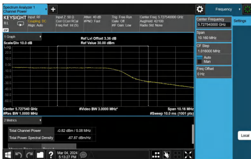
11AC40MIMO-Ant0-5710_UNII-3-TPC_L-PASS
