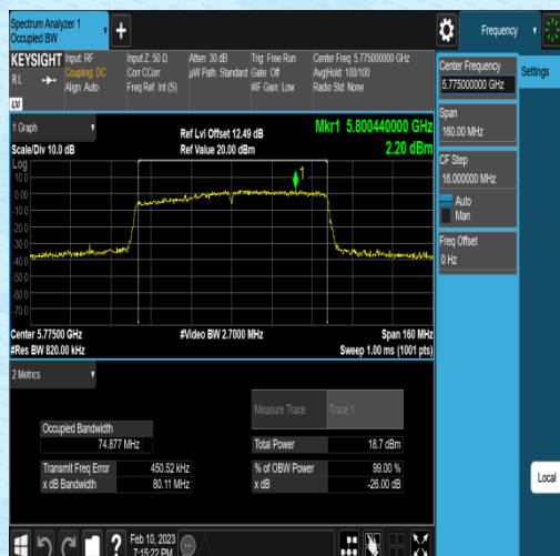
11AC80MIMO-Ant2-5775
