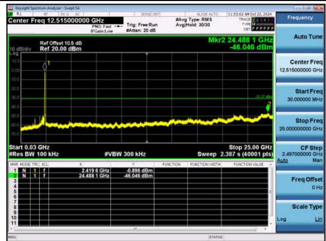
11AX40SISO-Ant1-2437-30~25000-PASS
