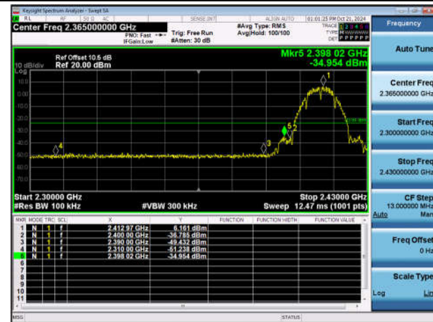
11G-Ant1-2412-PASS
