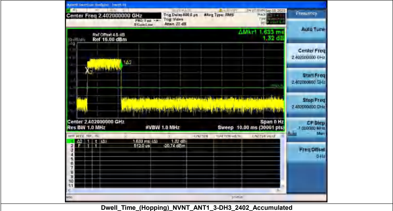
Dwell_Time_(Hopping)_NVNT_ANT1_3-DH3_2402_Accumulated
