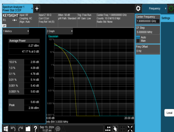
Band2-3MHz-QPSK-19185-1RB#0-PASS
