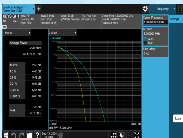
Band2-15MHz-QPSK-19125-1RB#0-PASS
