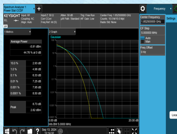
Band2-5MHz-16QAM-18625-25RB#0-PASS
