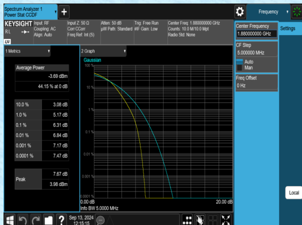
Band2-5MHz-16QAM-18900-1RB#0-PASS
