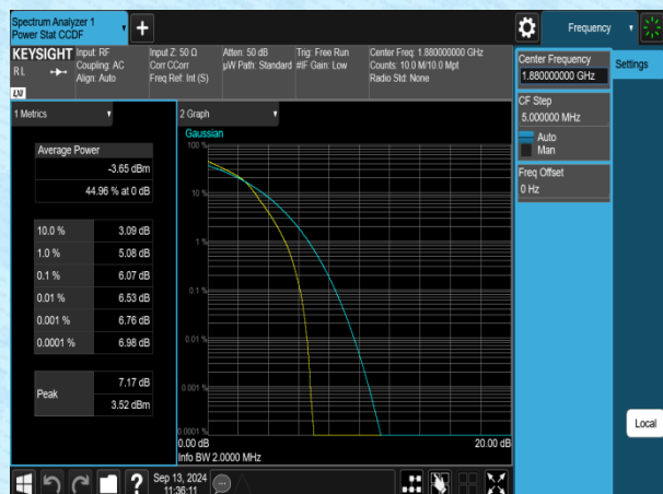
Band2-1.4MHz-16QAM-18900-1RB#0-PASS
