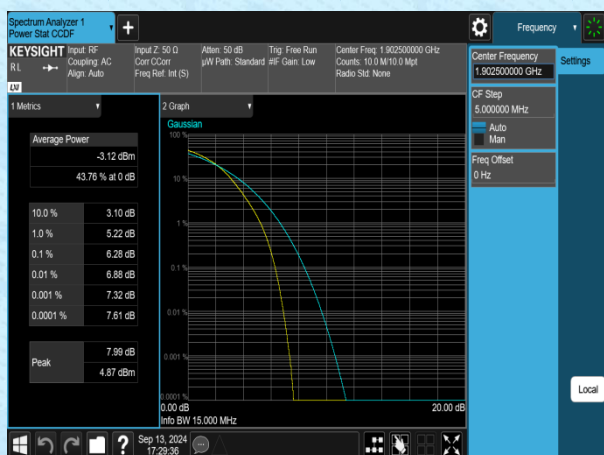
Band2-15MHz-16QAM-19125-1RB#0-PASS
