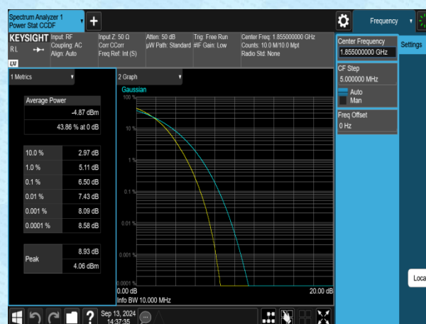
Band2-10MHz-16QAM-18650-50RB#0-PASS
