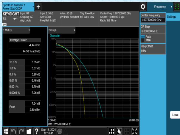
Band2-5MHz-16QAM-19175-1RB#0-PASS
