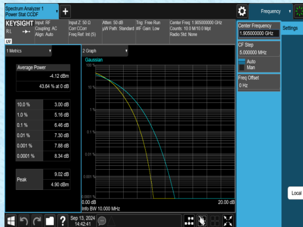
Band2-10MHz-16QAM-19150-50RB#0-PASS
