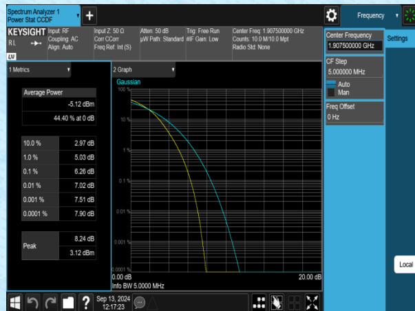
Band2-5MHz-16QAM-19175-25RB#0-PASS
