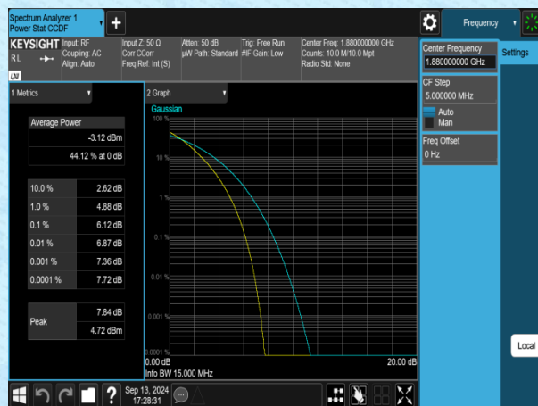
Band2-15MHz-QPSK-18900-75RB#0-PASS
