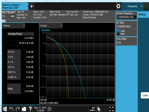
Band2-3MHz-16QAM-19185-1RB#0-PASS
