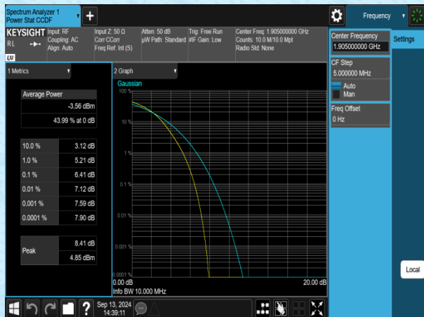
Band2-10MHz-16QAM-19150-1RB#0-PASS
