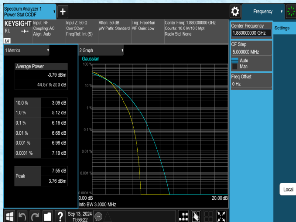
Band2-3MHz-16QAM-18900-1RB#0-PASS
