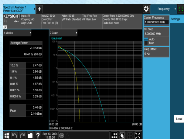
Band2-1.4MHz-QPSK-19193-1RB#0-PASS
