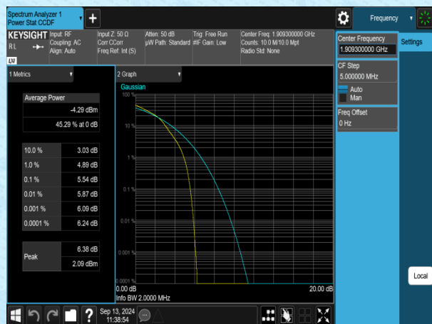
Band2-1.4MHz-16QAM-19193-1RB#0-PASS
