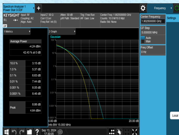
Band2-15MHz-16QAM-19125-75RB#0-PASS
