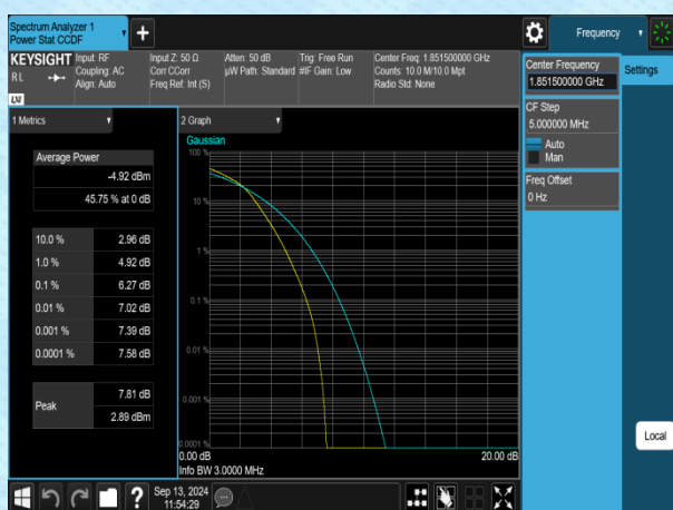
Band2-3MHz-16QAM-18615-1RB#0-PASS
