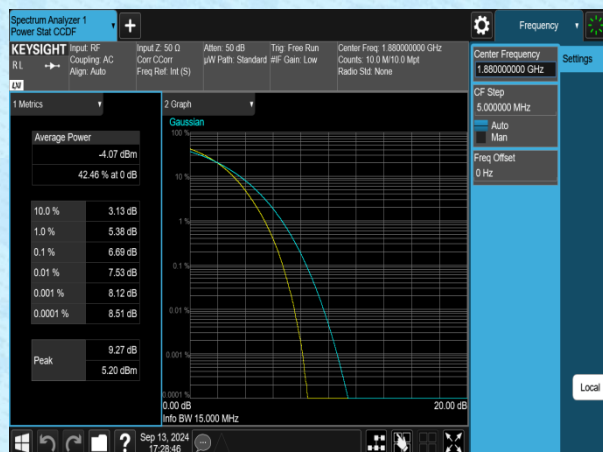
Band2-15MHz-16QAM-18900-75RB#0-PASS
