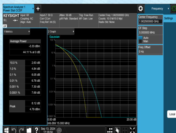
Band2-15MHz-QPSK-19125-75RB#0-PASS
