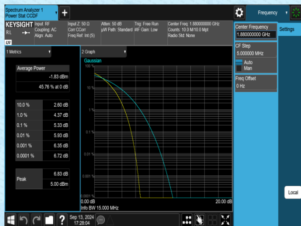
Band2-15MHz-QPSK-18900-1RB#0-PASS
