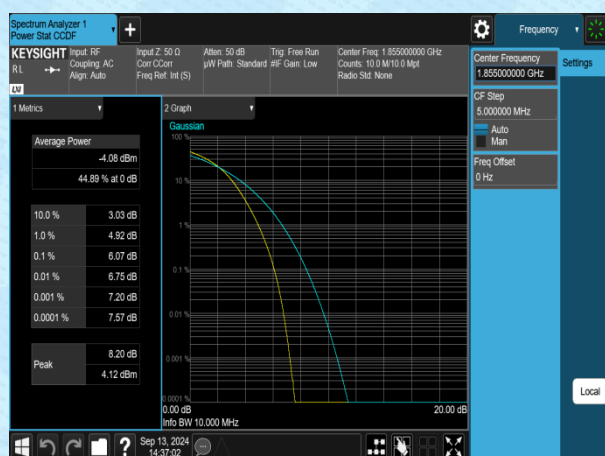
Band2-10MHz-16QAM-18650-1RB#0-PASS
