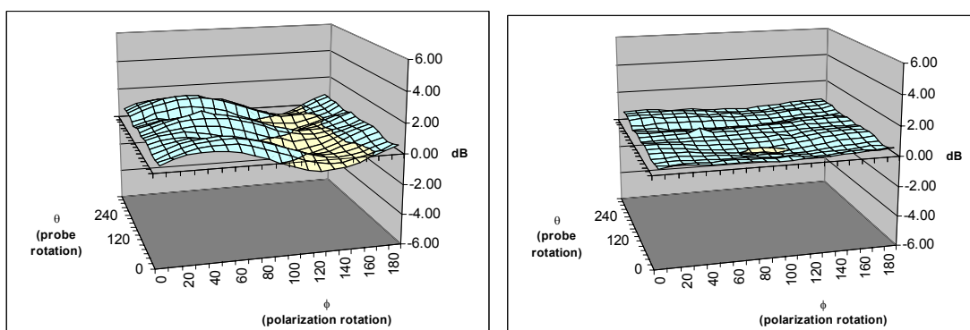
Figure 8: Probe isotropy at 2450MHz with probe oriented at 90 degrees to field gradient direction. At left, uncorrected readings. At right, corrected for sensor displacement.
