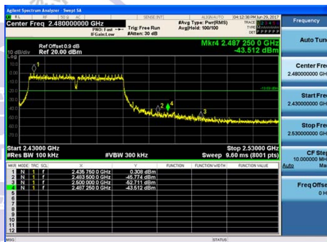
Right bandedge
