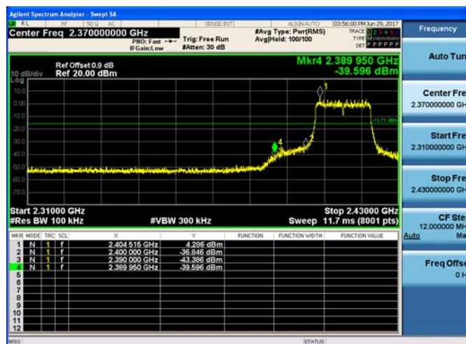
Left bandedge
