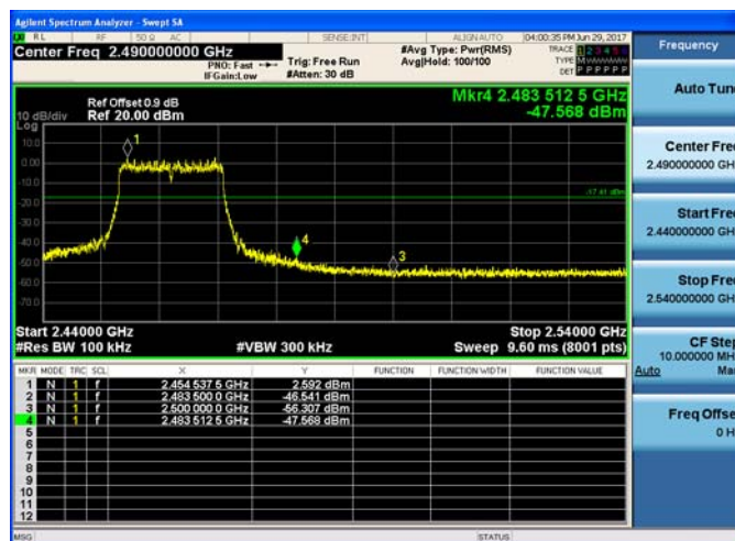
Right bandedge
