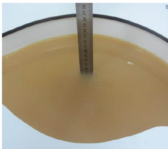
Photo 19: MBBL600-6000MHz Depth (15.2cm)
