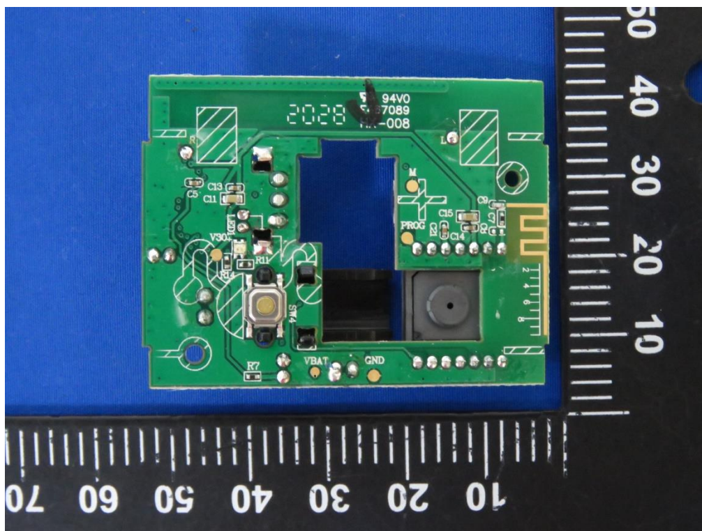
SRD Antenna
