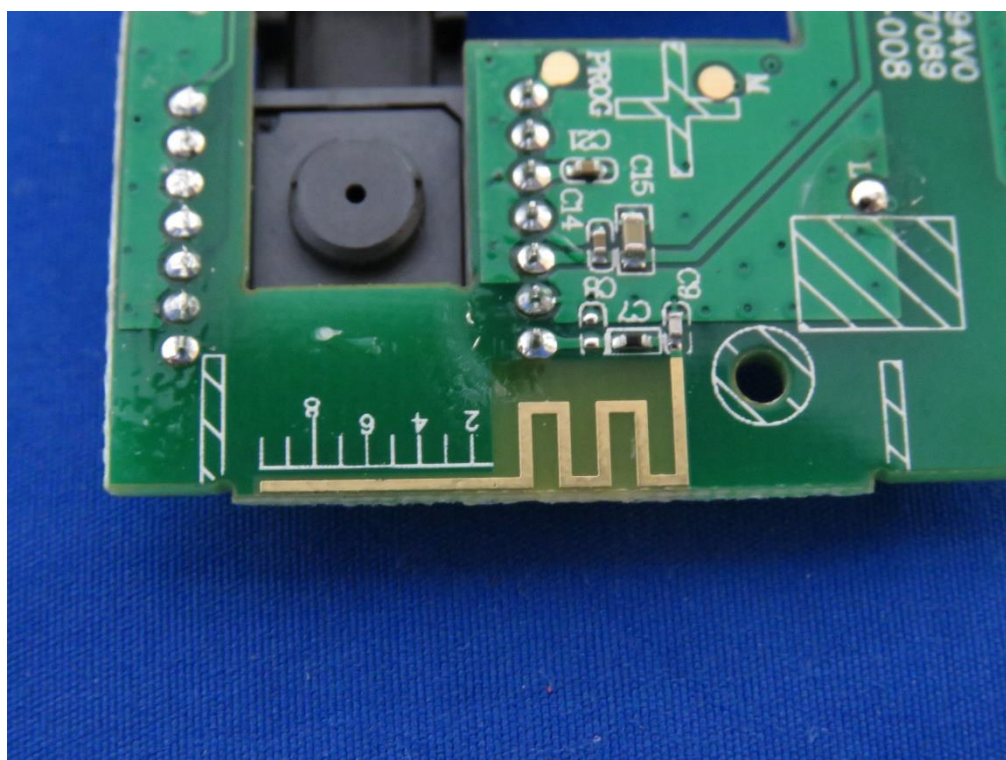
SRD Antenna
