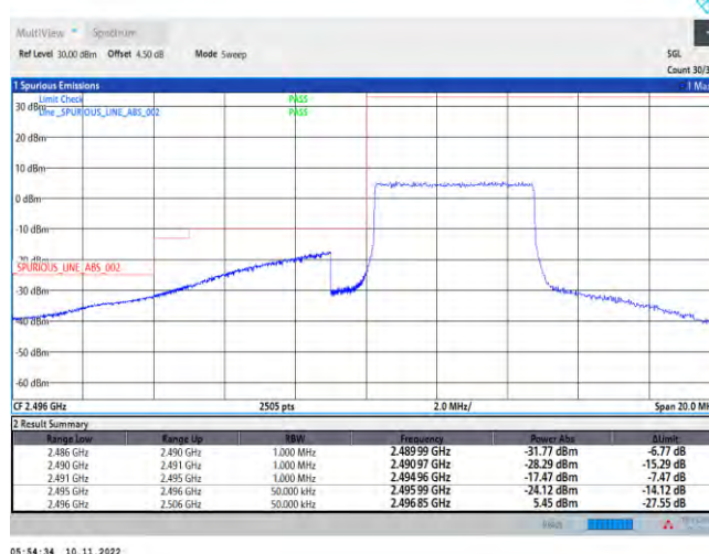
Band41-5MHz-QPSK-39675-25RB#0
