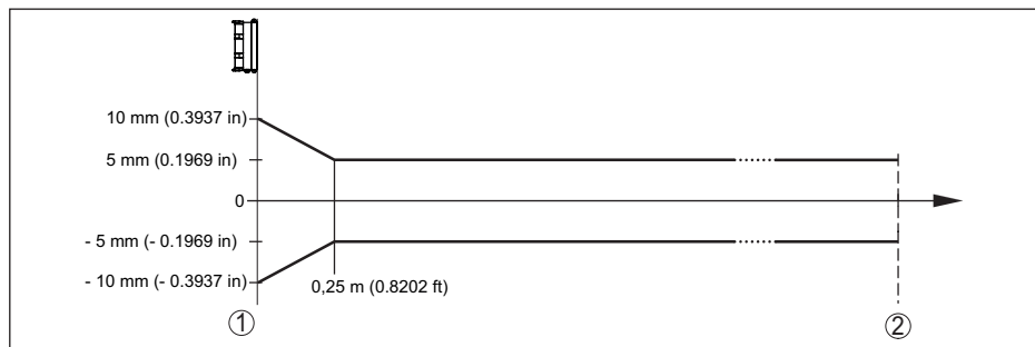
Fig. 9: Deviation under reference conditions
