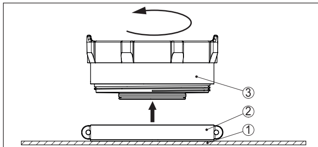
Fig. 7: Removal with glue connection
