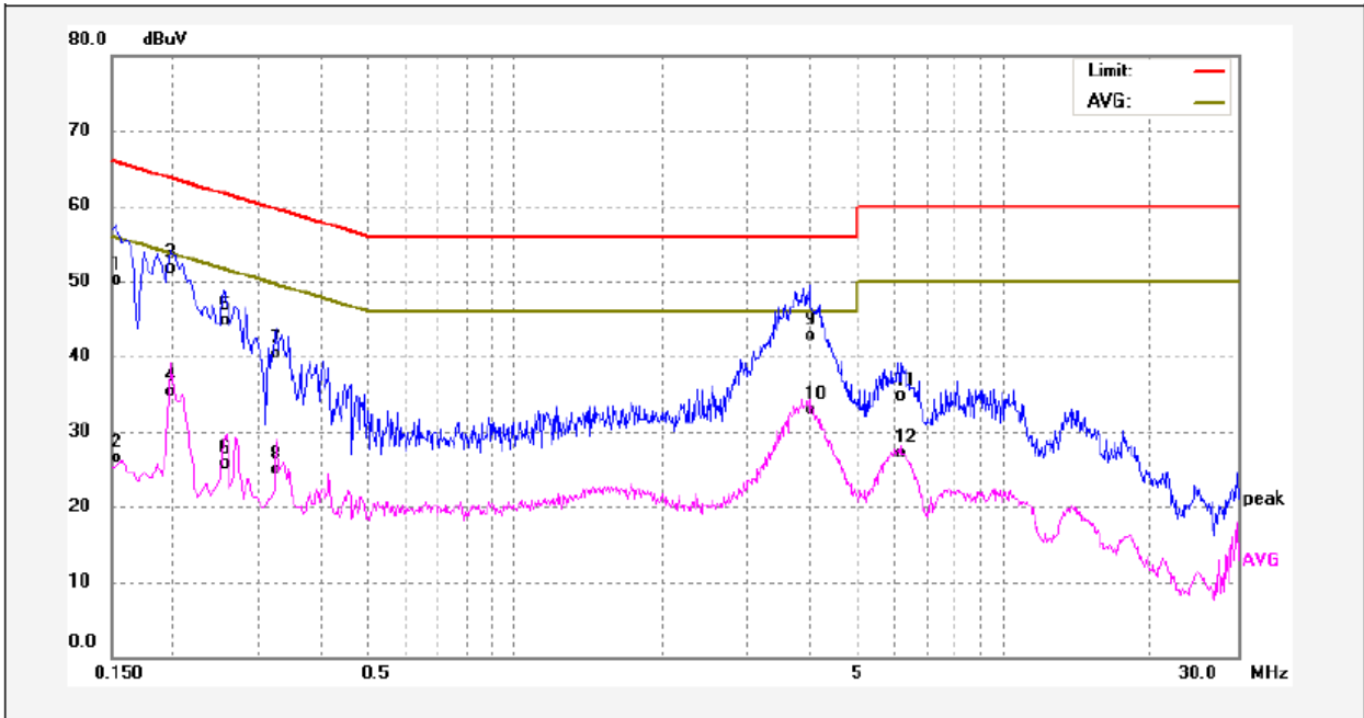
Neutral line:
