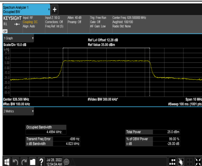
Band5-5MHz-QPSK-20425-25RB#0
