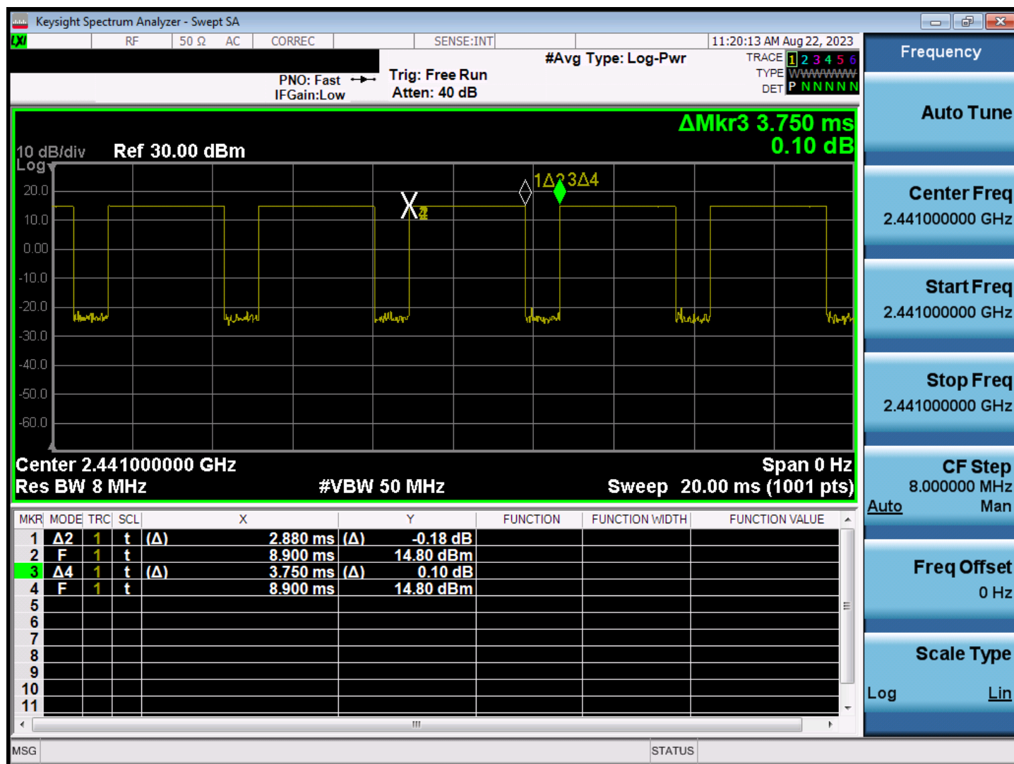
Figure 9.5.2.2 Bluetooth Transmission Plot
