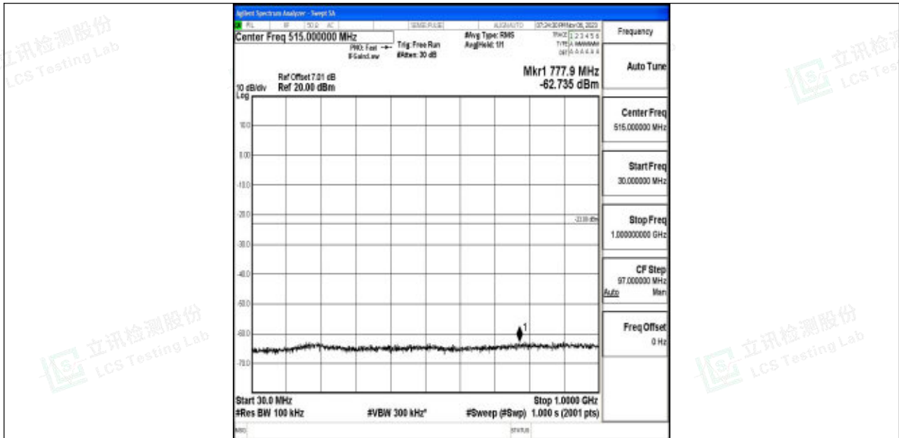
Band4_10MHz_QPSK_20000_1RB#0_30~1000_30~1000
