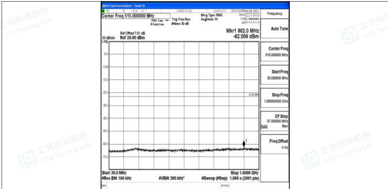
Band4_10MHz_16QAM_20175_1RB#0_30~1000_30~1000
