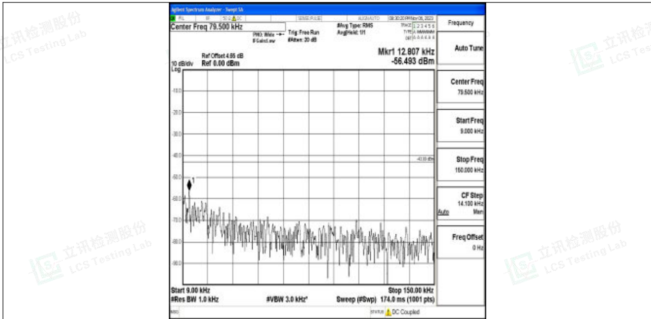
Band4_20MHz_QPSK_20300_1RB#0_0.009~0.15_0.009~0.15
