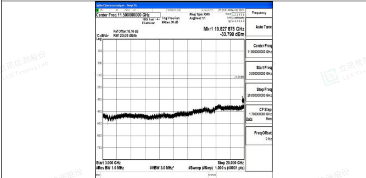
Band4_10MHz_16QAM_20350_1RB#0_3000~20000_3000~20000
