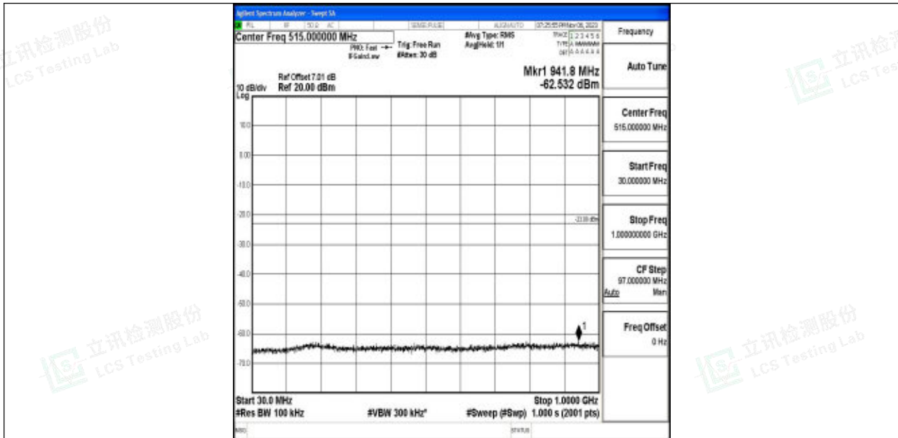
Band4_10MHz_64QAM_20000_1RB#0_30~1000_30~1000
