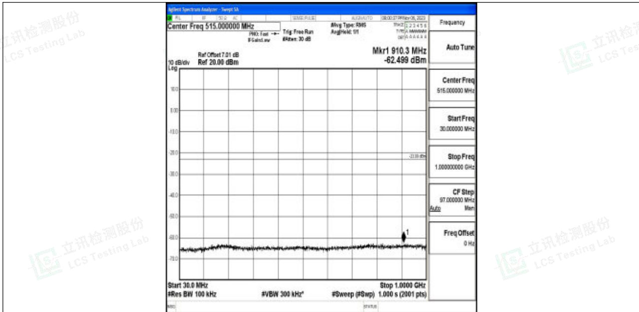
Band4_15MHz_16QAM_20325_1RB#0_30~1000_30~1000
