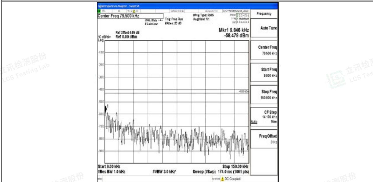
Band4_10MHz_64QAM_20175_1RB#0_0.009~0.15_0.009~0.15
