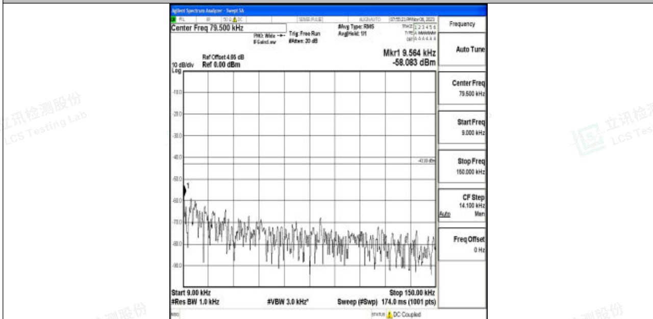
Band4_15MHz_QPSK_20025_1RB#0_0.009~0.15_0.009~0.15
