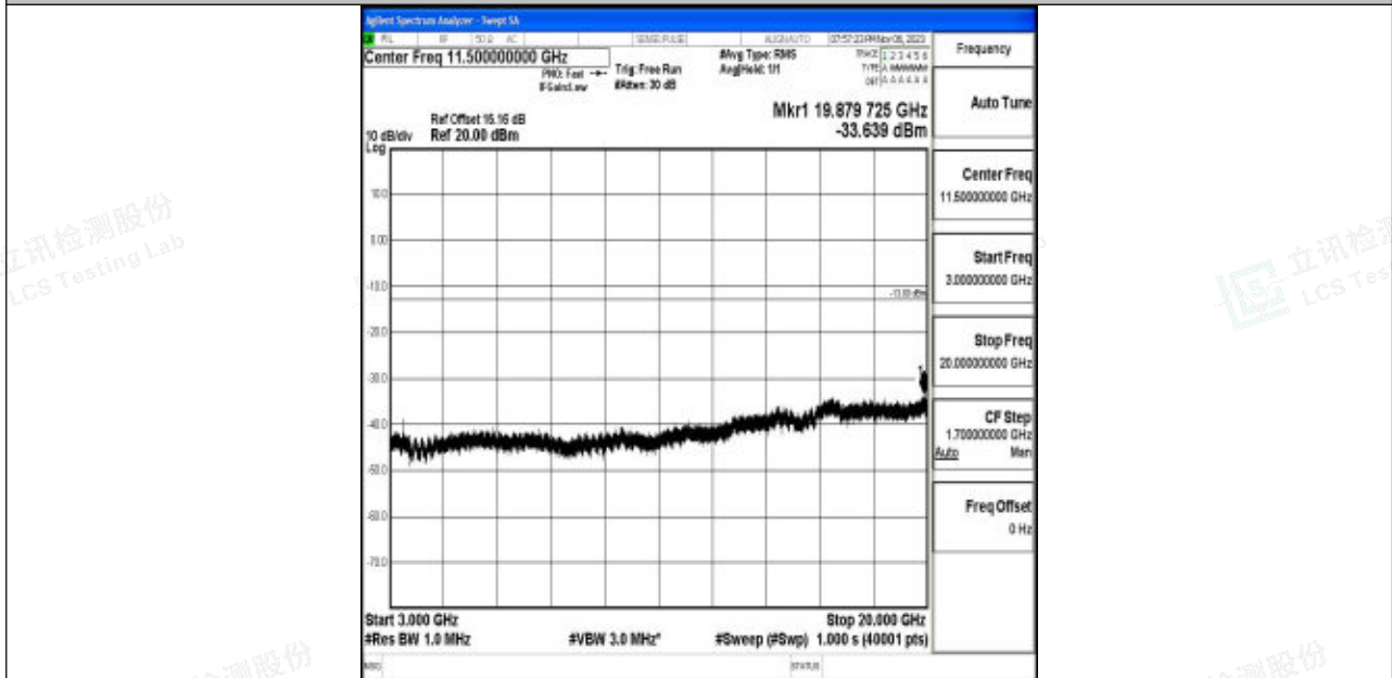
Band4_15MHz_64QAM_20025_1RB#0_3000~20000_3000~20000
