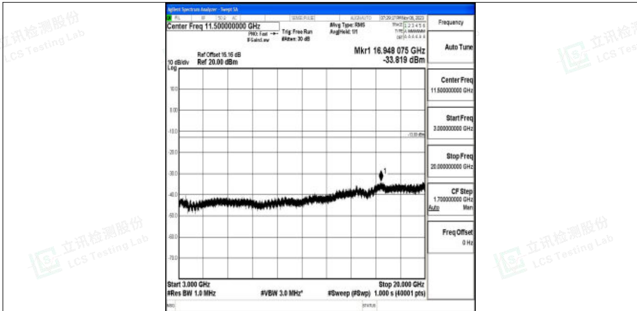
Band4_10MHz_QPSK_20350_1RB#0_3000~20000_3000~20000
