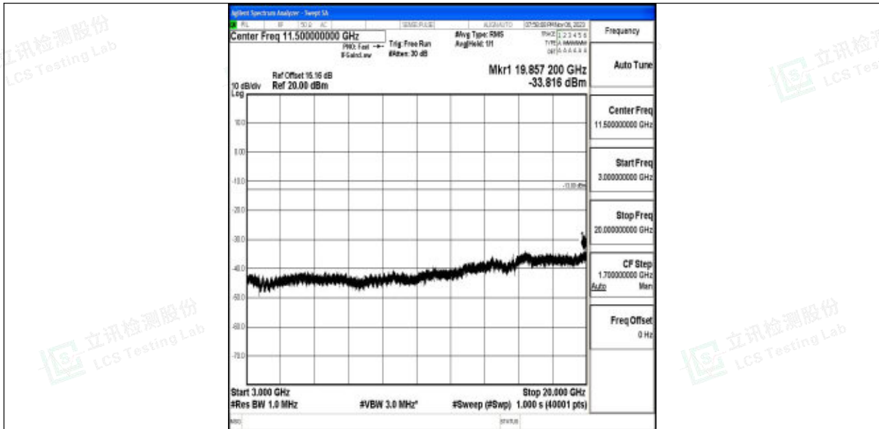
Band4_15MHz_QPSK_20175_1RB#0_3000~20000_3000~20000
