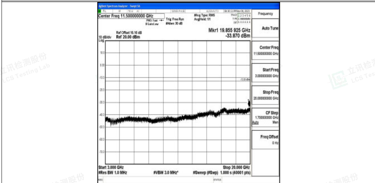
Band4_20MHz_64QAM_20175_1RB#0_3000~20000_3000~20000
