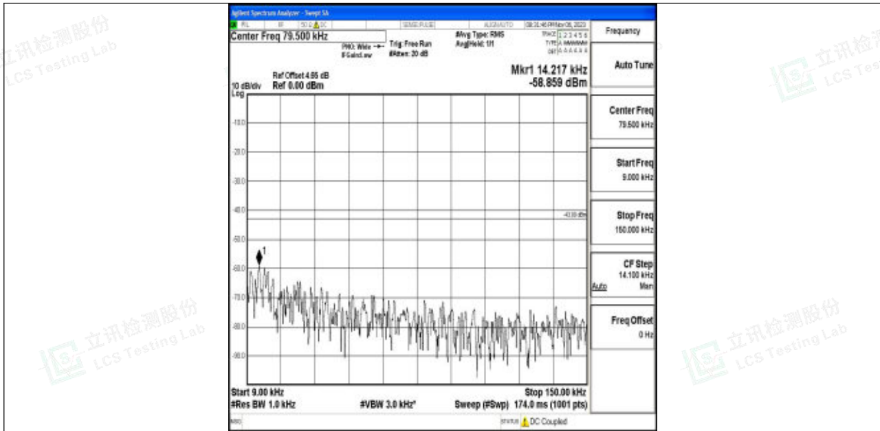
Band4_20MHz_64QAM_20300_1RB#0_0.009~0.15_0.009~0.15
