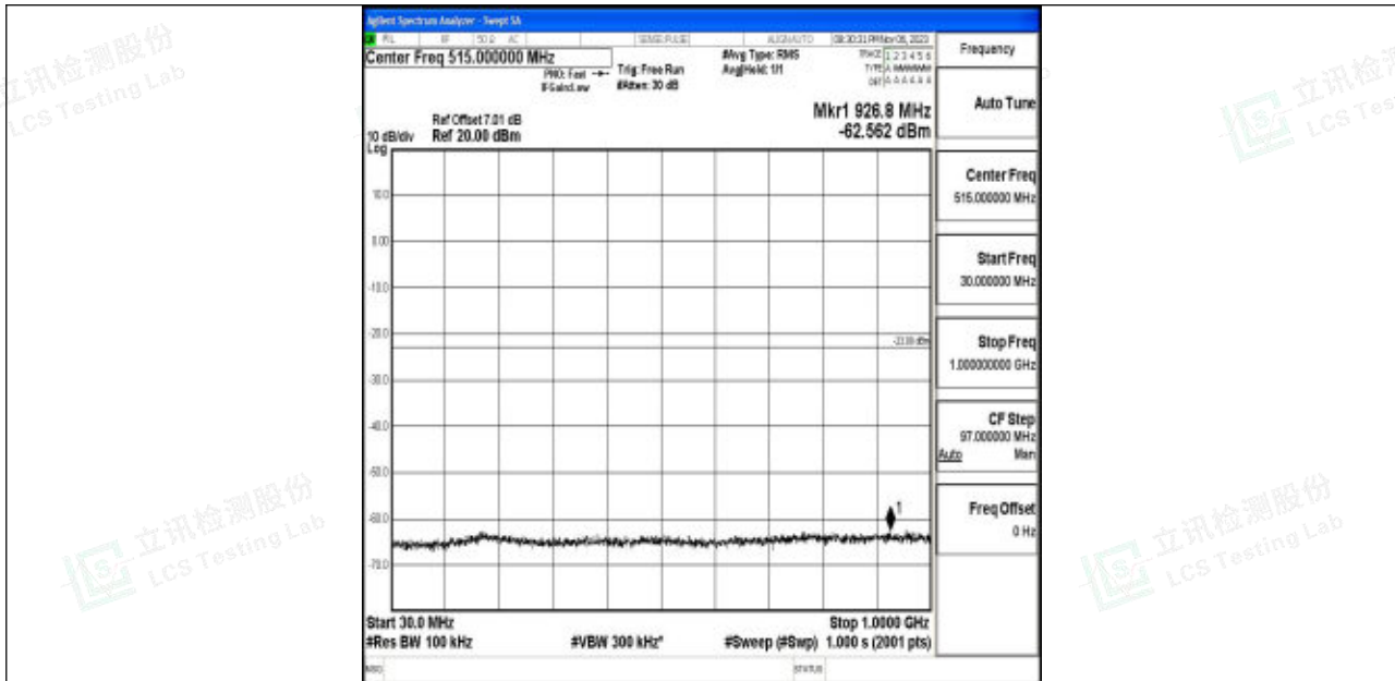
Band4_20MHz_QPSK_20300_1RB#0_30~1000_30~1000
