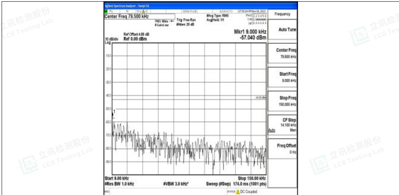
Band4_15MHz_16QAM_20025_1RB#0_0.009~0.15_0.009~0.15
