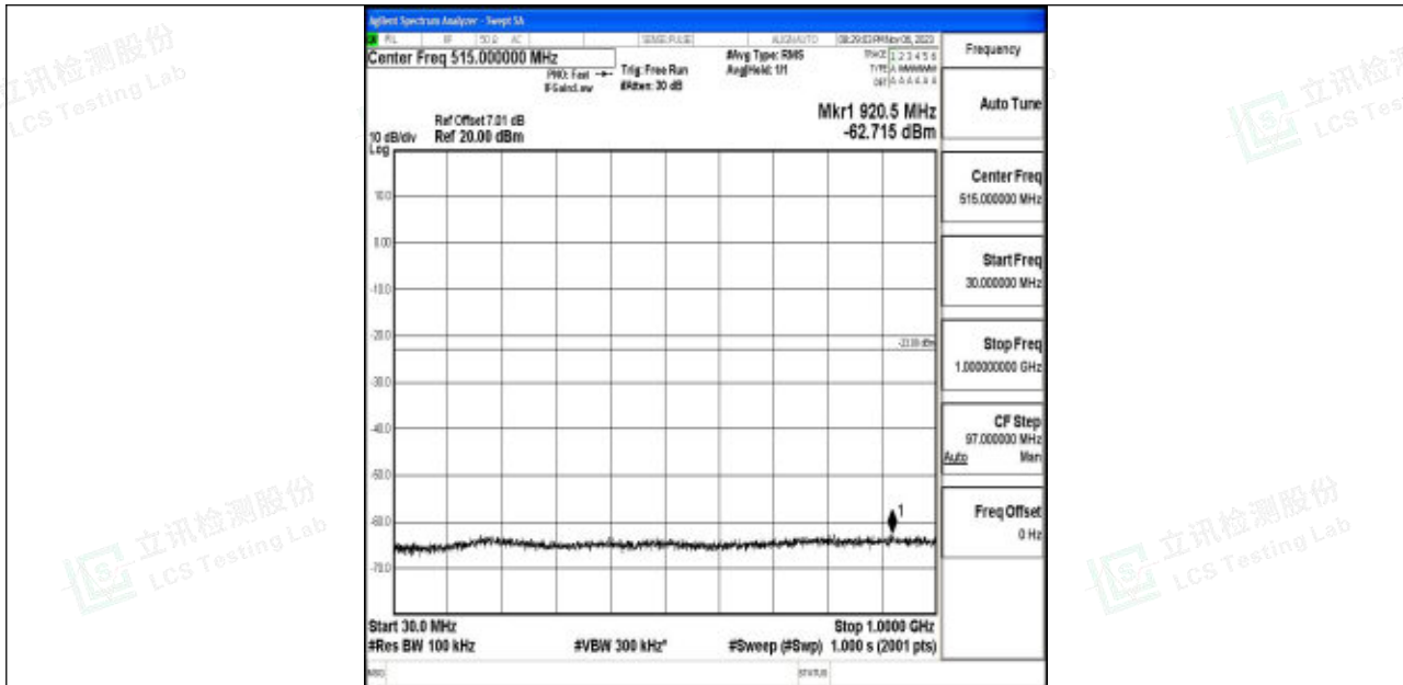
Band4_20MHz_16QAM_20175_1RB#0_30~1000_30~1000
