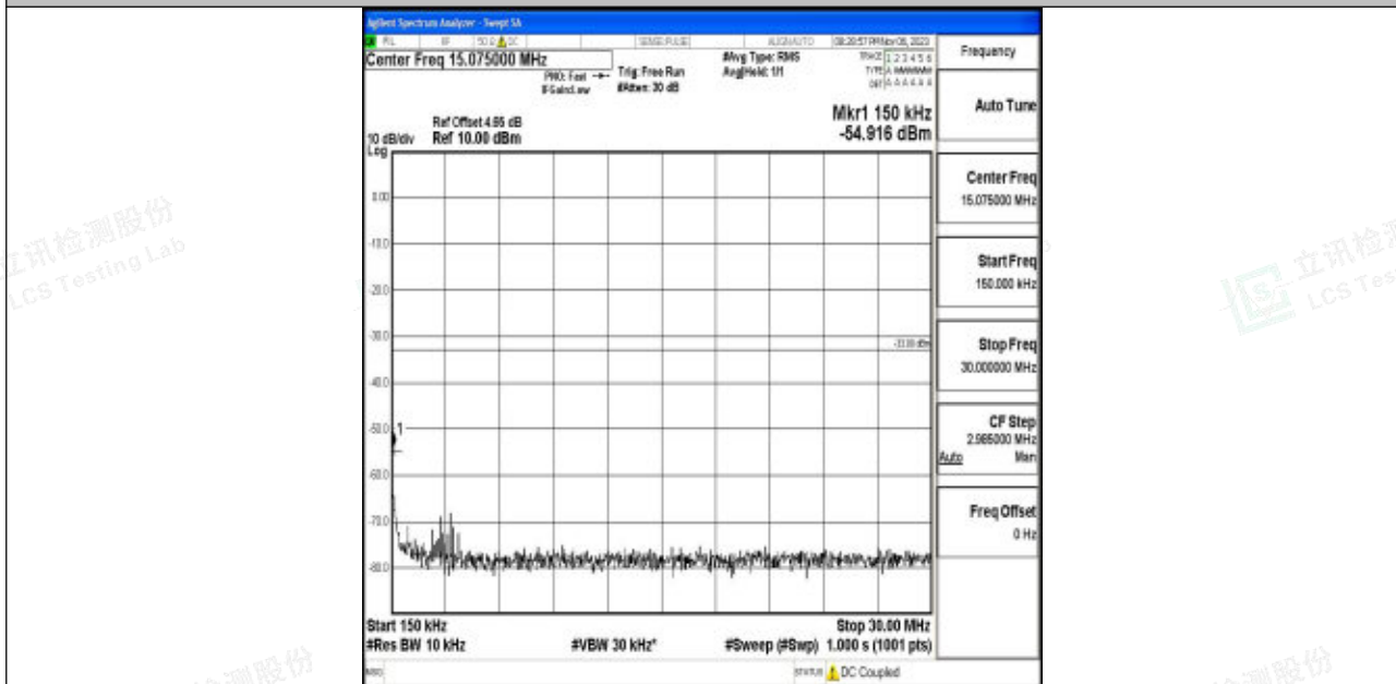
Band4_20MHz_16QAM_20175_1RB#0_0.15~30_0.15~30
