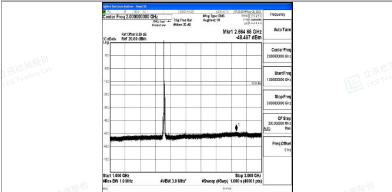
Band4_10MHz_64QAM_20000_1RB#0_1000~3000_1000~3000
