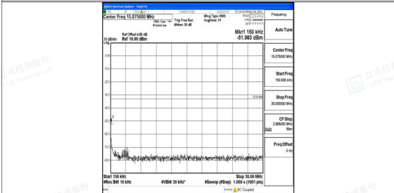
Band4_10MHz_QPSK_20000_1RB#0_0.15~30_0.15~30
