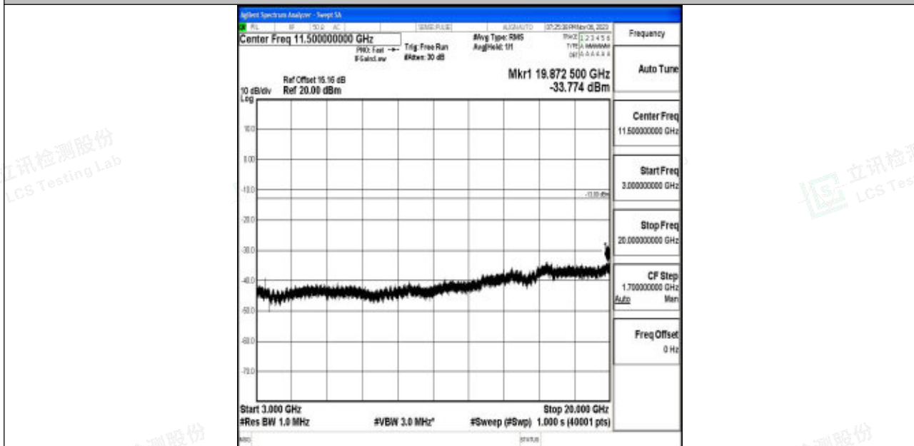
Band4_10MHz_16QAM_20000_1RB#0_3000~20000_3000~20000
