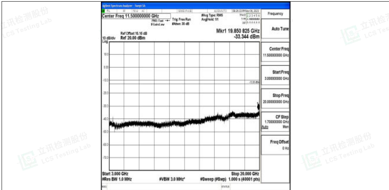
Band4_20MHz_QPSK_20050_1RB#0_3000~20000_3000~20000
