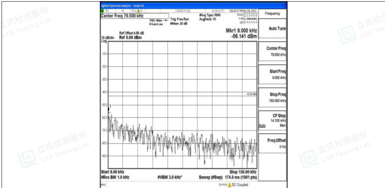
Band4_15MHz_16QAM_20325_1RB#0_0.009~0.15_0.009~0.15
