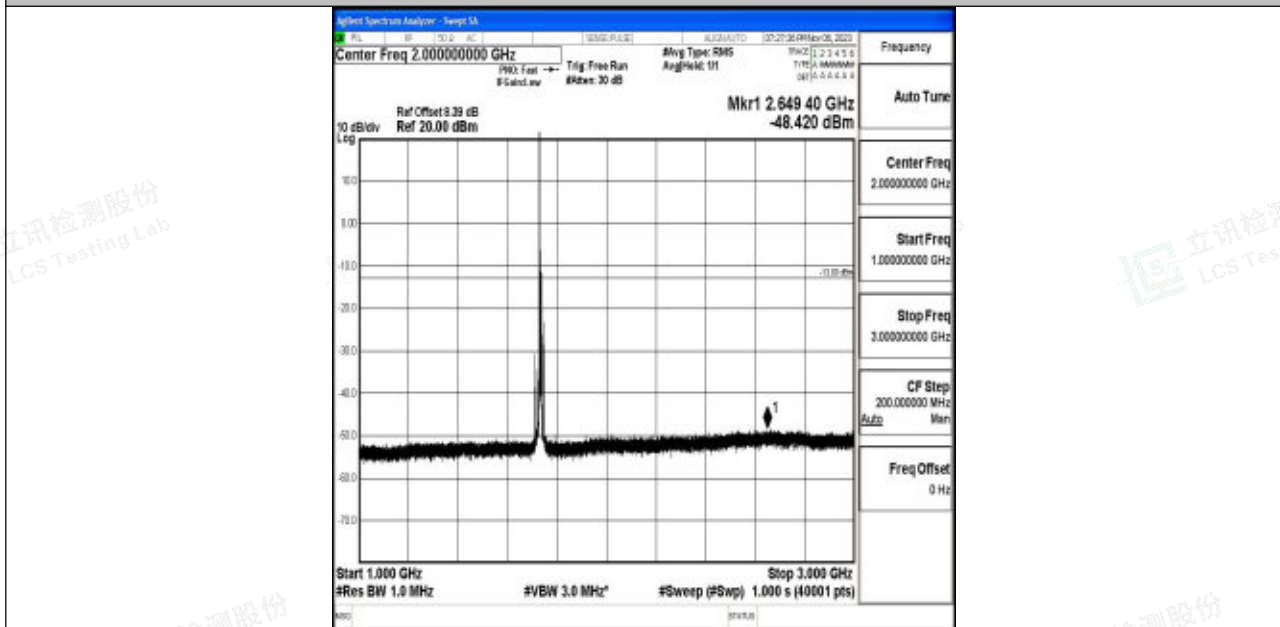
Band4_10MHz_16QAM_20175_1RB#0_1000~3000_1000~3000
