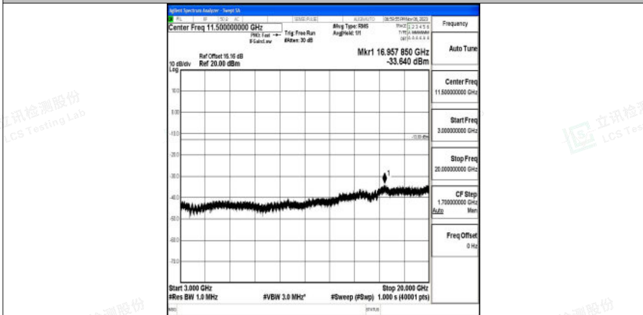
Band4_5MHz_16QAM_20175_1RB#0_3000~20000_3000~20000
