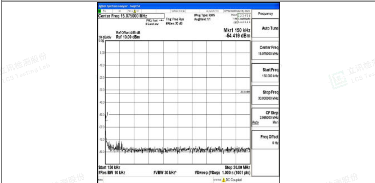
Band4_15MHz_64QAM_20175_1RB#0_0.15~30_0.15~30
