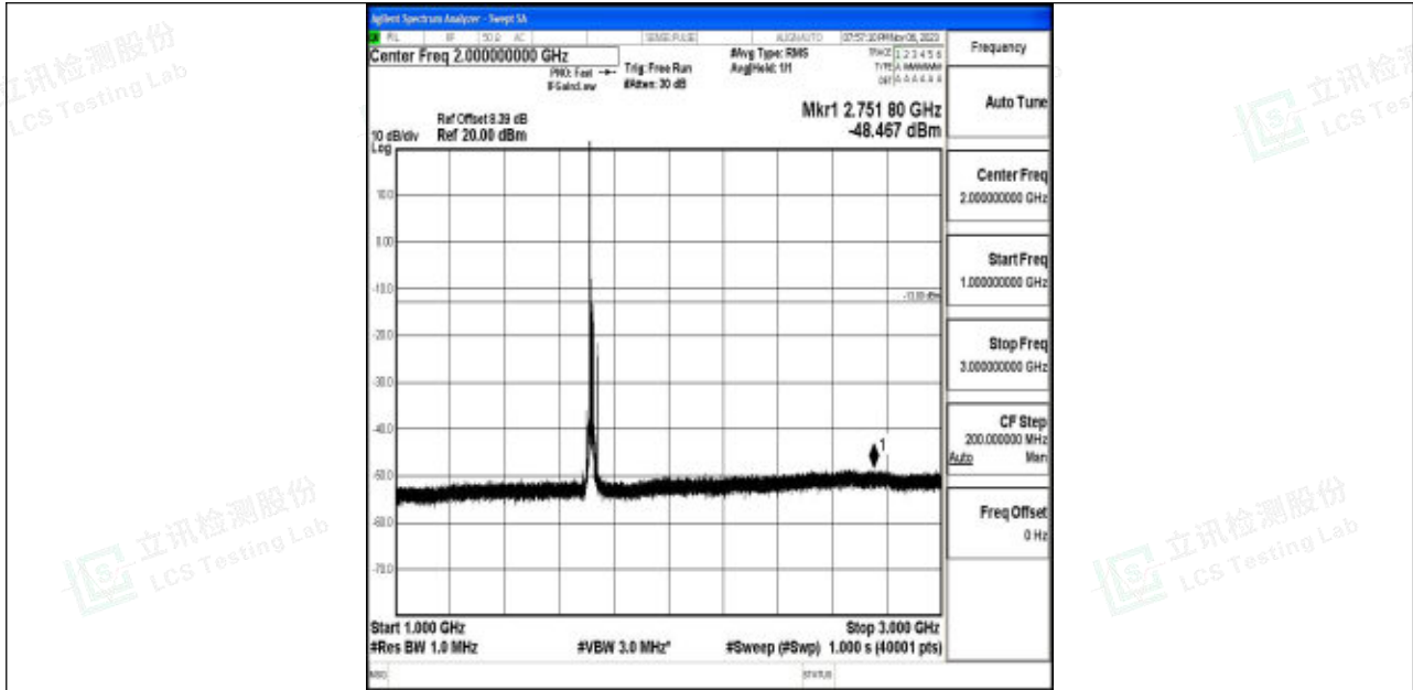
Band4_15MHz_64QAM_20025_1RB#0_1000~3000_1000~3000
