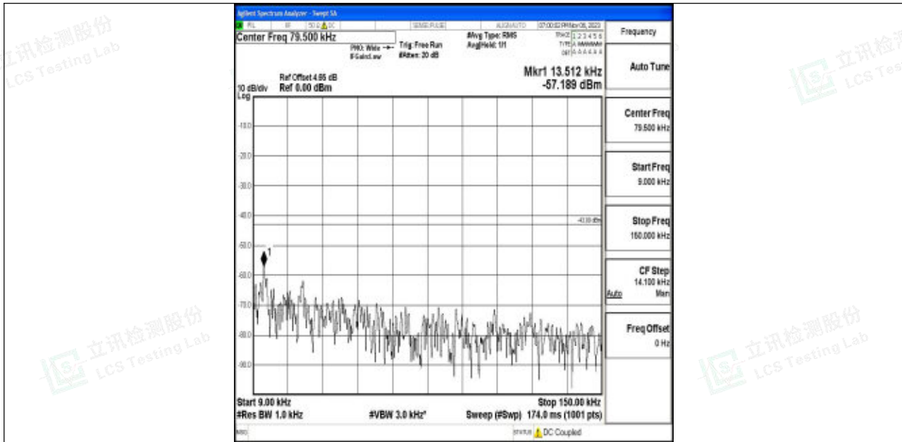
Band4_5MHz_64QAM_20175_1RB#0_0.009~0.15_0.009~0.15
