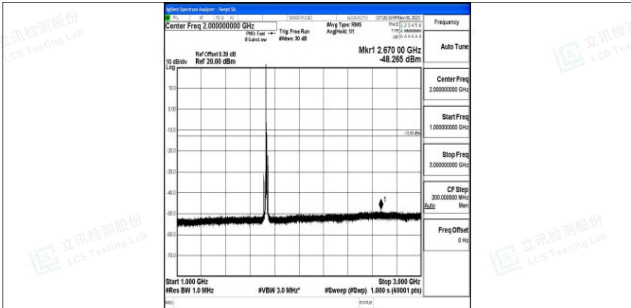
Band4_10MHz_64QAM_20175_1RB#0_1000~3000_1000~3000
