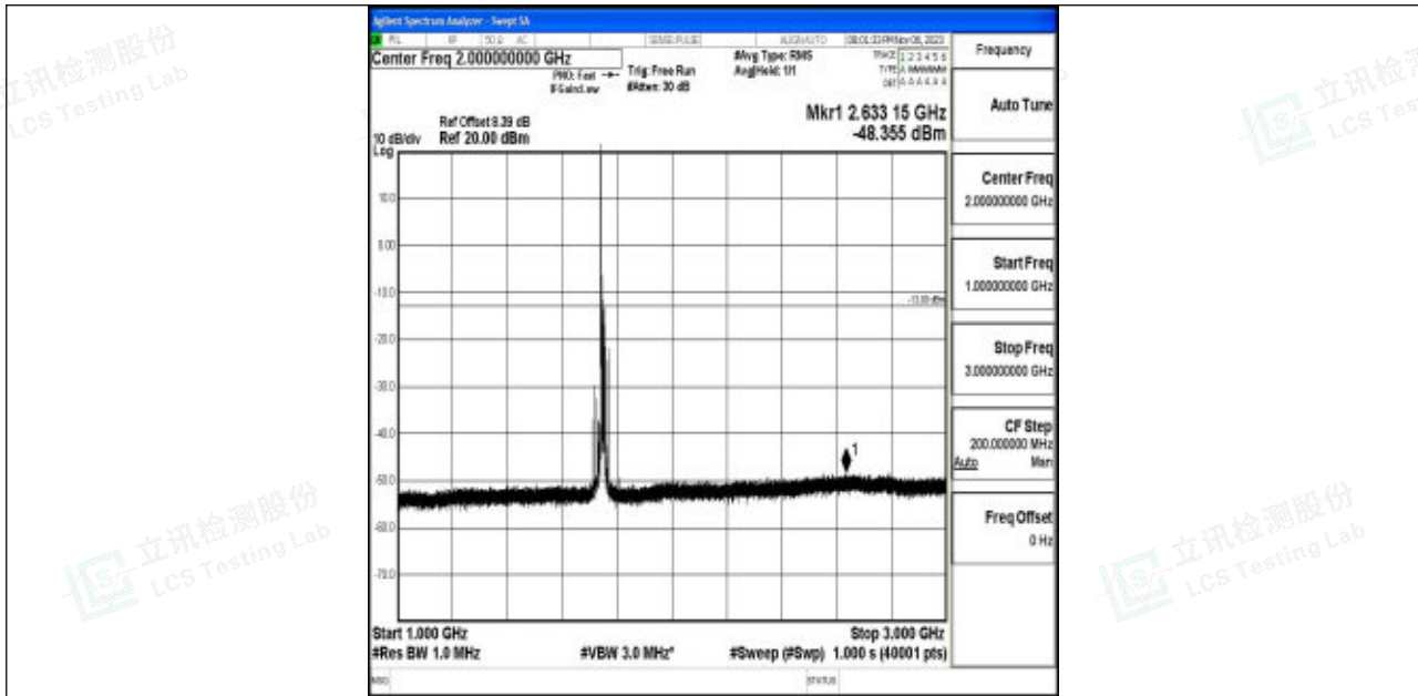
Band4_15MHz_64QAM_20325_1RB#0_1000~3000_1000~3000
