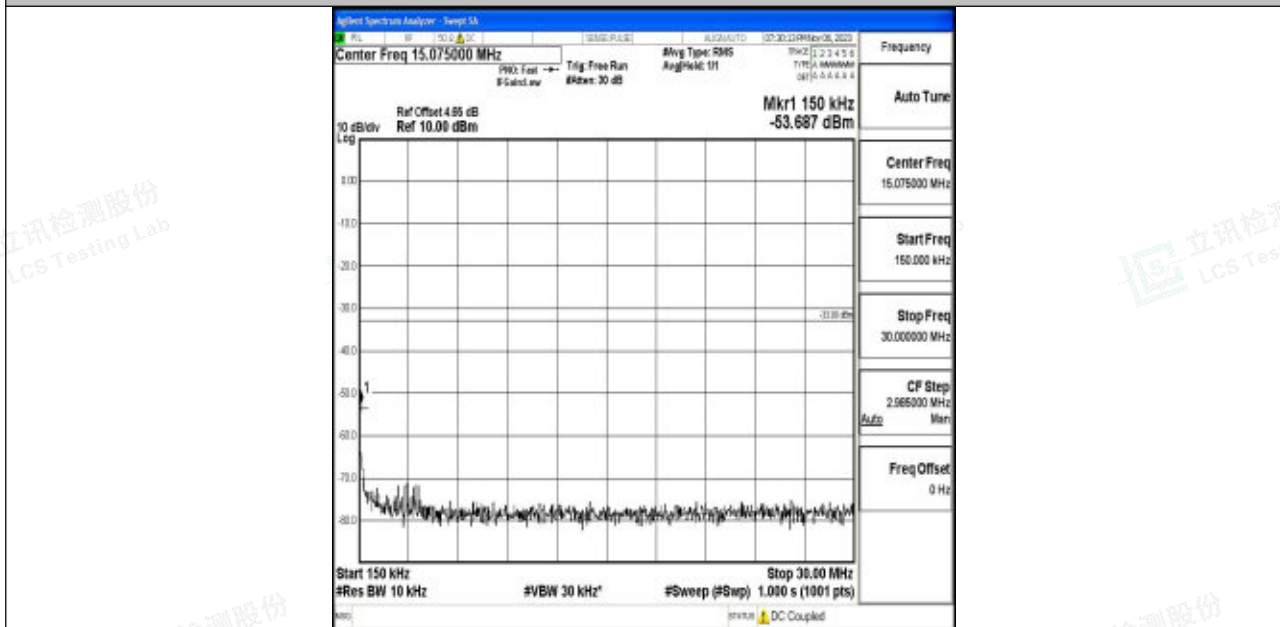
Band4_10MHz_64QAM_20350_1RB#0_0.15~30_0.15~30
