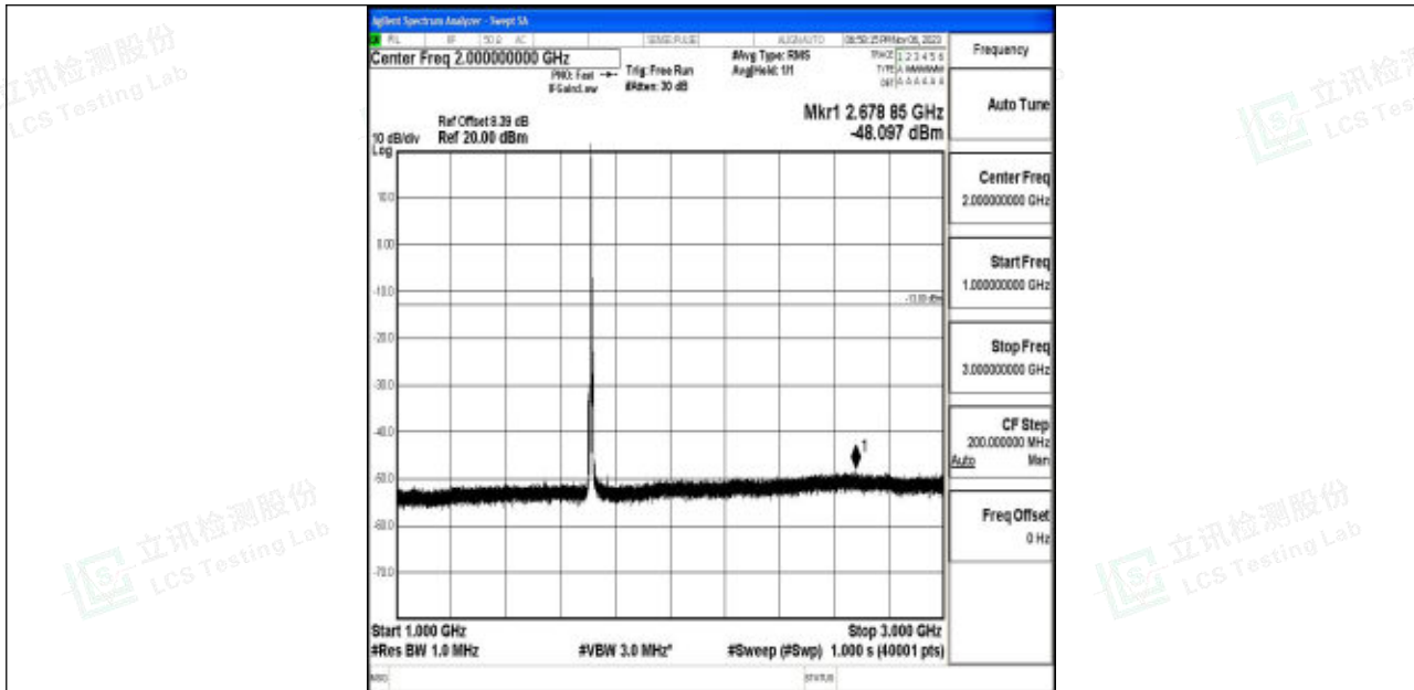
Band4_5MHz_64QAM_19975_1RB#0_1000~3000_1000~3000
