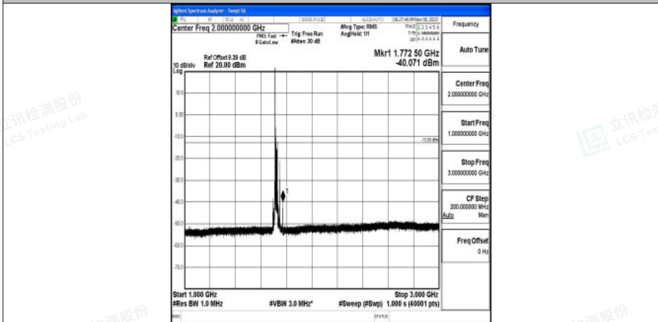
Band4_20MHz_64QAM_20050_1RB#0_1000~3000_1000~3000
