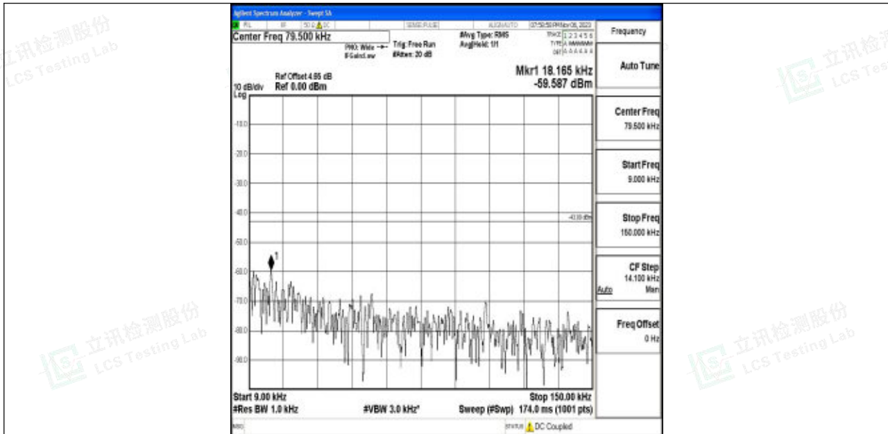
Band4_15MHz_64QAM_20175_1RB#0_0.009~0.15_0.009~0.15
