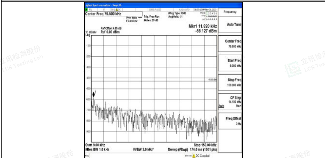
Band4_5MHz_16QAM_20175_1RB#0_0.009~0.15_0.009~0.15
