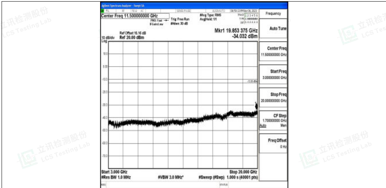
Band4_5MHz_QPSK_20175_1RB#0_3000~20000_3000~20000
