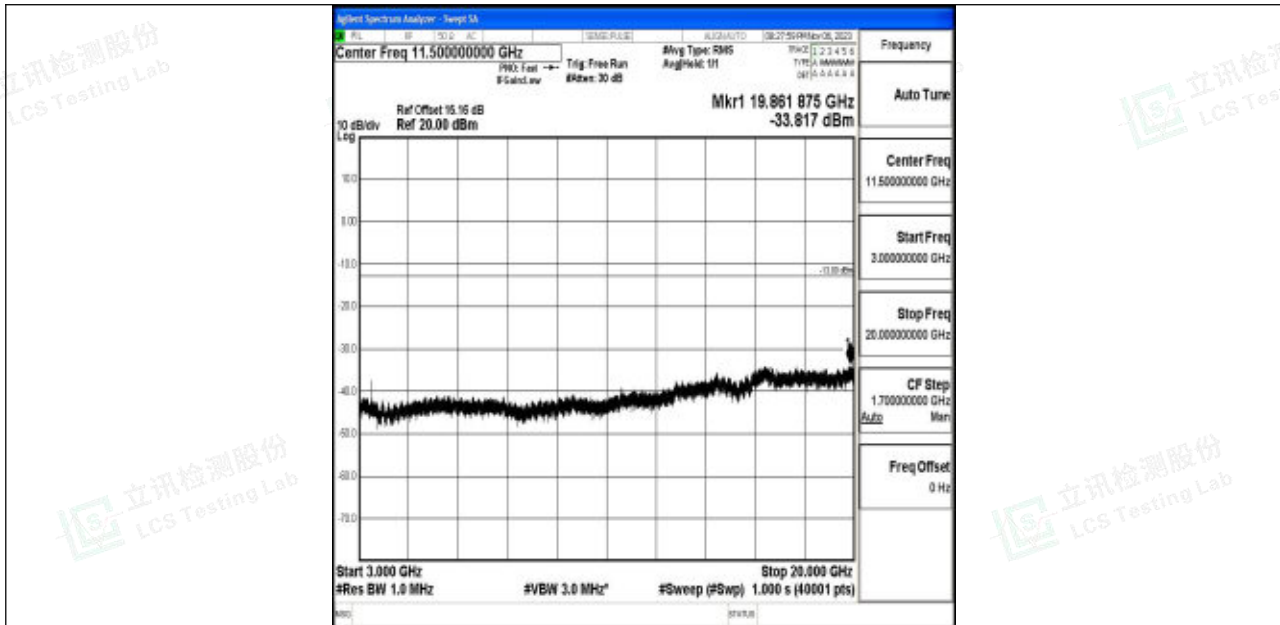
Band4_20MHz_64QAM_20050_1RB#0_3000~20000_3000~20000
