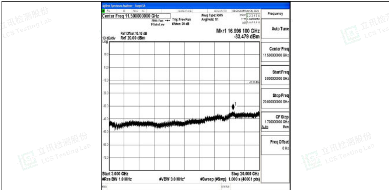
Band4_20MHz_16QAM_20175_1RB#0_3000~20000_3000~20000
