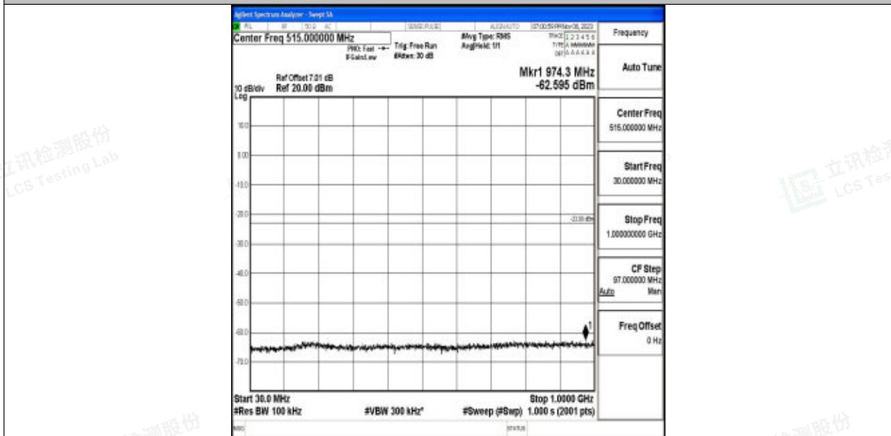
Band4_5MHz_QPSK_20375_1RB#0_30~1000_30~1000
