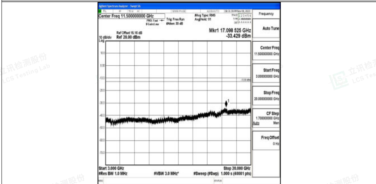
Band4_20MHz_16QAM_20300_1RB#0_3000~20000_3000~20000
