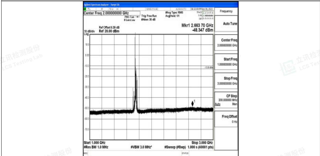
Band4_20MHz_64QAM_20300_1RB#0_1000~3000_1000~3000
