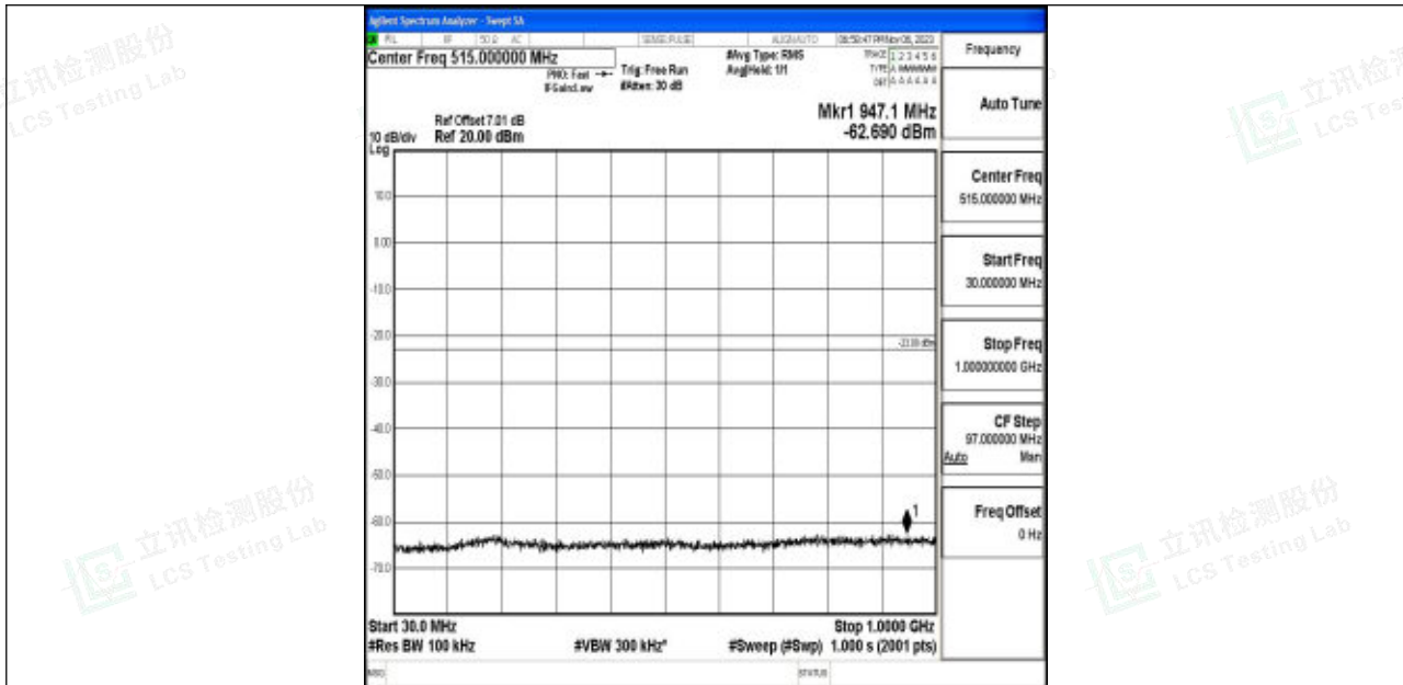
Band4_5MHz_QPSK_20175_1RB#0_30~1000_30~1000
