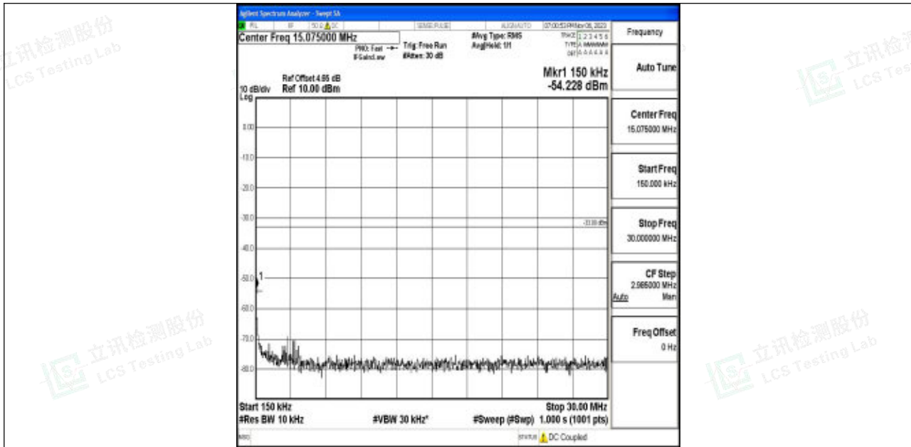
Band4_5MHz_QPSK_20375_1RB#0_0.15~30_0.15~30
