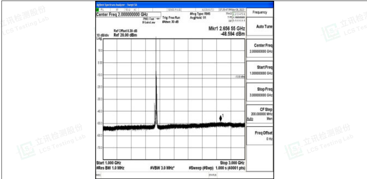
Band4_10MHz_16QAM_20350_1RB#0_1000~3000_1000~3000
