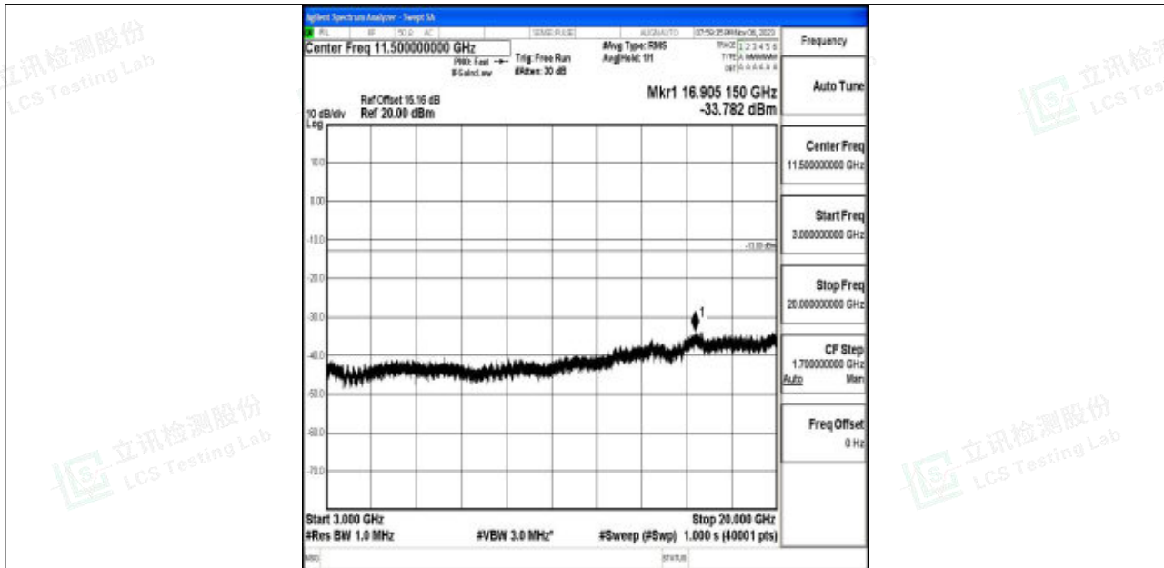
Band4_15MHz_64QAM_20175_1RB#0_3000~20000_3000~20000
