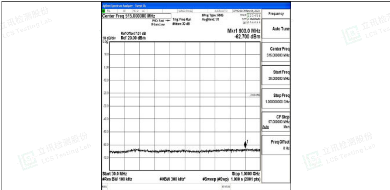
Band4_15MHz_64QAM_20175_1RB#0_30~1000_30~1000
