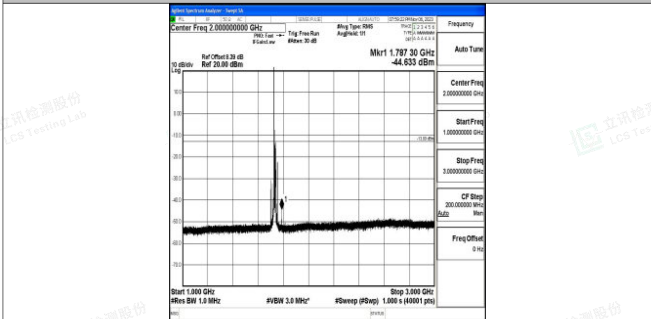
Band4_15MHz_64QAM_20175_1RB#0_1000~3000_1000~3000
