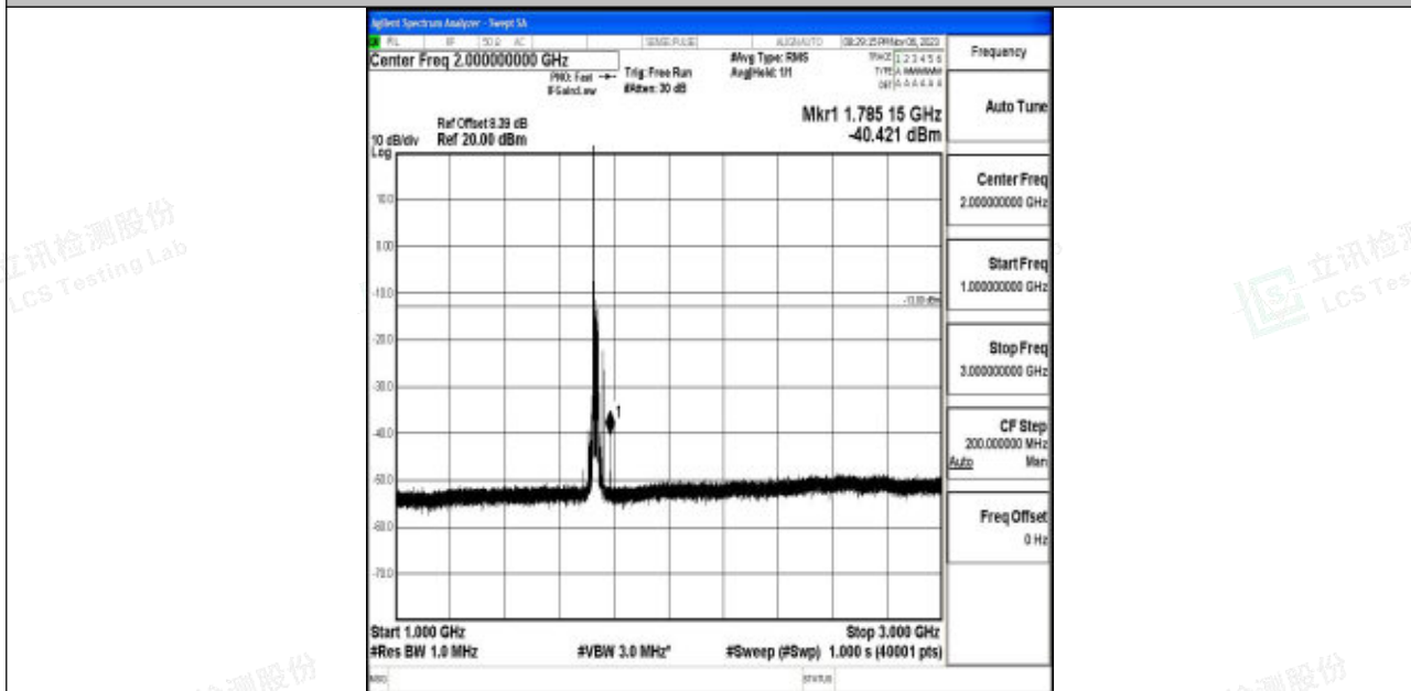
Band4_20MHz_16QAM_20175_1RB#0_1000~3000_1000~3000
