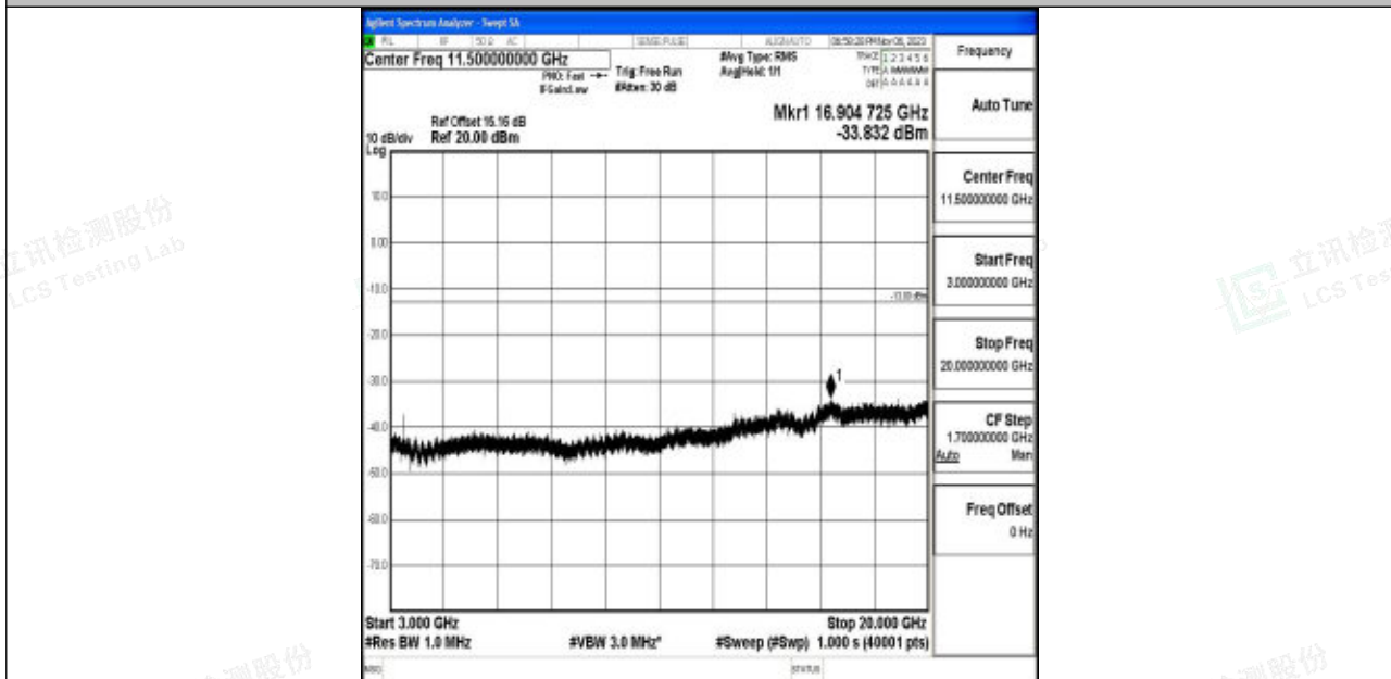
Band4_5MHz_64QAM_19975_1RB#0_3000~20000_3000~20000
