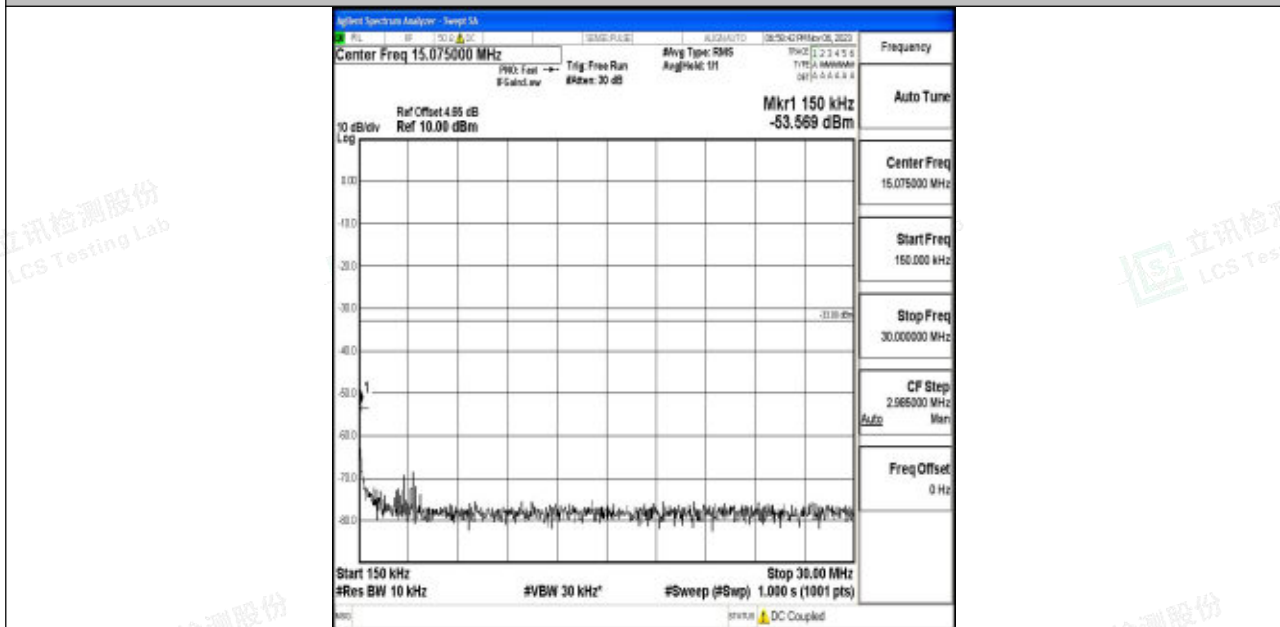
Band4_5MHz_QPSK_20175_1RB#0_0.15~30_0.15~30
