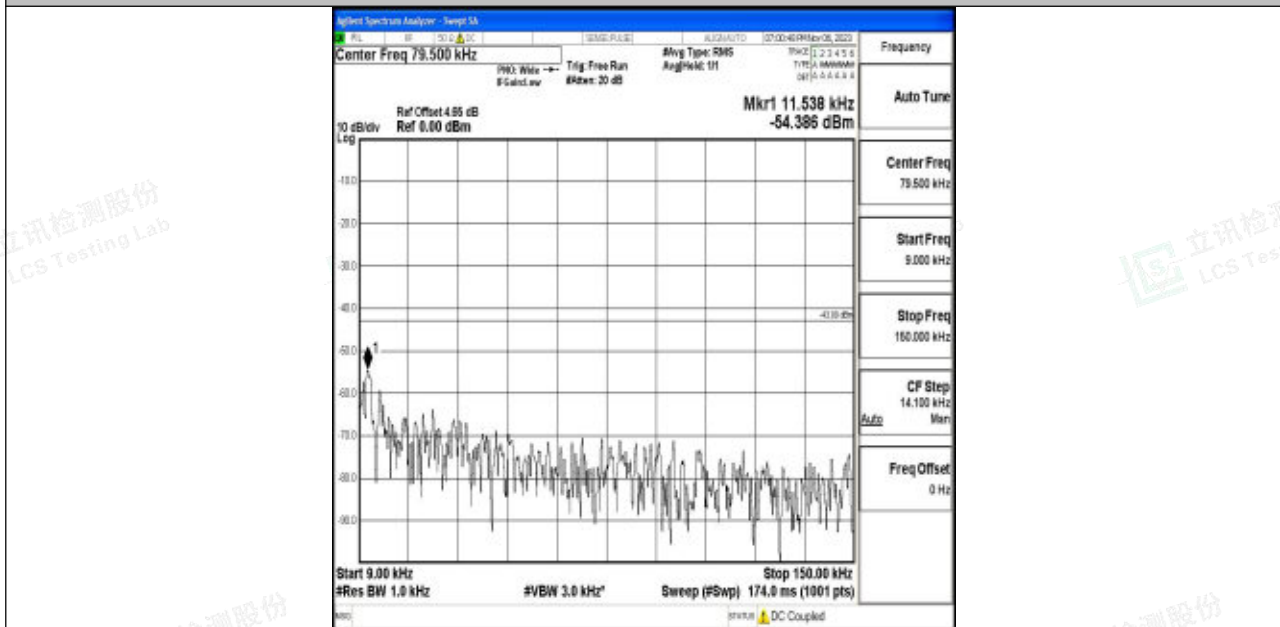
Band4_5MHz_QPSK_20375_1RB#0_0.009~0.15_0.009~0.15
