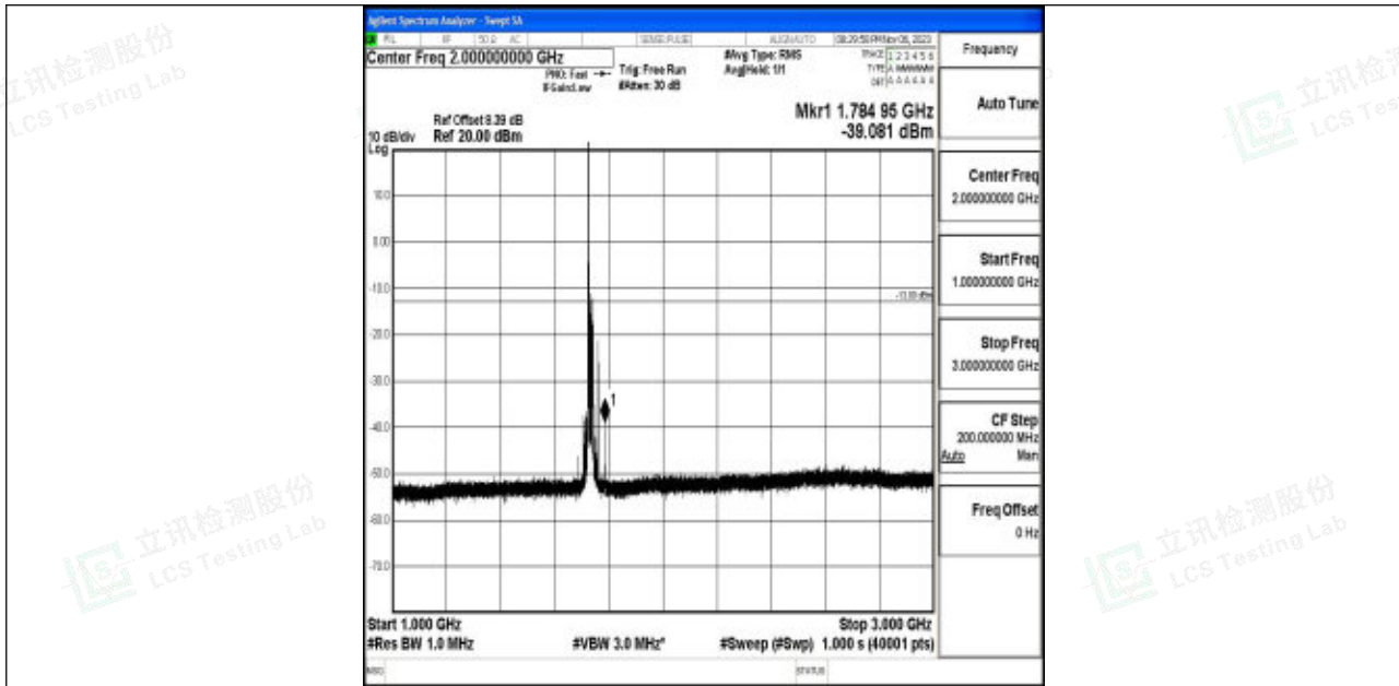
Band4_20MHz_64QAM_20175_1RB#0_1000~3000_1000~3000
