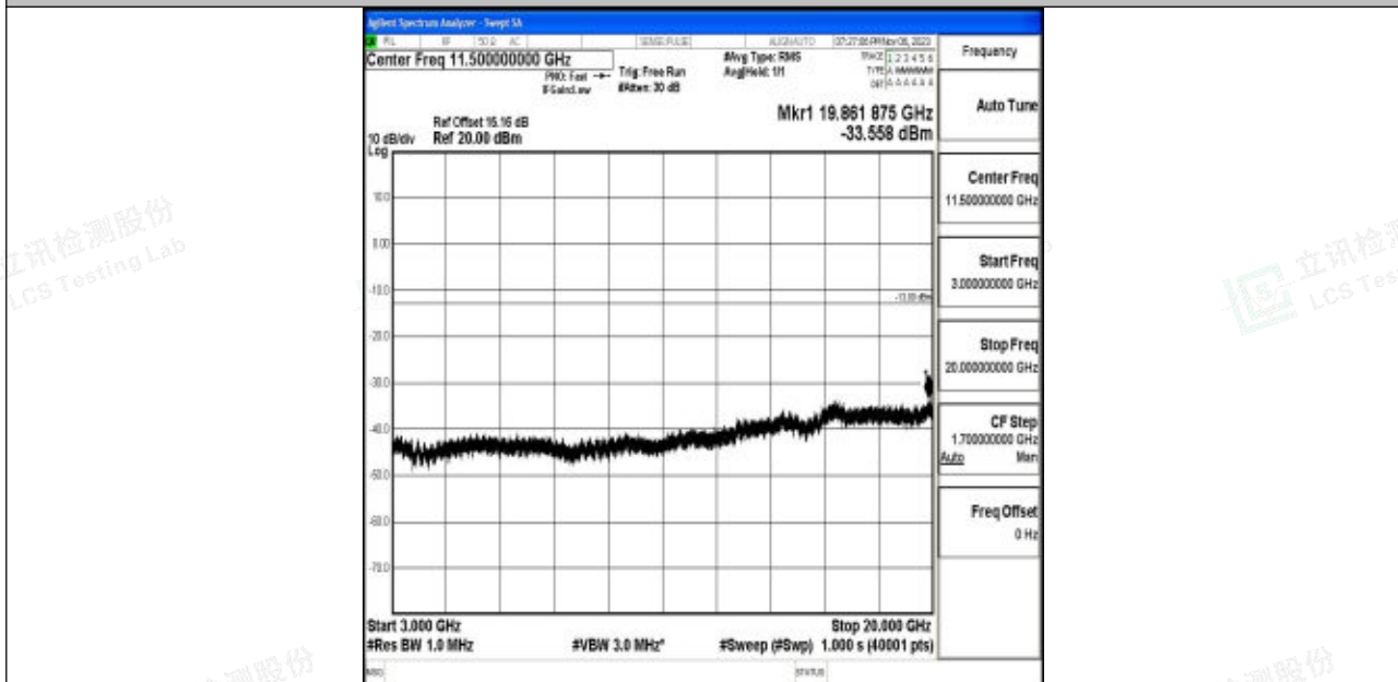
Band4_10MHz_QPSK_20175_1RB#0_3000~20000_3000~20000
