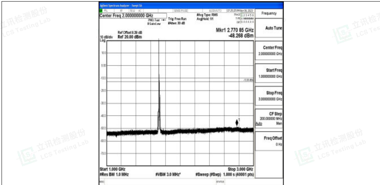
Band4_10MHz_16QAM_20000_1RB#0_1000~3000_1000~3000
