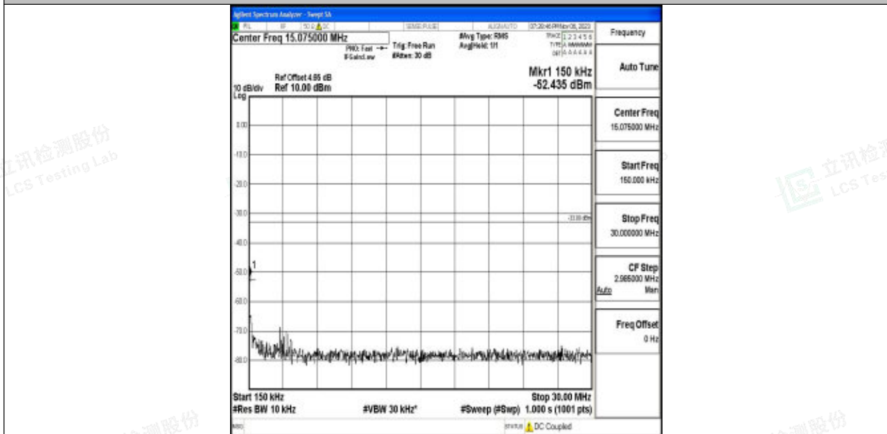
Band4_10MHz_QPSK_20350_1RB#0_0.15~30_0.15~30
