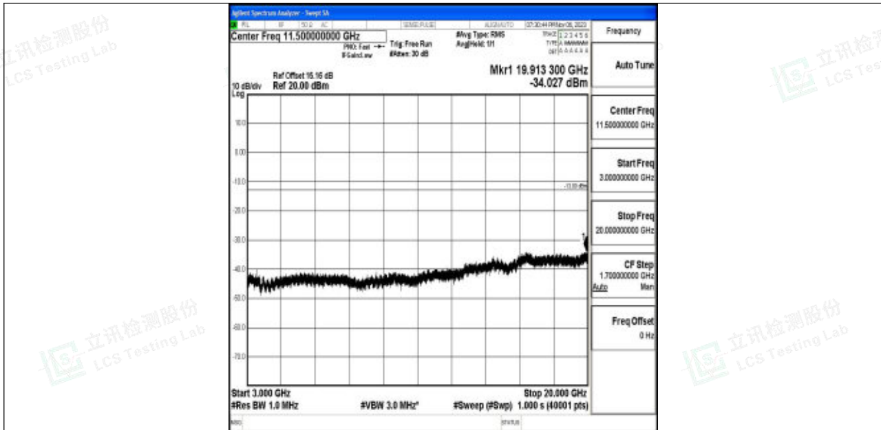
Band4_10MHz_64QAM_20350_1RB#0_3000~20000_3000~20000
