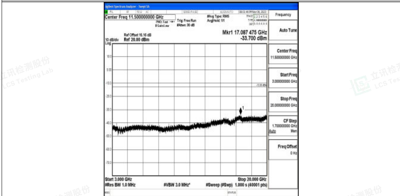
Band4_15MHz_64QAM_20325_1RB#0_3000~20000_3000~20000
