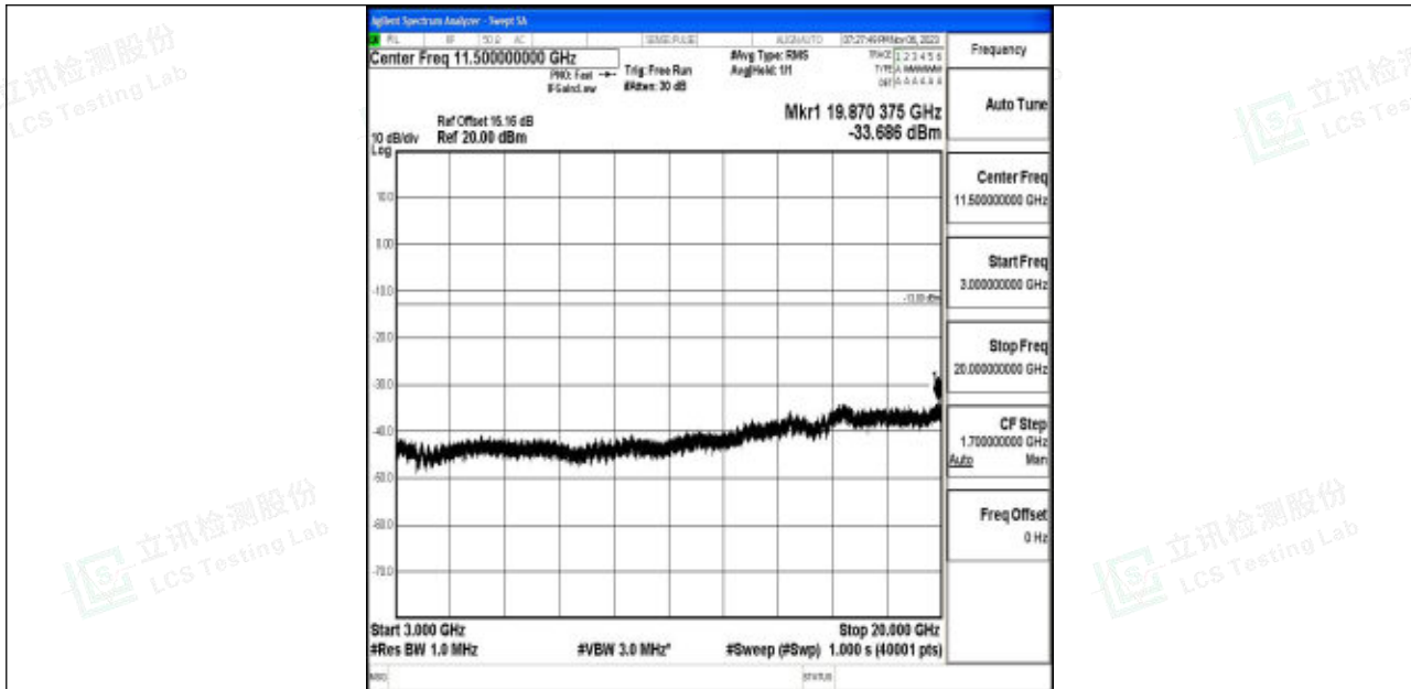
Band4_10MHz_16QAM_20175_1RB#0_3000~20000_3000~20000
