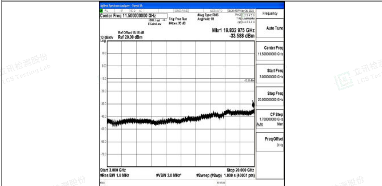
Band4_20MHz_QPSK_20175_1RB#0_3000~20000_3000~20000
