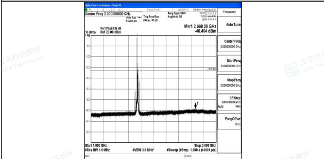
Band4_20MHz_QPSK_20300_1RB#0_1000~3000_1000~3000
