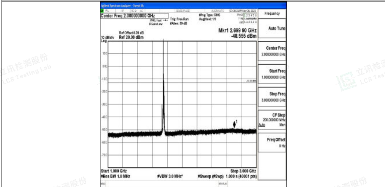
Band4_10MHz_64QAM_20350_1RB#0_1000~3000_1000~3000
