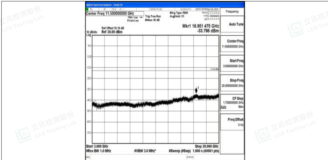
Band4_5MHz_16QAM_19975_1RB#0_3000~20000_3000~20000
