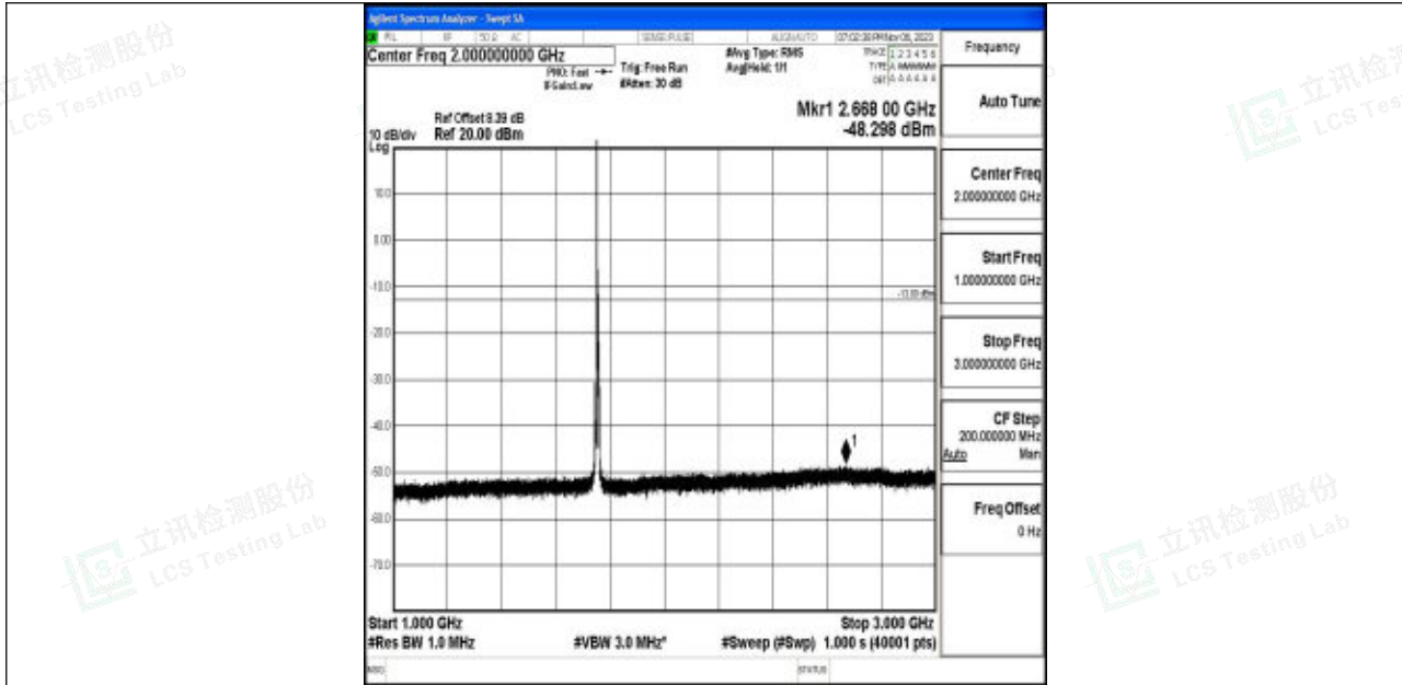
Band4_5MHz_64QAM_20375_1RB#0_1000~3000_1000~3000
