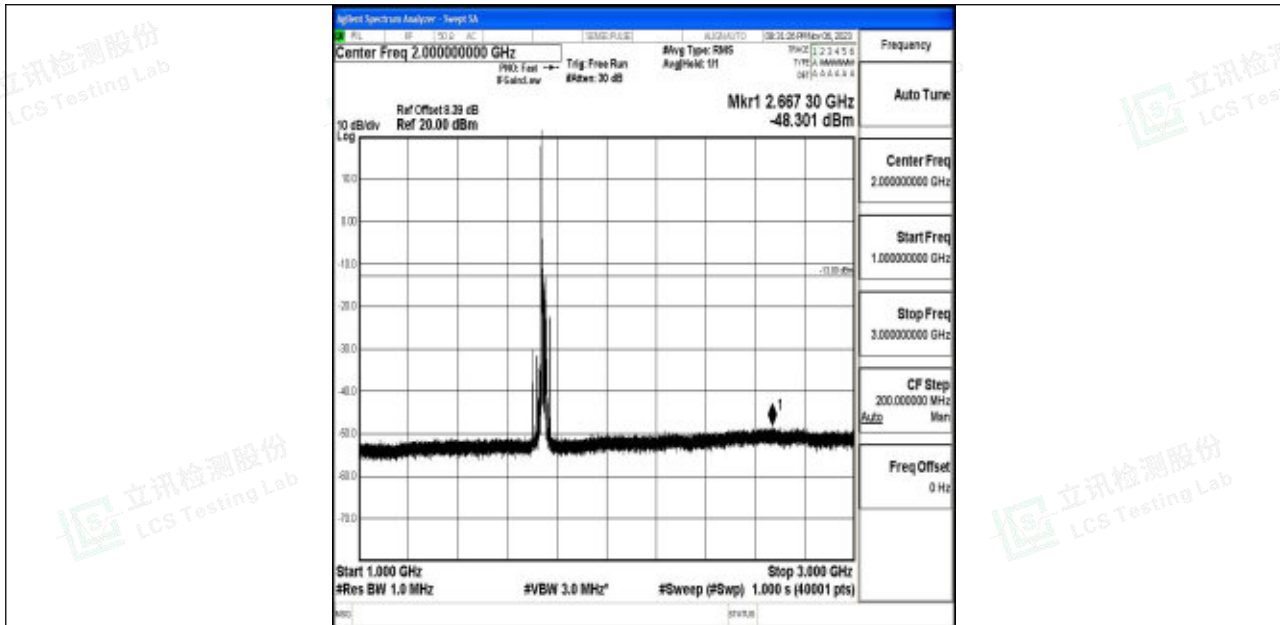
Band4_20MHz_16QAM_20300_1RB#0_1000~3000_1000~3000
