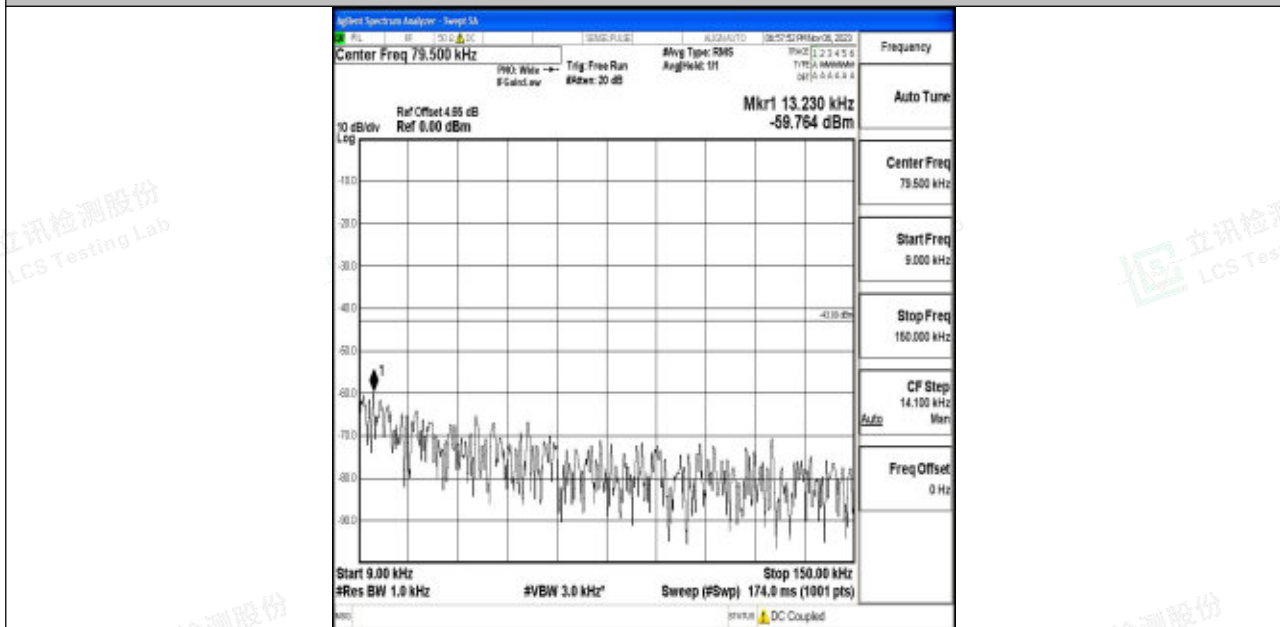
Band4_5MHz_64QAM_19975_1RB#0_0.009~0.15_0.009~0.15
