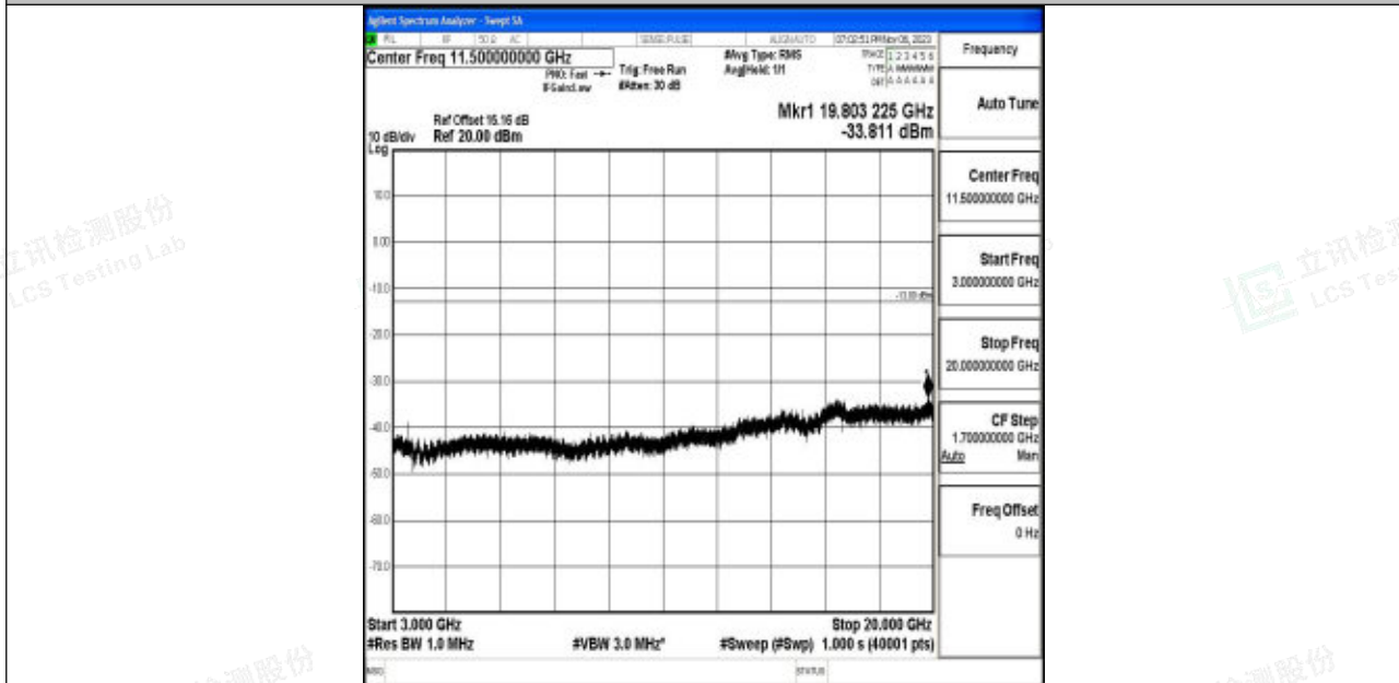
Band4_5MHz_64QAM_20375_1RB#0_3000~20000_3000~20000
