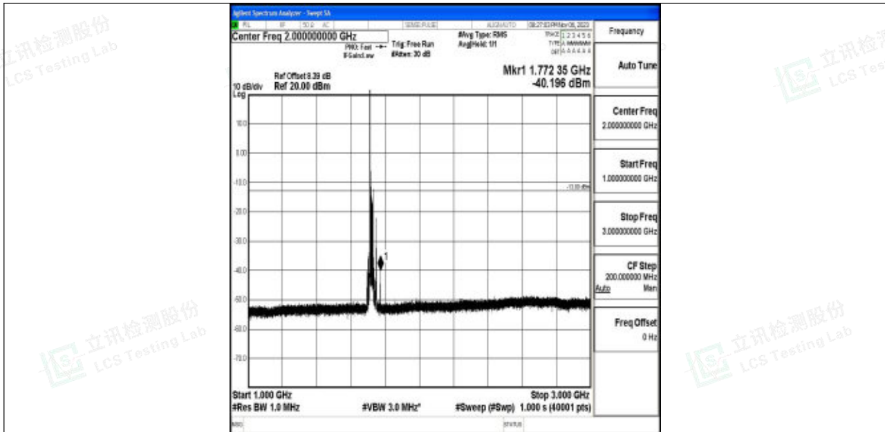
Band4_20MHz_16QAM_20050_1RB#0_1000~3000_1000~3000
