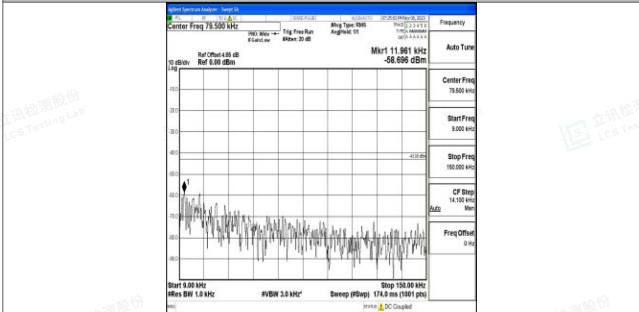
Band4_10MHz_16QAM_20000_1RB#0_0.009~0.15_0.009~0.15
