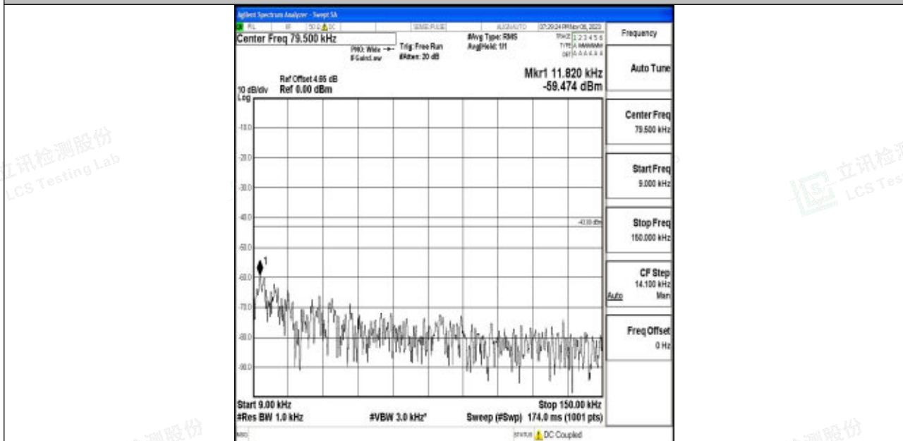
Band4_10MHz_16QAM_20350_1RB#0_0.009~0.15_0.009~0.15
