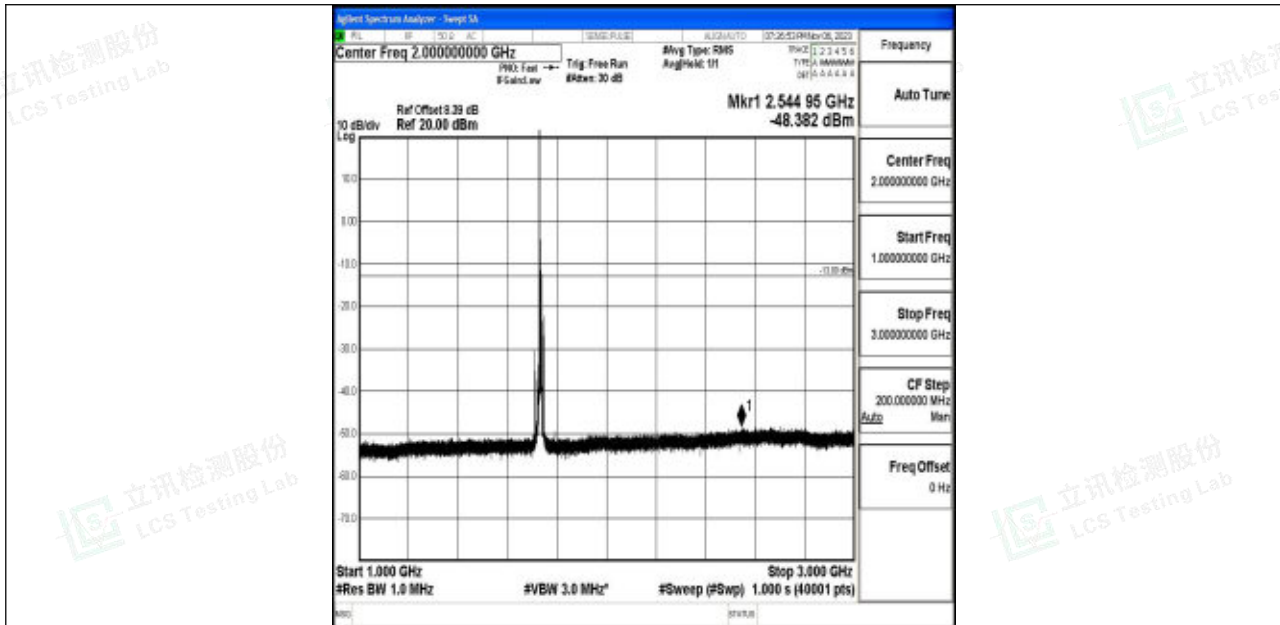
Band4_10MHz_QPSK_20175_1RB#0_1000~3000_1000~3000
