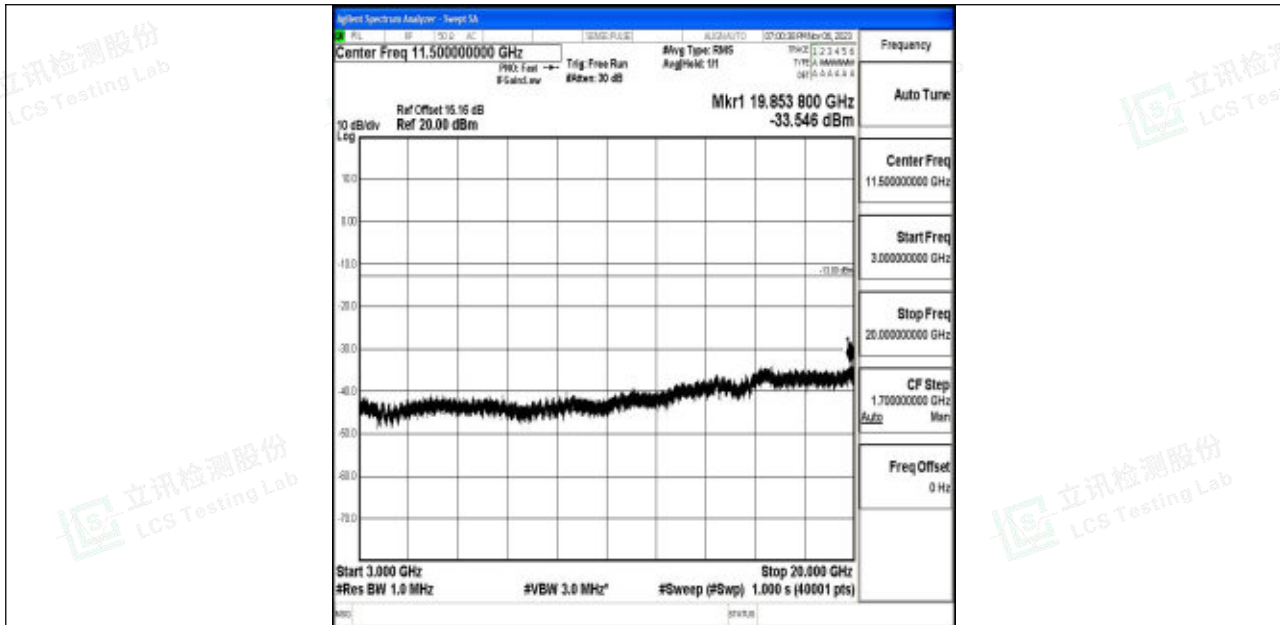
Band4_5MHz_64QAM_20175_1RB#0_3000~20000_3000~20000
