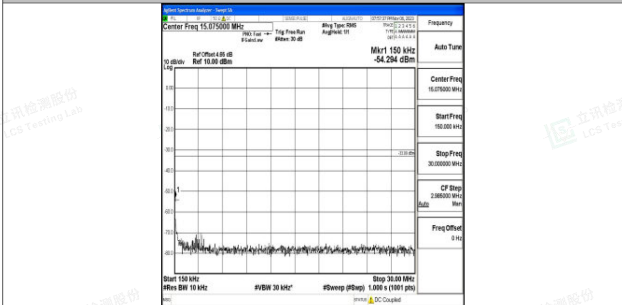
Band4_15MHz_QPSK_20175_1RB#0_0.15~30_0.15~30
