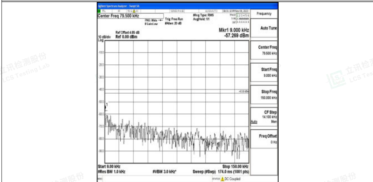
Band4_15MHz_64QAM_20325_1RB#0_0.009~0.15_0.009~0.15
