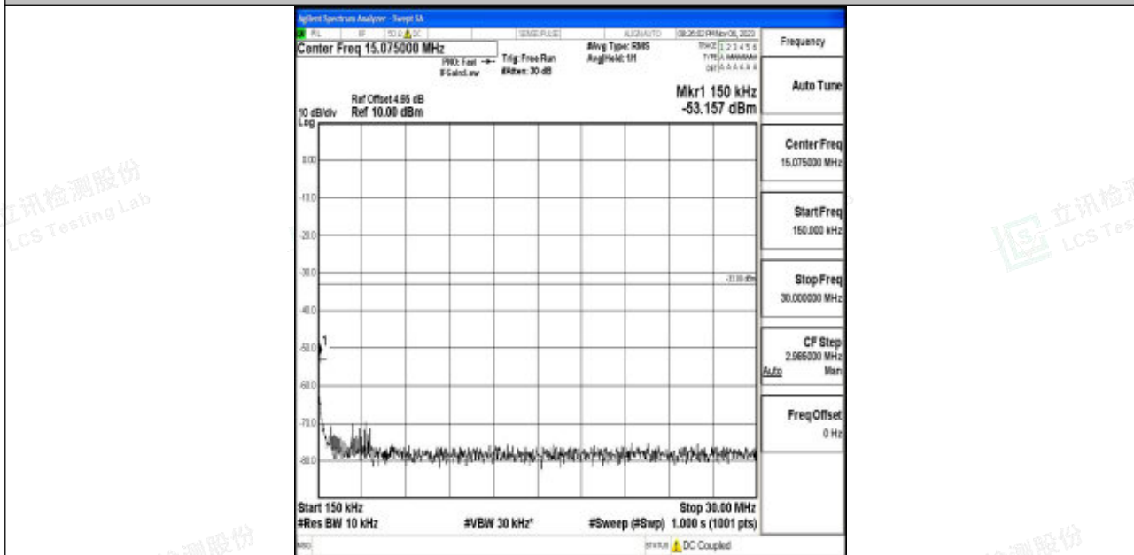
Band4_20MHz_QPSK_20050_1RB#0_0.15~30_0.15~30
