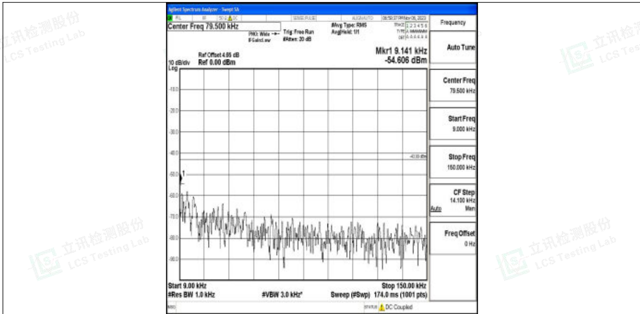
Band4_5MHz_QPSK_20175_1RB#0_0.009~0.15_0.009~0.15
