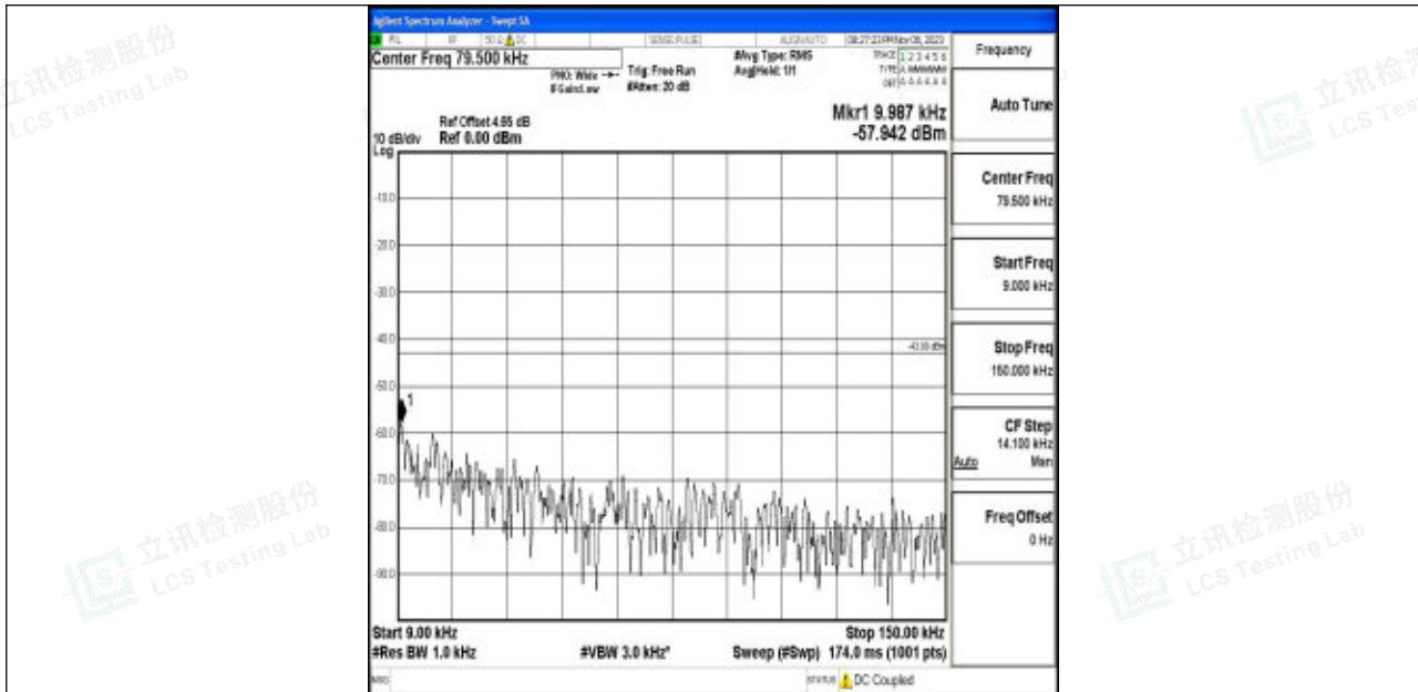
Band4_20MHz_64QAM_20050_1RB#0_0.009~0.15_0.009~0.15
