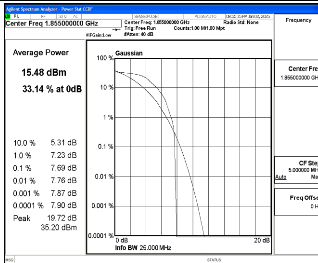
Band25-10MHz-QPSK-26090-1-0-Low-7.69-13-PASS
