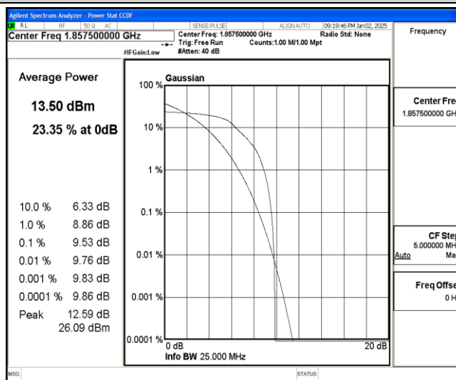
Band25-15MHz-QPSK-26115-6-0-Low-9.53-&lt;=13-PASS
