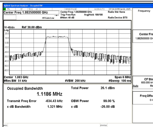
Band25-3MHz-16QAM-26365-6-0-Low-1.1186-1.321-PASS
