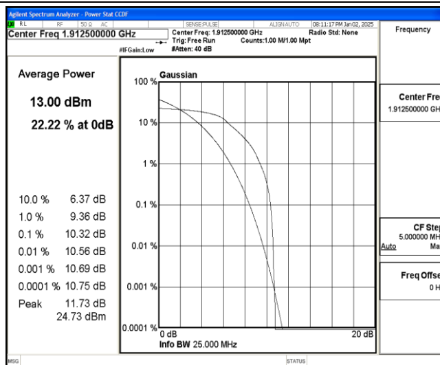
Band25-5MHz-16QAM-26665-6-0-High-10.32-13-PASS
