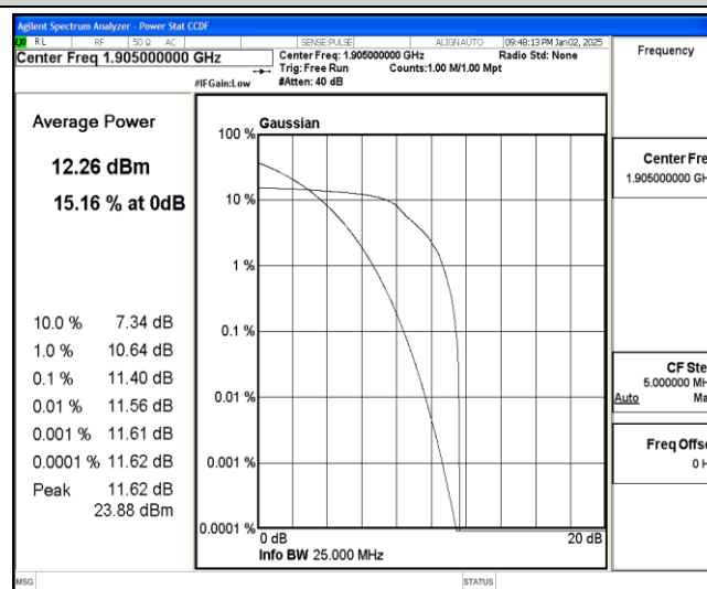
Band25-20MHz-QPSK-26590-1-0-High-11.40-&lt;=13-PASS
