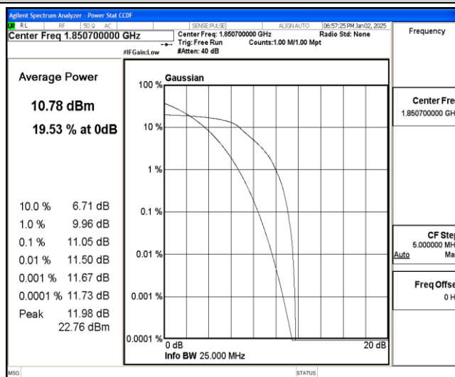
Band25-1.4MHz-QPSK-26047-6-0-Low-11.05-13-PASS
