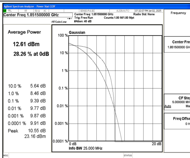
Band25-3MHz-16QAM-26055-6-0-Low-9.39-&lt;=13-PASS
