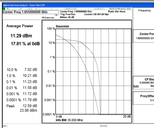
Band25-10MHz-QPSK-26090-6-0-Low-11.23-13-PASS
