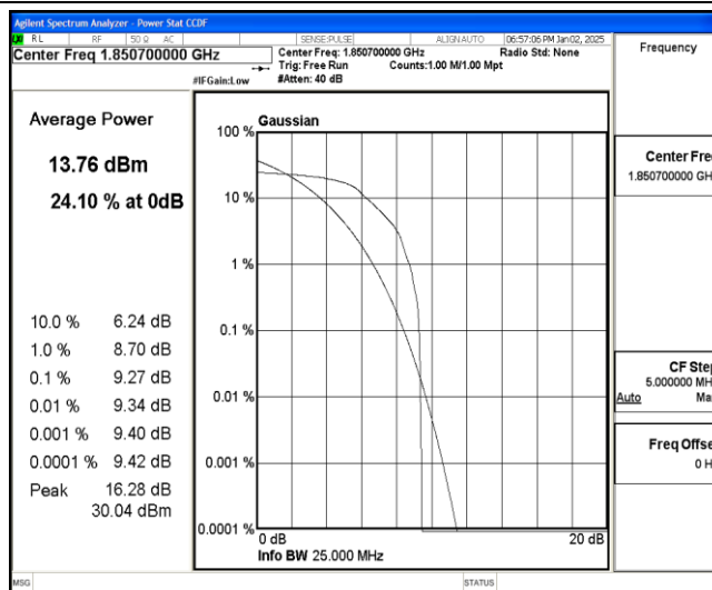
Band25-1.4MHz-QPSK-26047-1-0-Low-9.27-13-PASS
