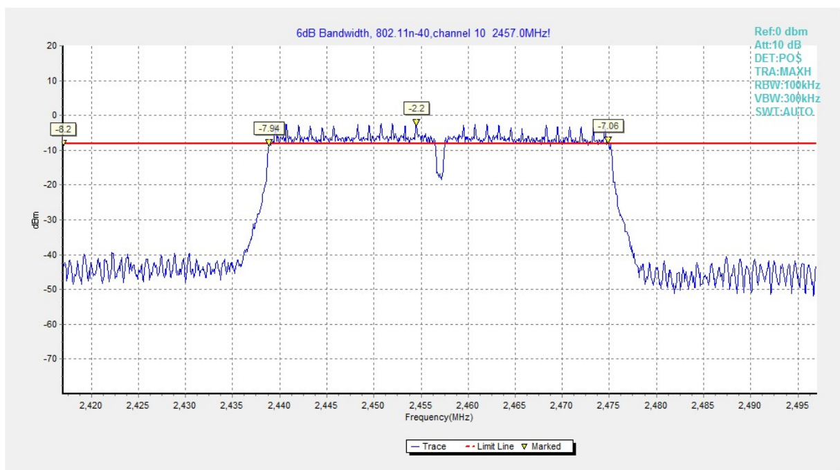
Fig.A.4.19 Occupied 6dB Bandwidth (802.11 n-HT40, Ch 10)
