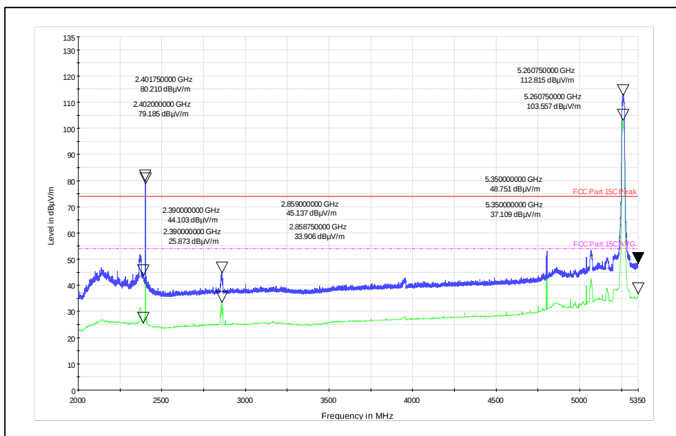
Horizontal Polarization
