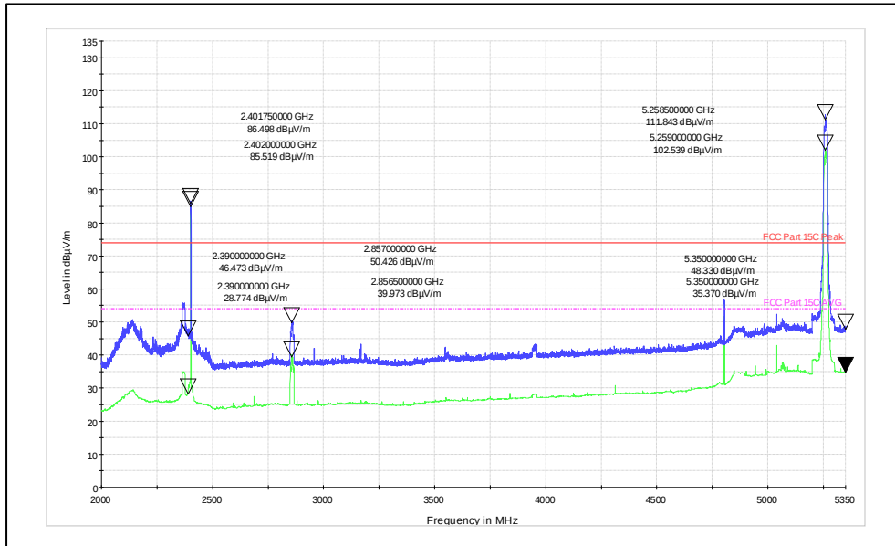
Vertical Polarization
