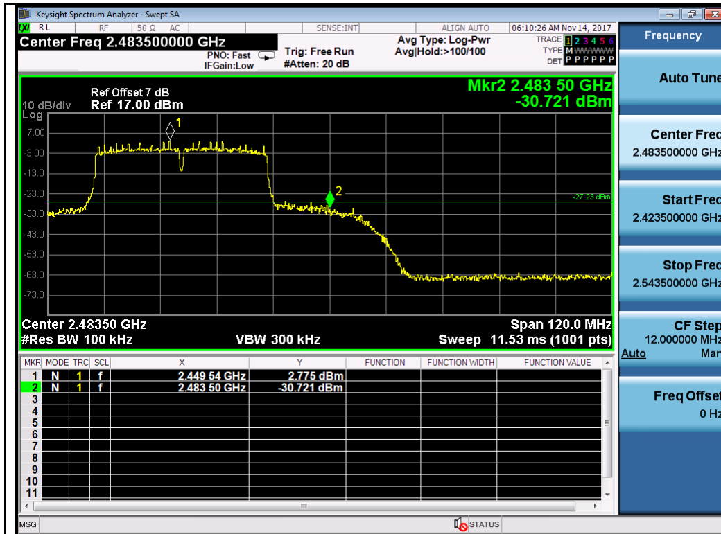
802.11n-HT40-2452MHz Chain 0
