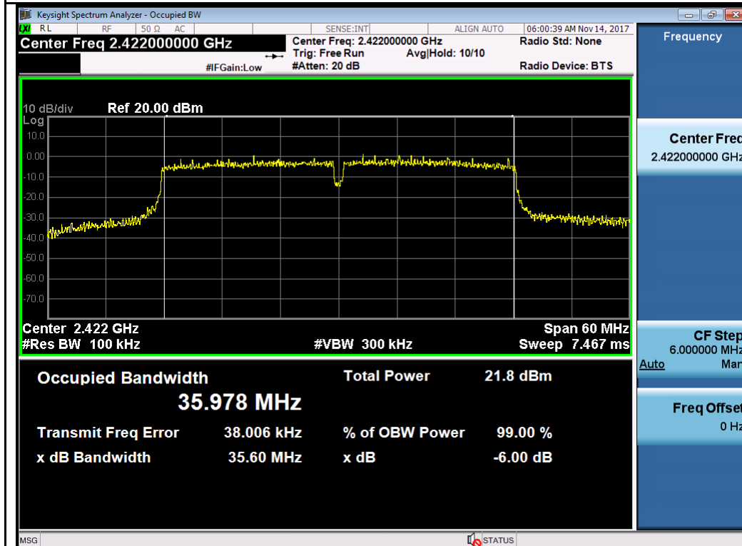
802.11n-HT40-2422MHz
