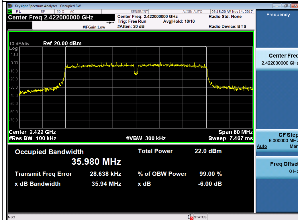
802.11n-HT40-2422MHz
