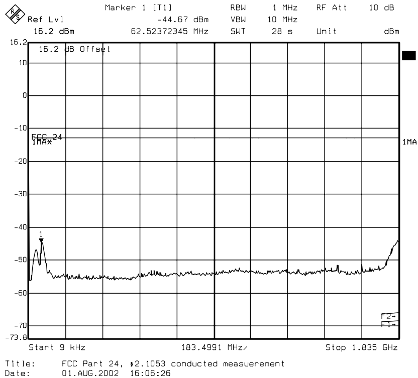
diagram 14.01: carrier on channel 512 (1850,2 MHz)
