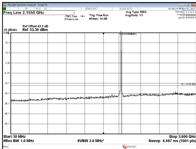
Figure 8.2-323: Conducted spurious emissions within 30–3600 MHz, Port C, WCDMA, 2 top channels, QPSK
