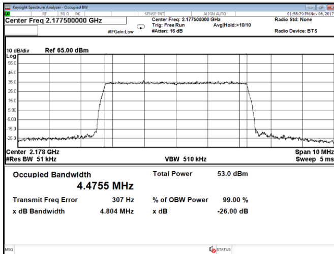
Figure 8.5-3: Occupied bandwidth, QPSK, LTE, 5 MHz, Port A, high channel
