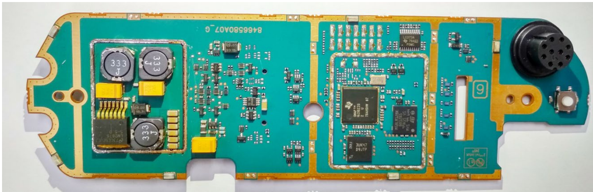
MTM5200 / MTM5400 / MTM5500 Enhanced Control Head
