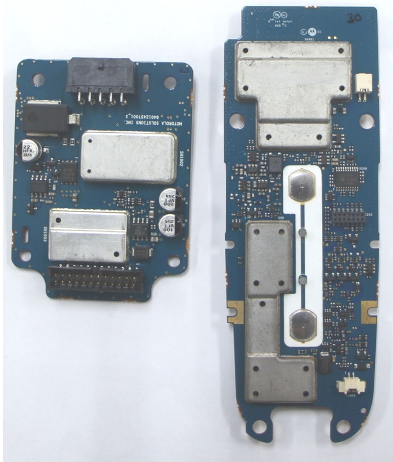
MTM5500 Telephone Style Control Head
