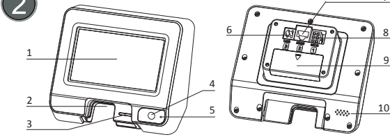
Figure 1: front view 1. LCD & Touchscreen 2. Smart Card & Magnetic Strip Card Reader 3. Status Indicator Light 4. Camera 5. Camera Indicator Light Figure 2: back view 6. Type-B 7. RS232 8. MDB Port 9. SAM Card Cover 10. Speaker
