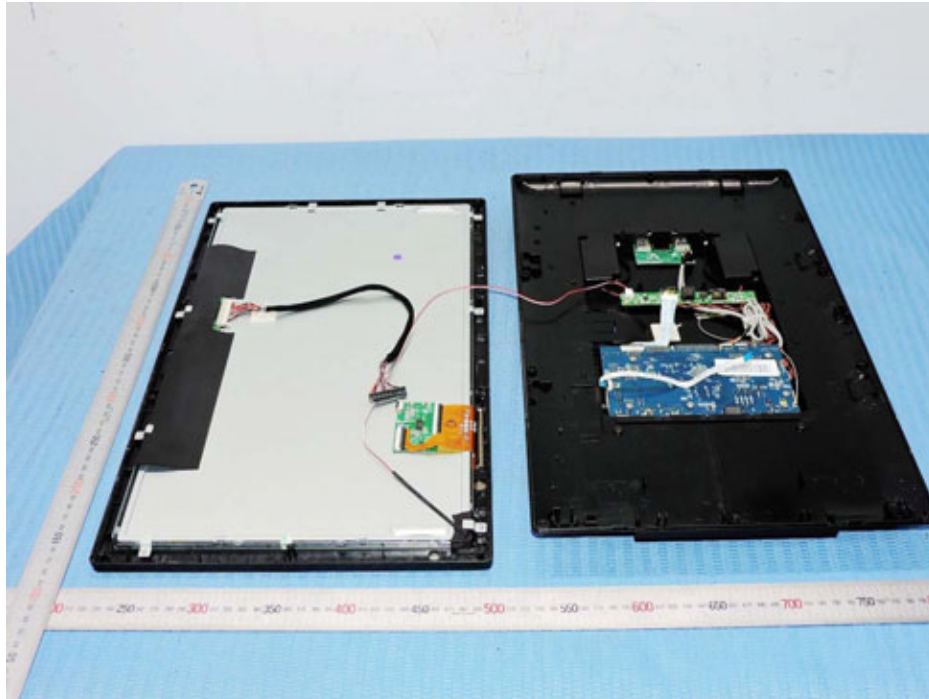
Photos of EUT Model No: JAR185
