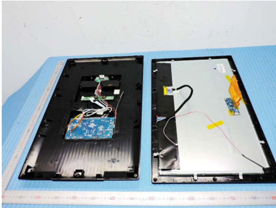
Photos of EUT Model No: JAR215
