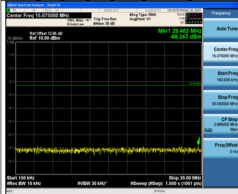
Band26_3MHz_16QAM_26705_15RB#0_0.15~30_0.15~30
