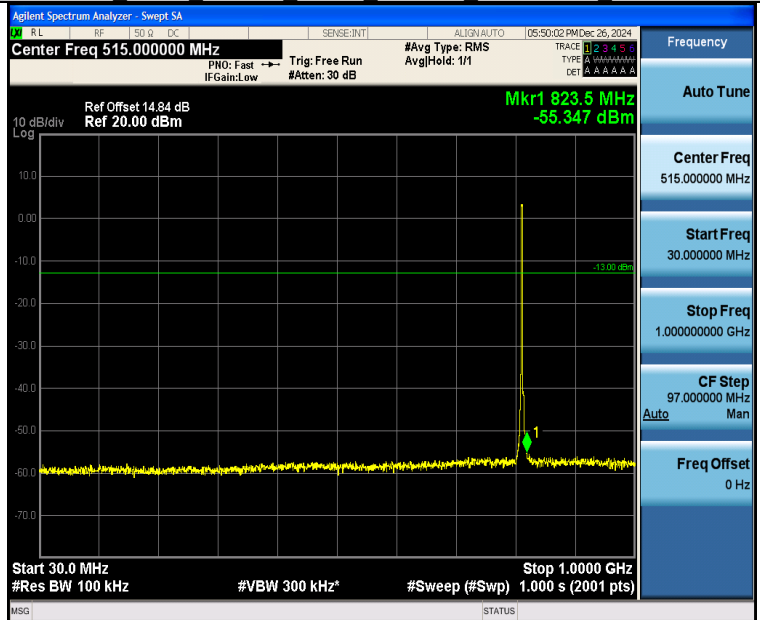
Band26_3MHz_16QAM_26705_15RB#0_30~1000_30~1000
