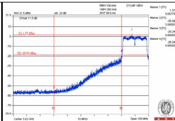
802.11ac (VHT20) MODULATION (CH 132: 5660MHz)
