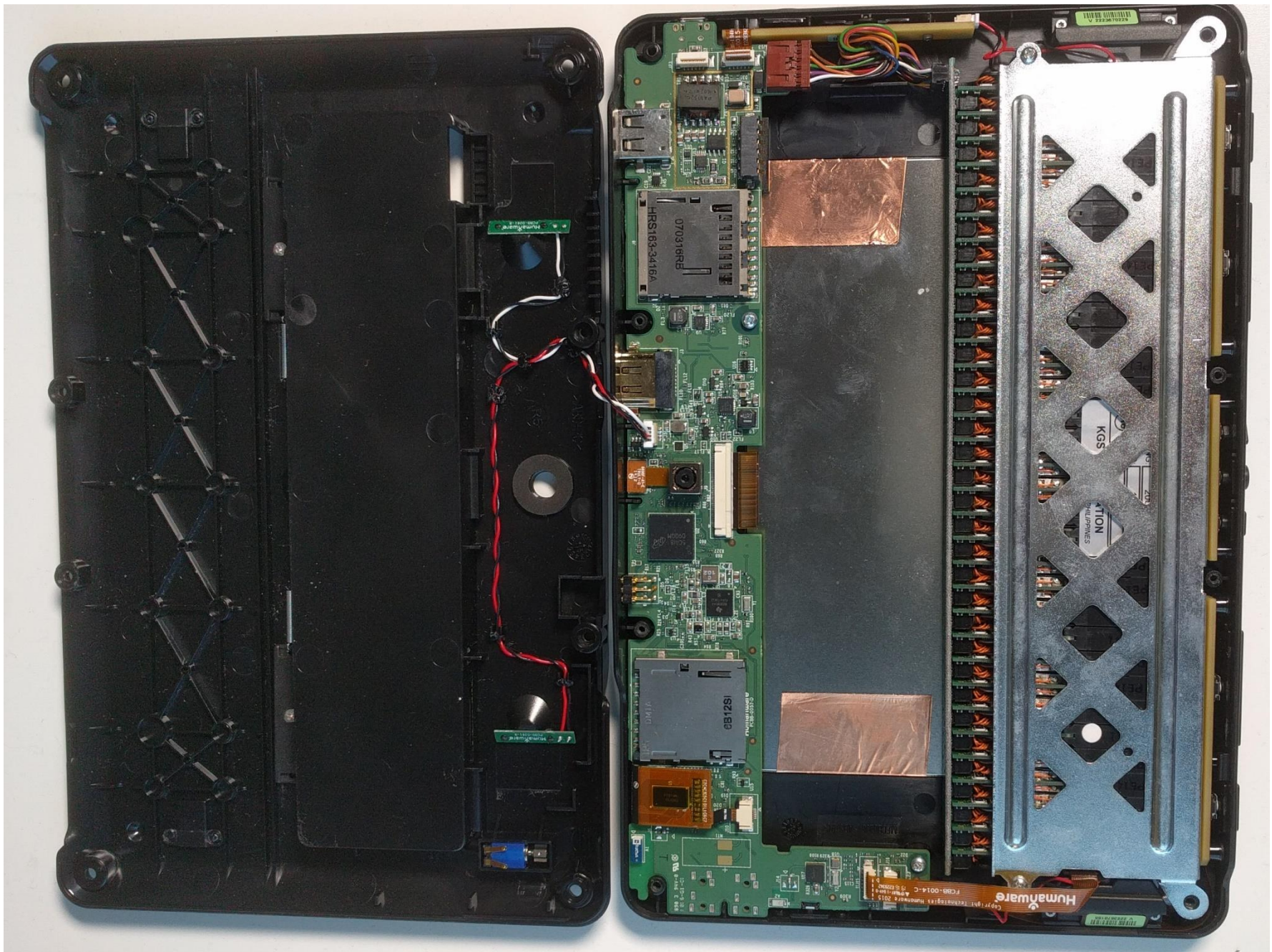
Internal photo full enclosure
