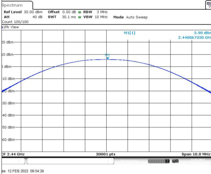
Channel 19 (2440MHz)
