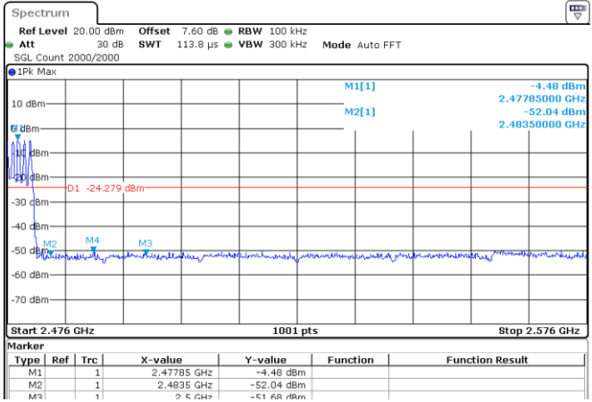
Hopping mode
