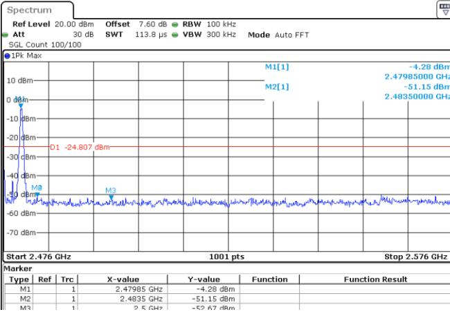
No-hopping mode
