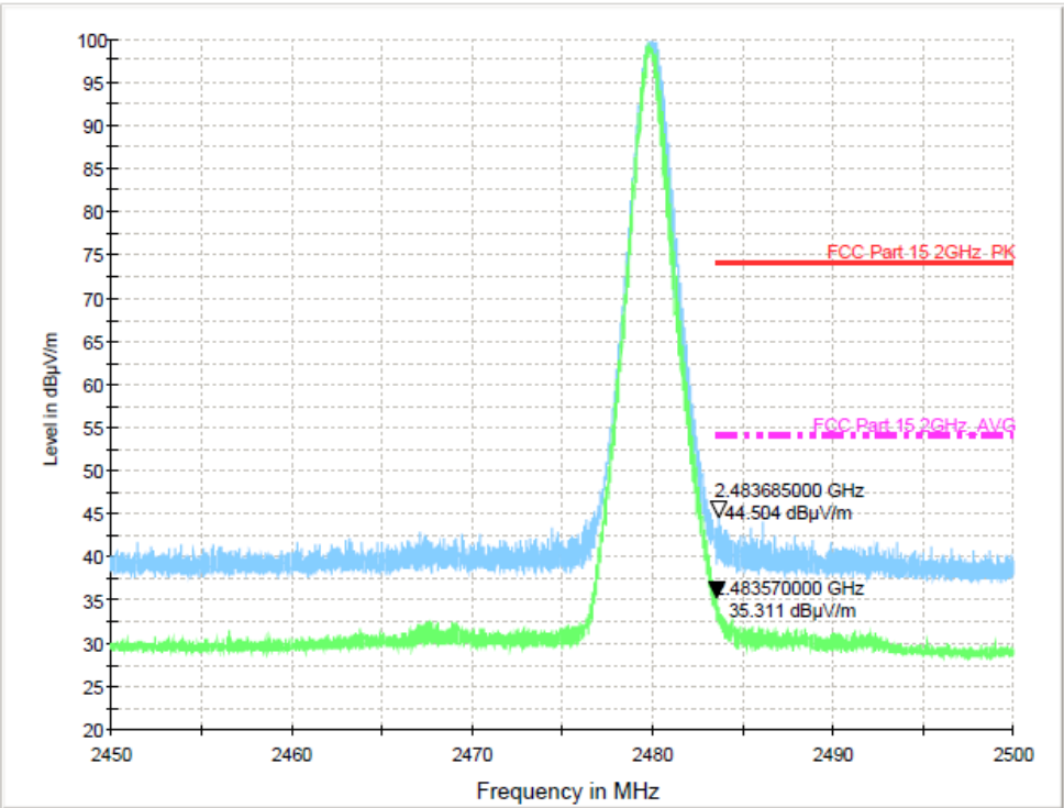
hopping-off
