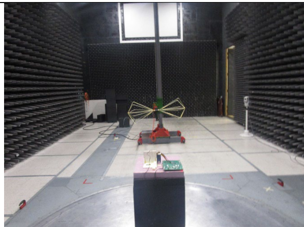
30-200 MHz Radiated
