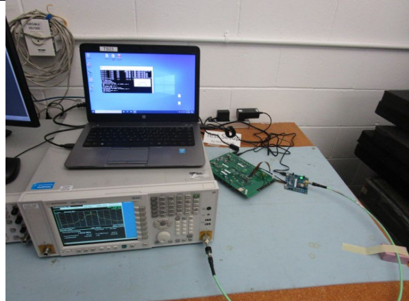
RF Conducted
