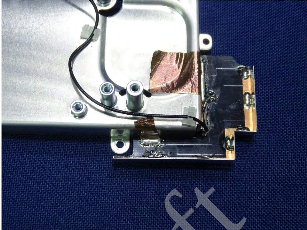
(29) EUT Photo – LTE Antenna
