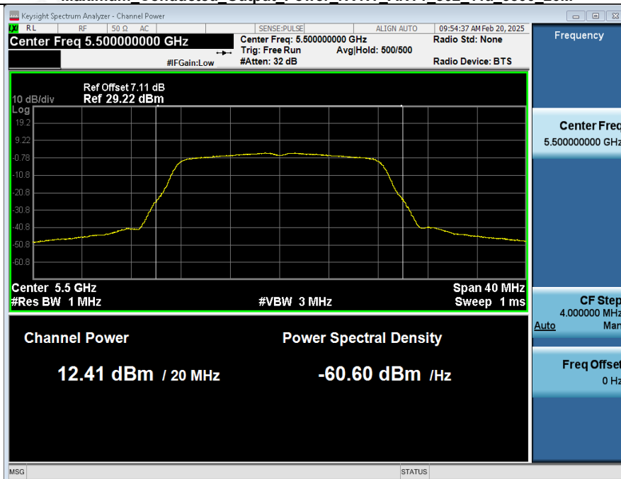
Maximum Conducted Output Power_NVNT_ANT2_802_11a_5500_20M
