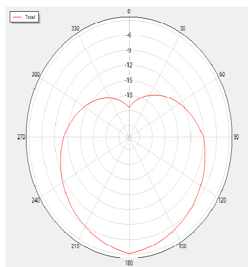
2450 Total
