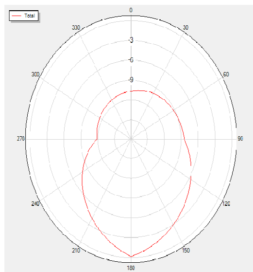
2500 Total
