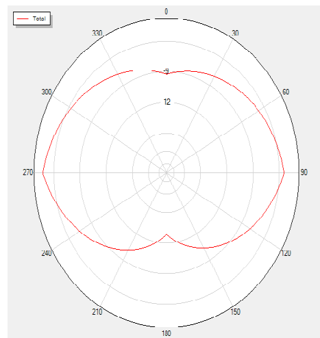
2425 Total
