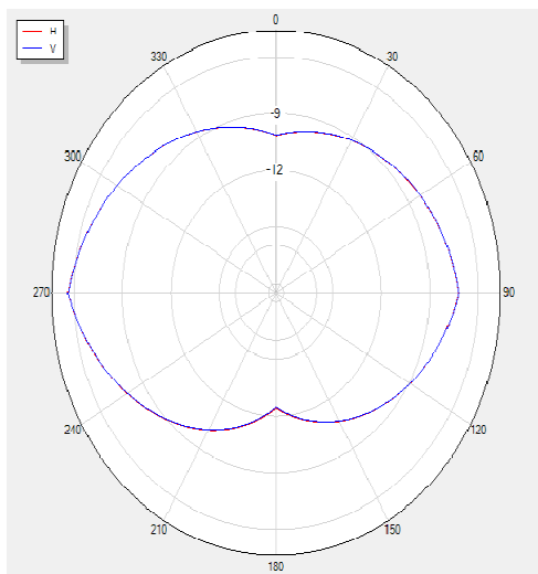
2475 Polar
