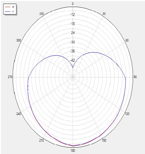
2400 Polar
