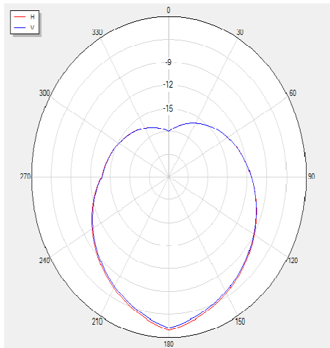
2475 Polar
