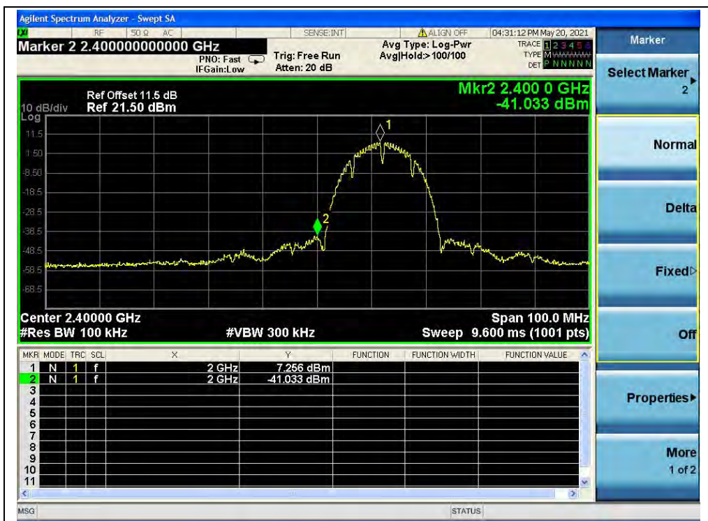
(Band Edge, Channel 1, 802.11b)
