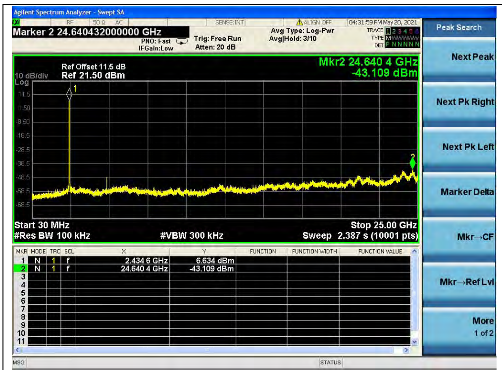
(30MHz to 25GHz, Channel 6, 802.11b)
