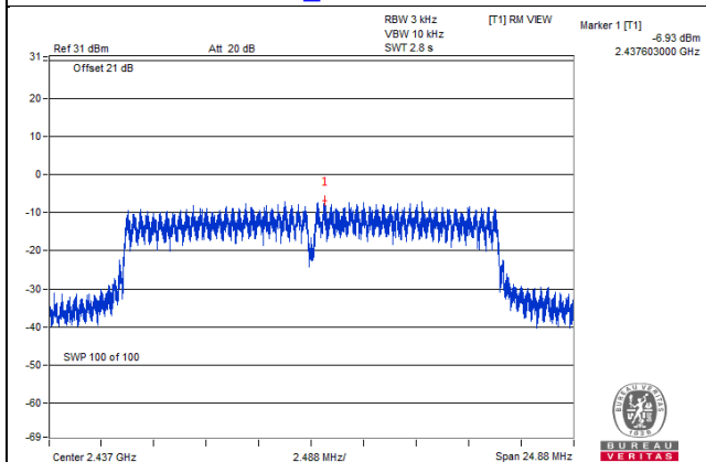
VHT20_Chain 0 / CH6
