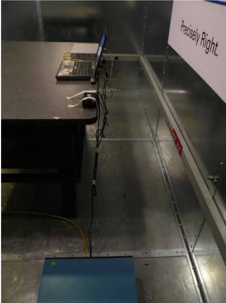
Figure 9: AC Conducted Emission Test Setup (Front)
