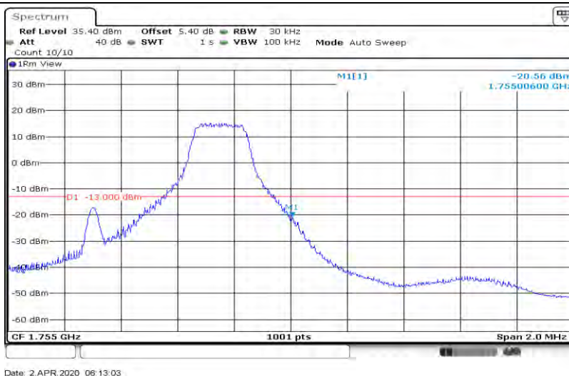
Band4-1.4MHz-16QAM-20393-6RB#0
