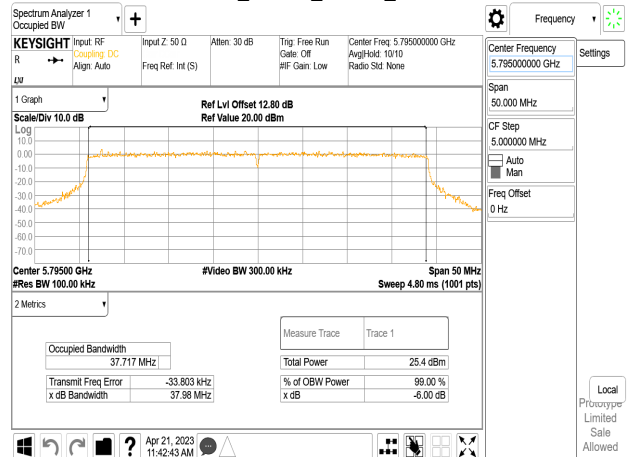
802.11ax_40MHz_Chain0_5795MHz
