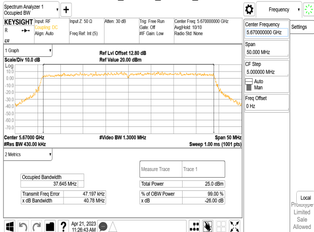
802.11ax_40MHz_Chain0_5670MHz
